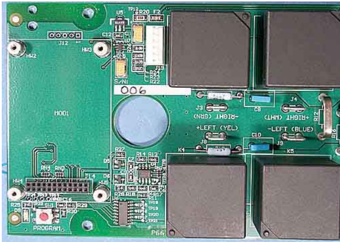
Receiver Board Left Side Close-up View
