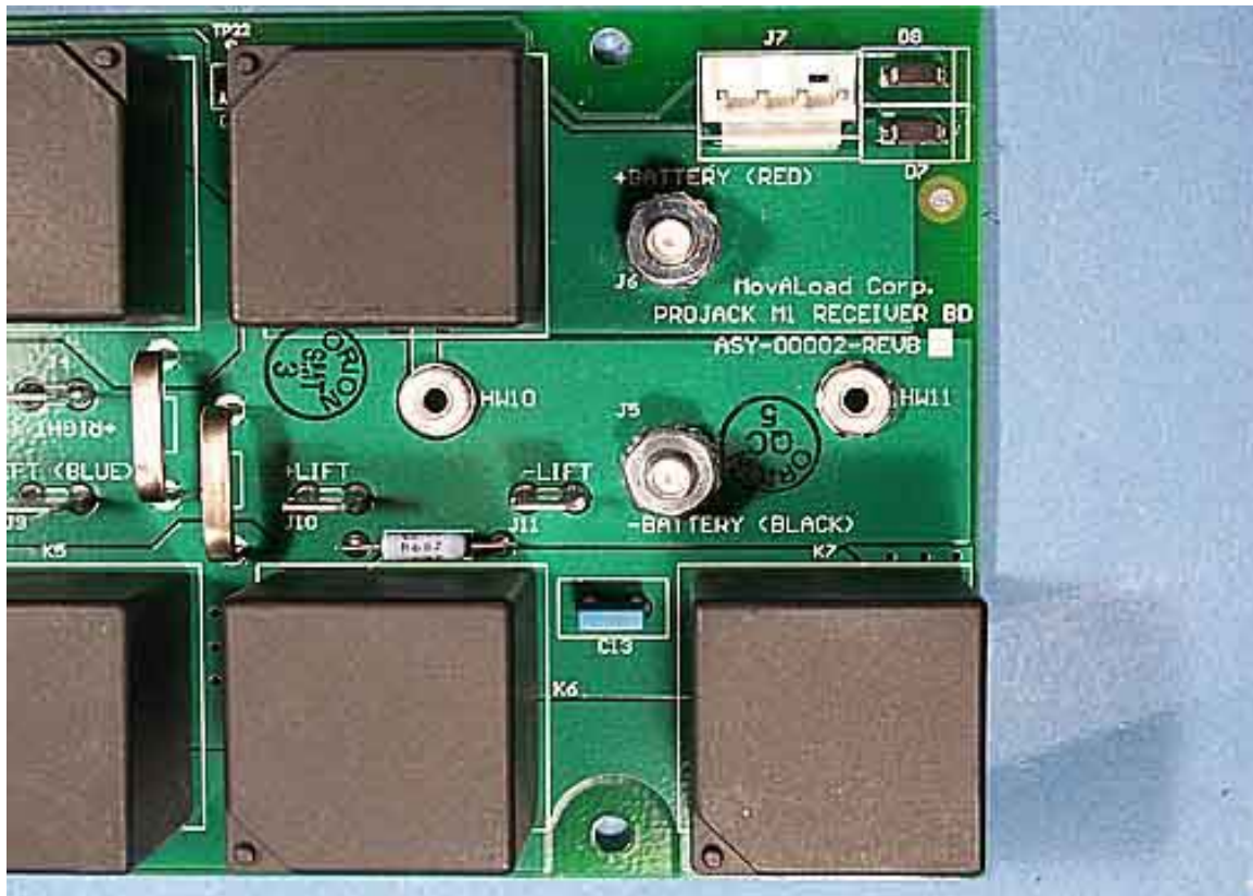
Receiver Board Right Side Close-up of Top
