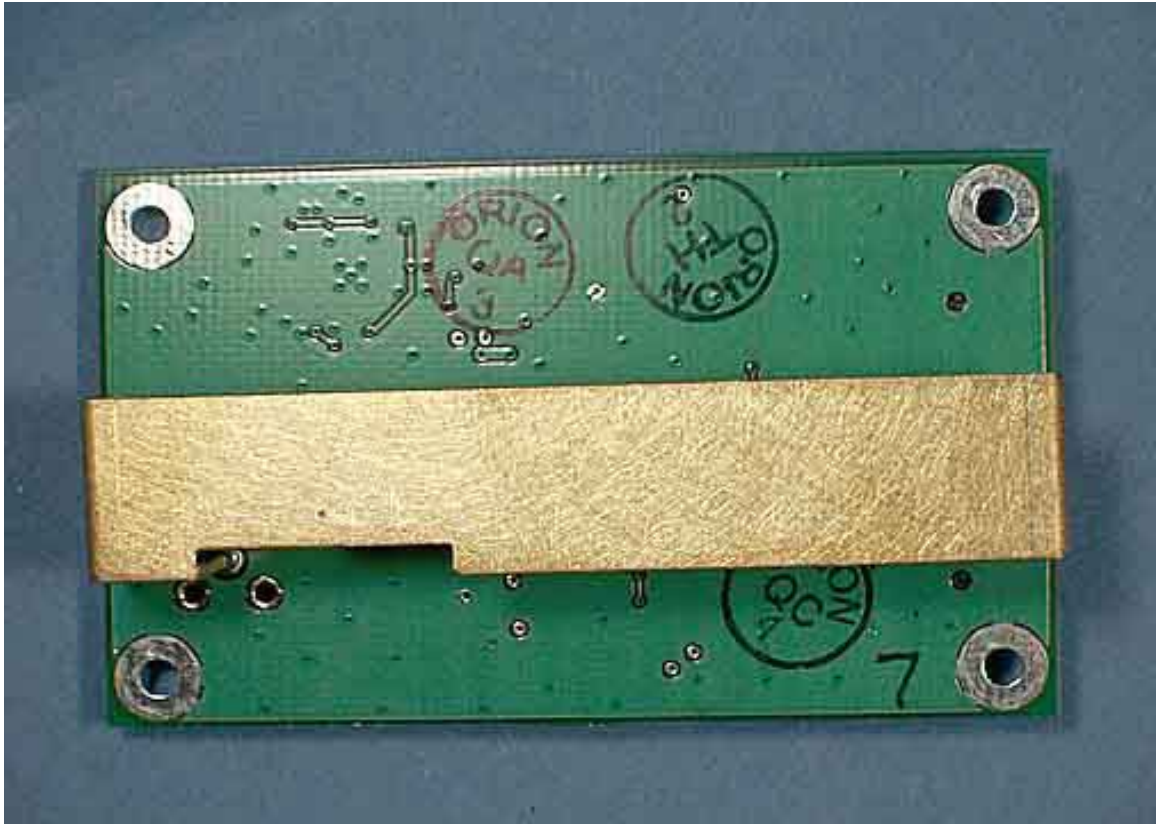
Falcon-900 RF Modem Board Top View
