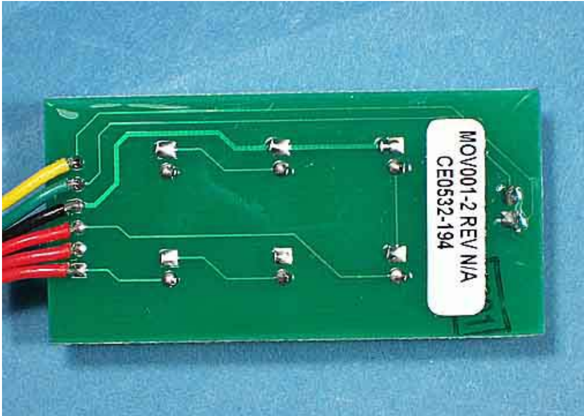
MOV001-2A PCB Board Bottom View
