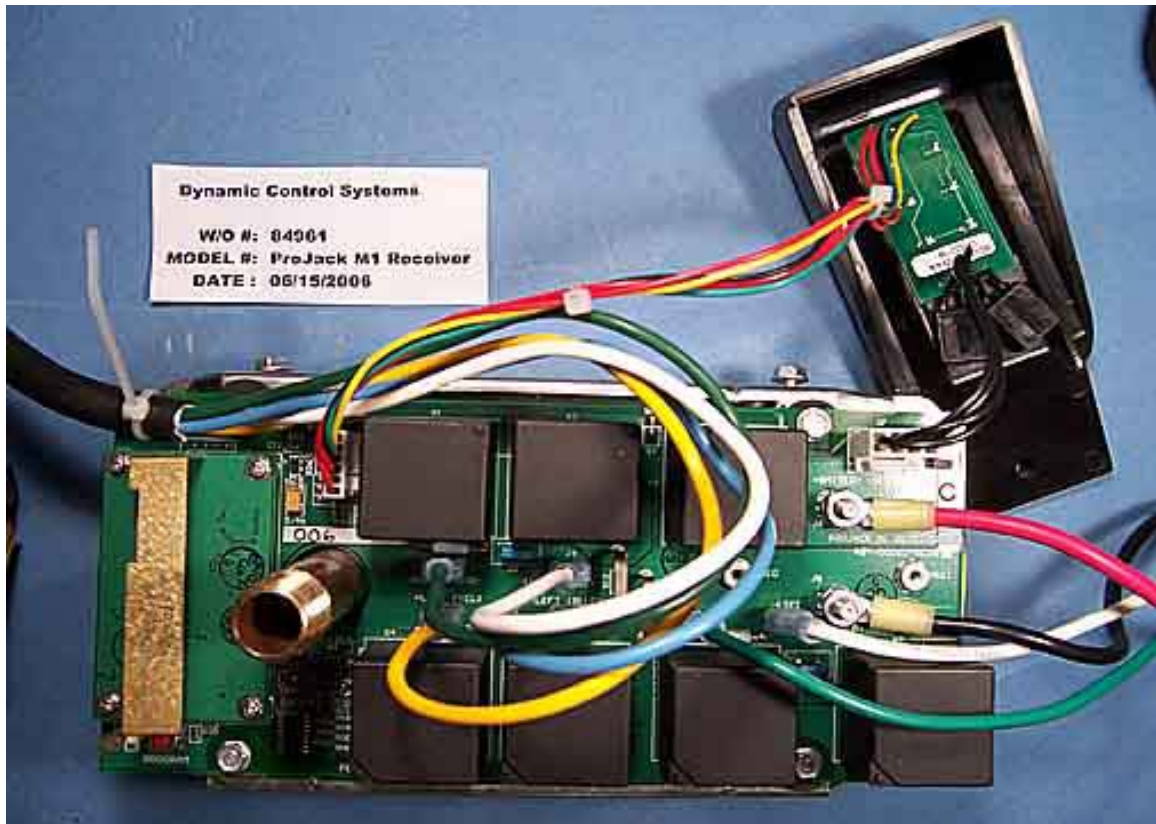
Receiver Full System
