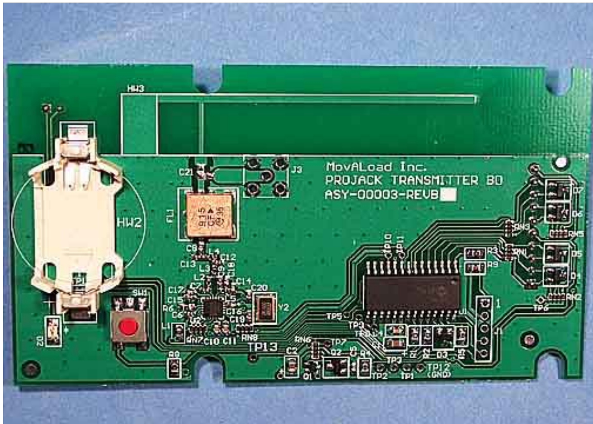
Transmitter Board Top
