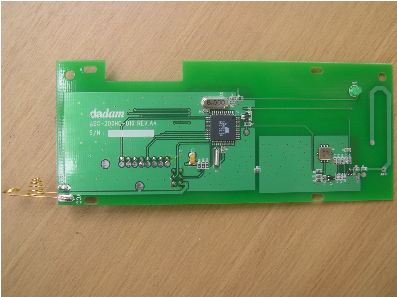
<Photograph 2: Front View – Main board>
