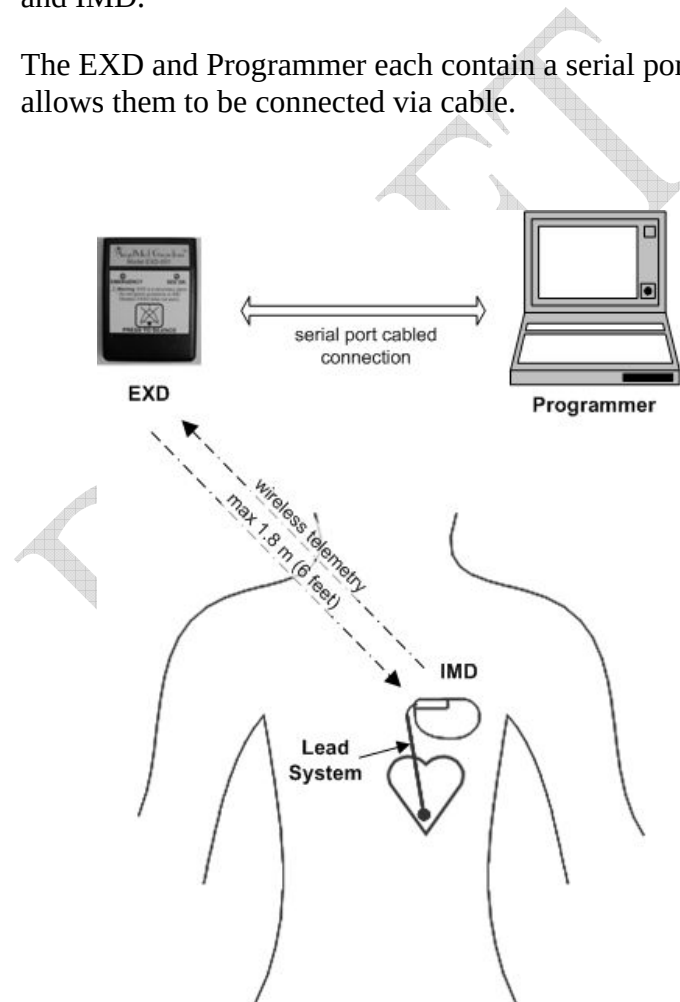
Fig. 1: Guardian System Communication Architecture
