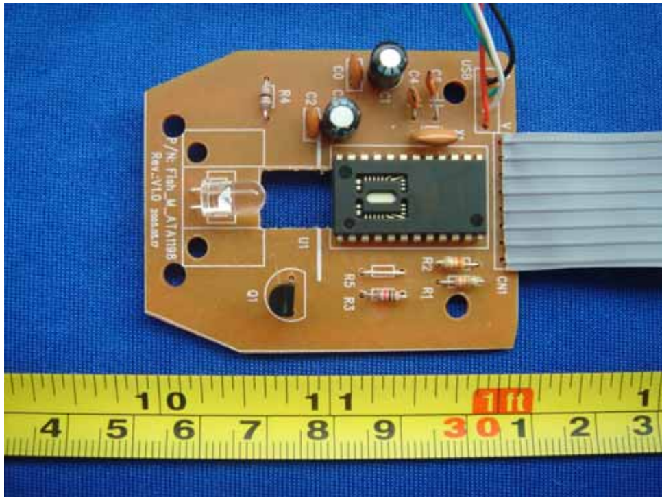
PCB(1) - Component View
