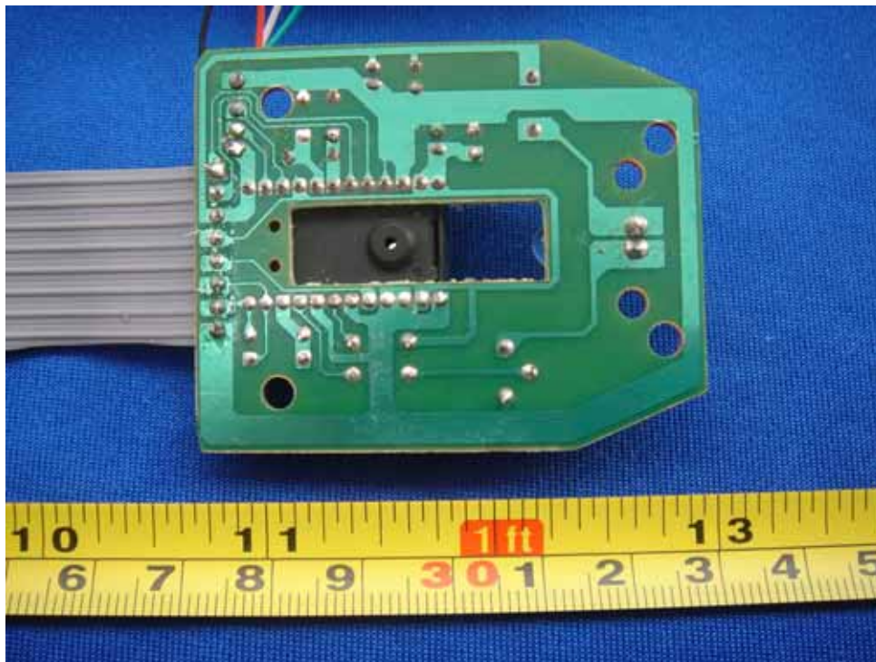
PCB(1) - Solder View
