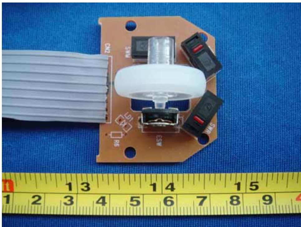
PCB(2) - Component View
