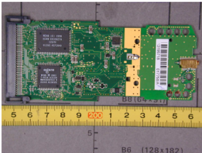
Top view of printed board of RF-modem (disassembled version)
