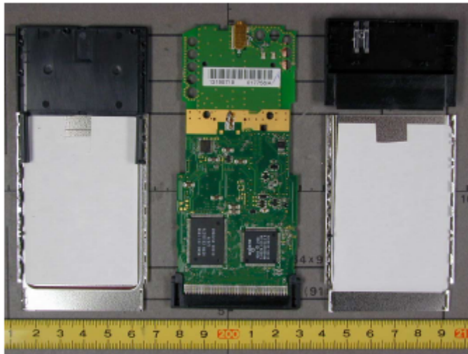
Top view of disassembled RF-modem (disassembled version)
