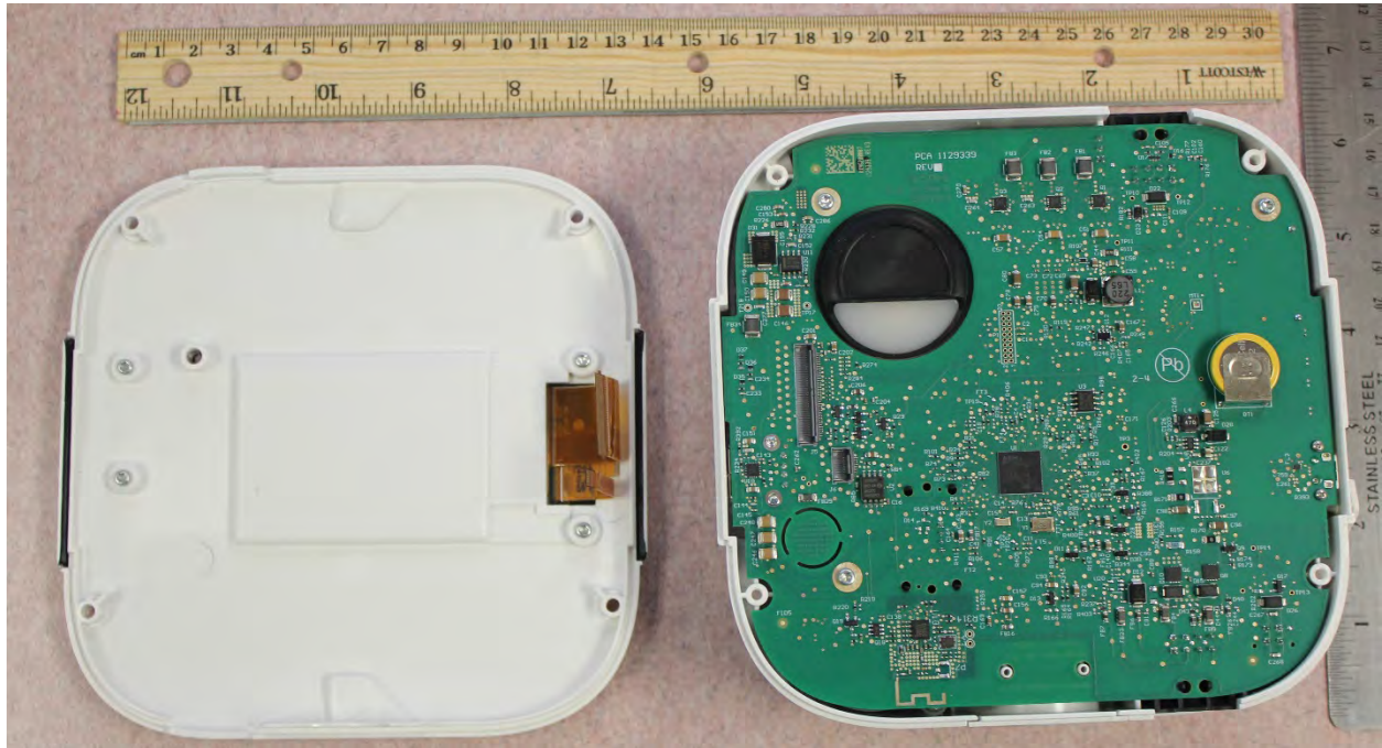
Figure 1: Internal Top View of DreamStation Go Device
