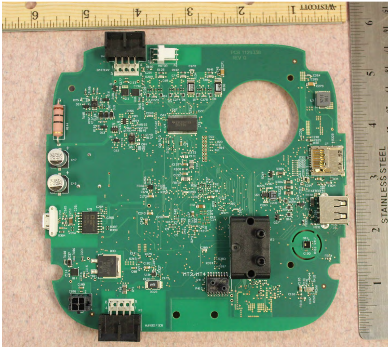
Figure 3: Internal Bottom View of DreamStation Go PCA
