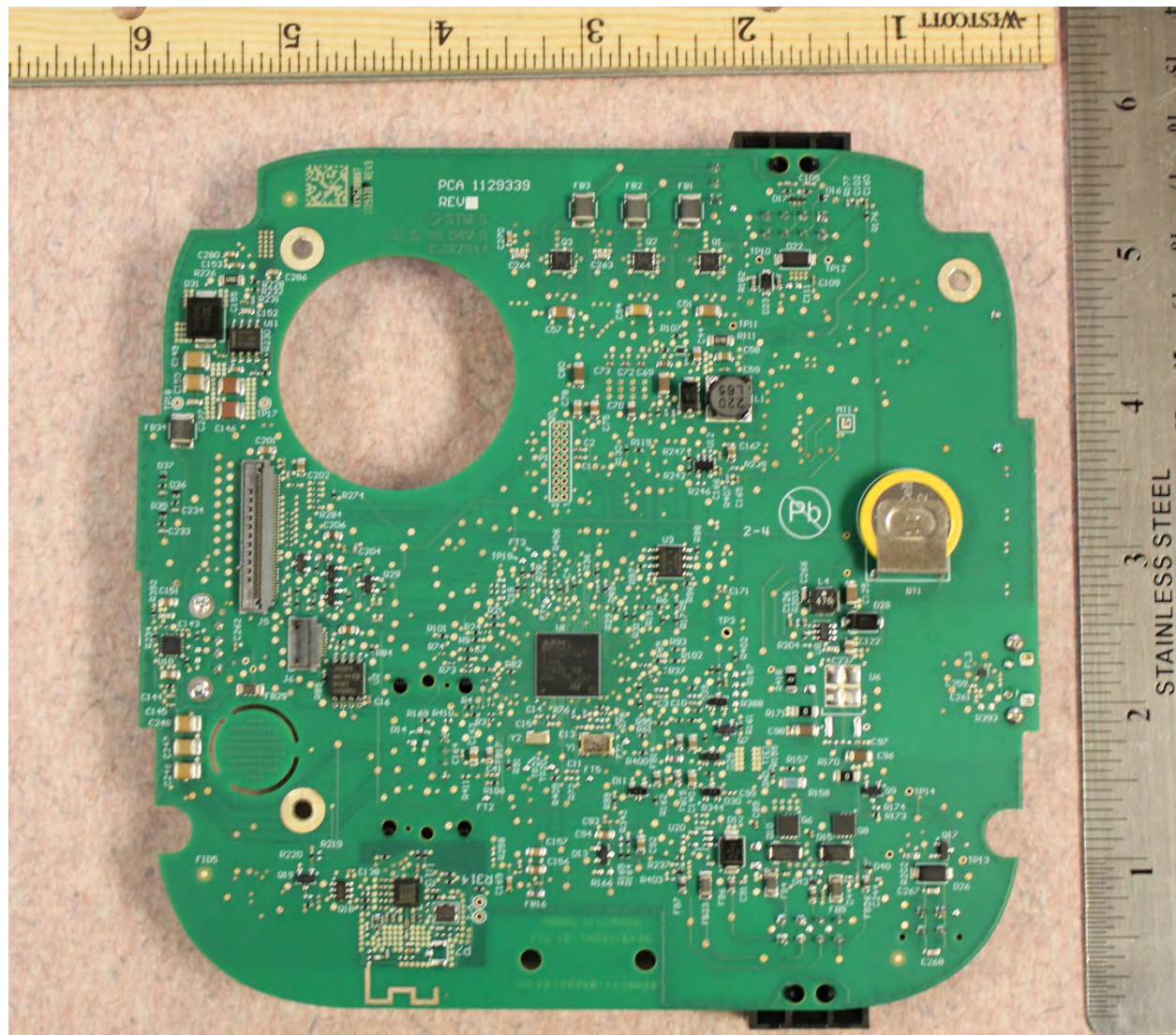
Figure 2: Internal Top View of DreamStation Go PCA
