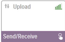
Upload Screen
