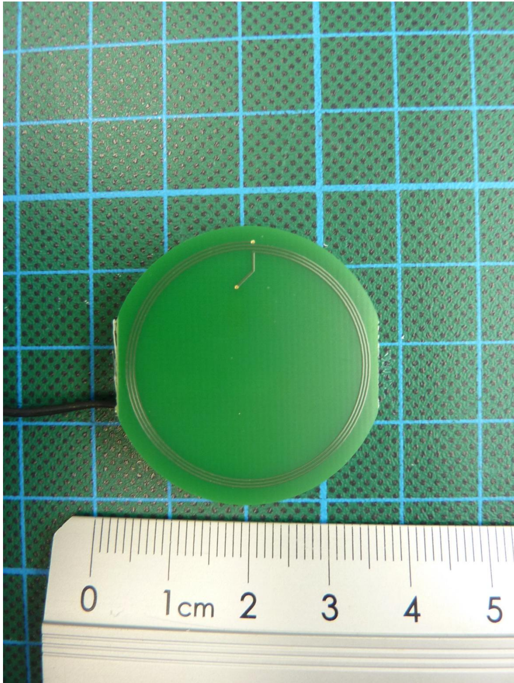
160874_18.jpg: EasyScan Module, antenna 2, bottom view
