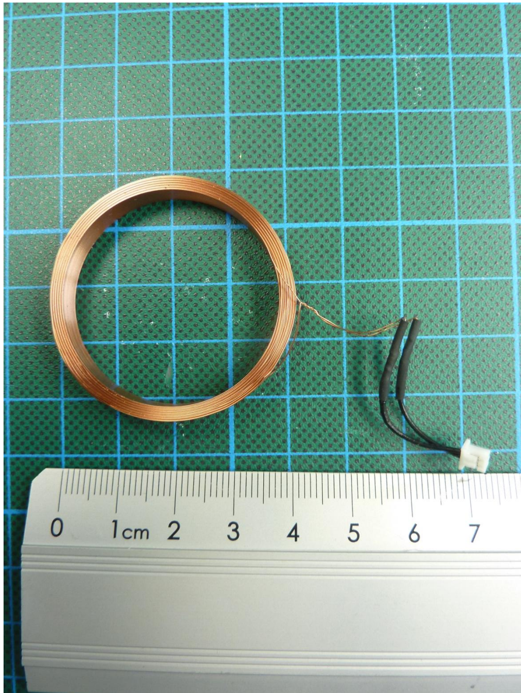
160874_19.jpg: EasyScan Module, antenna 1
