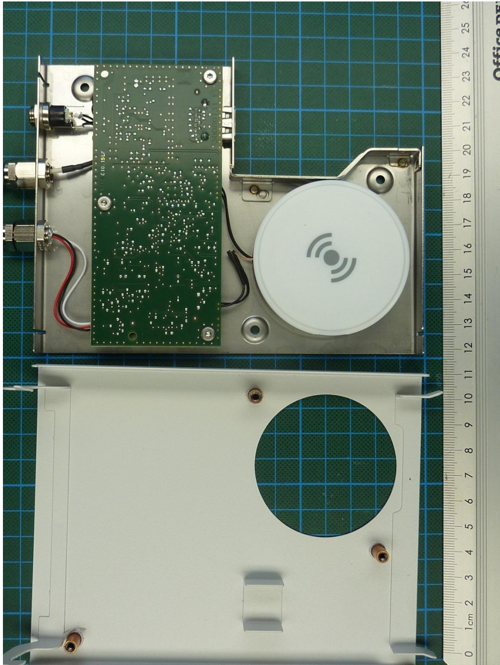
160874_13.jpg: EasyScan Module, internal view 1
