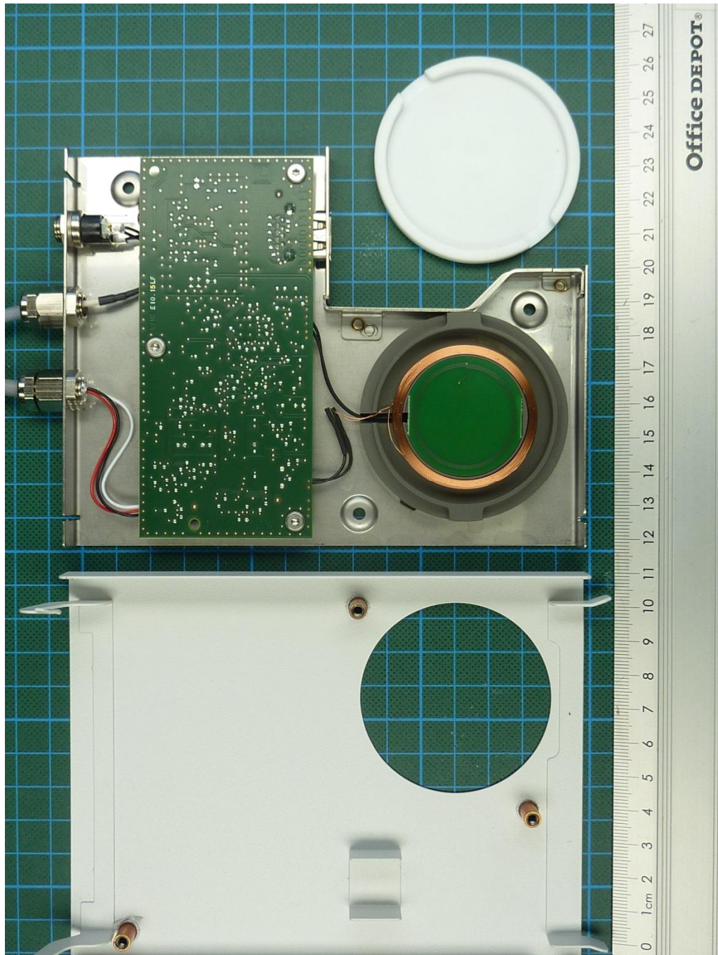
160874_14.jpg: EasyScan Module, internal view 2
