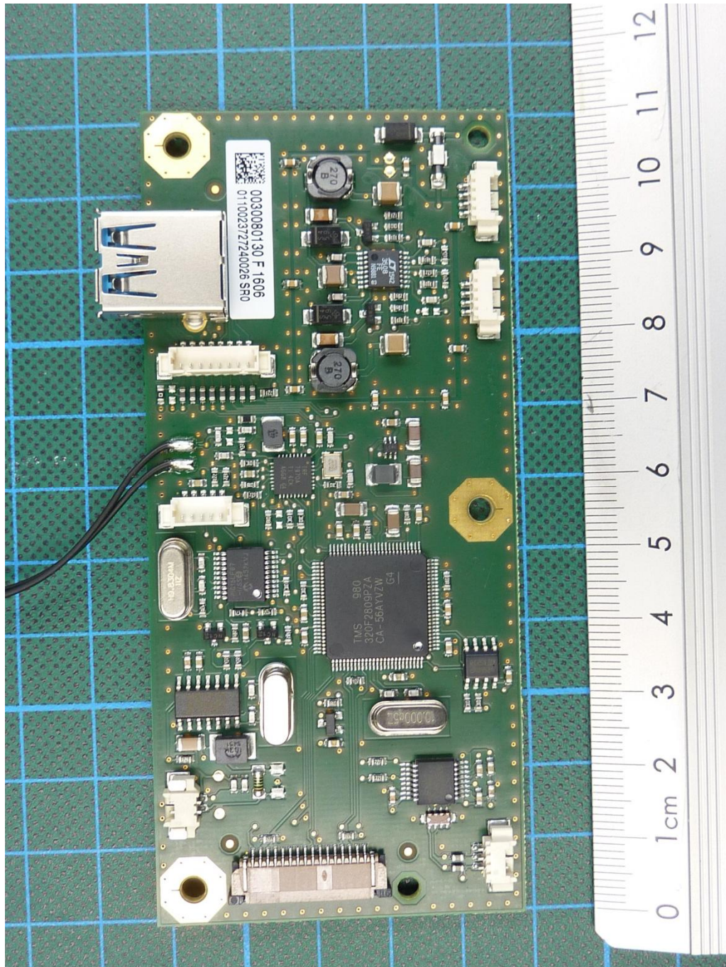
160874_15.jpg: EasyScan Module, PCB, top view
