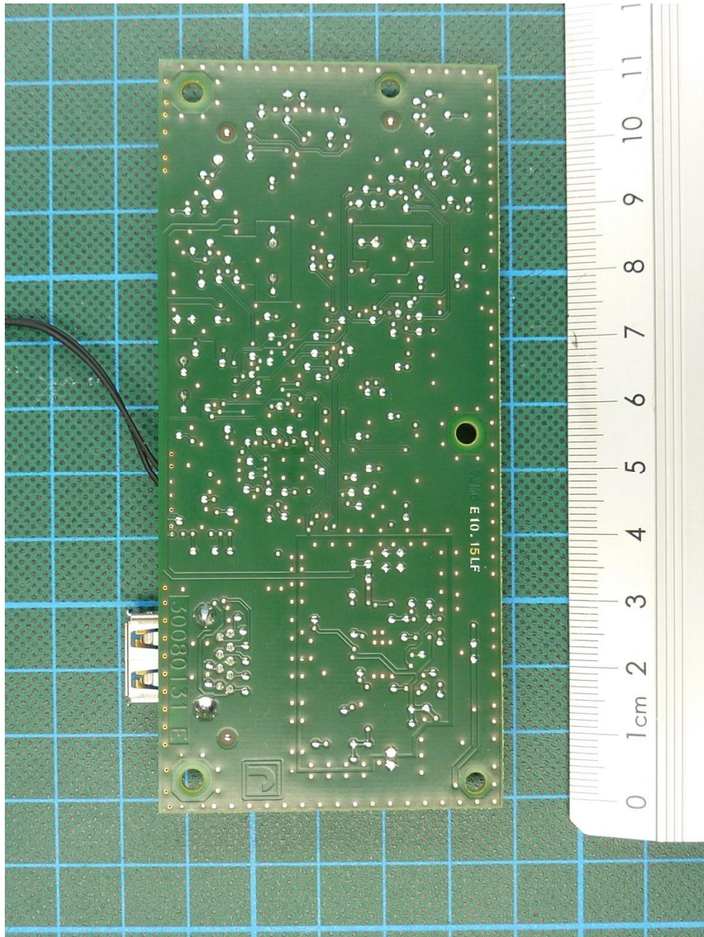
160874_16.jpg: EasyScan Module, PCB, bottom view
