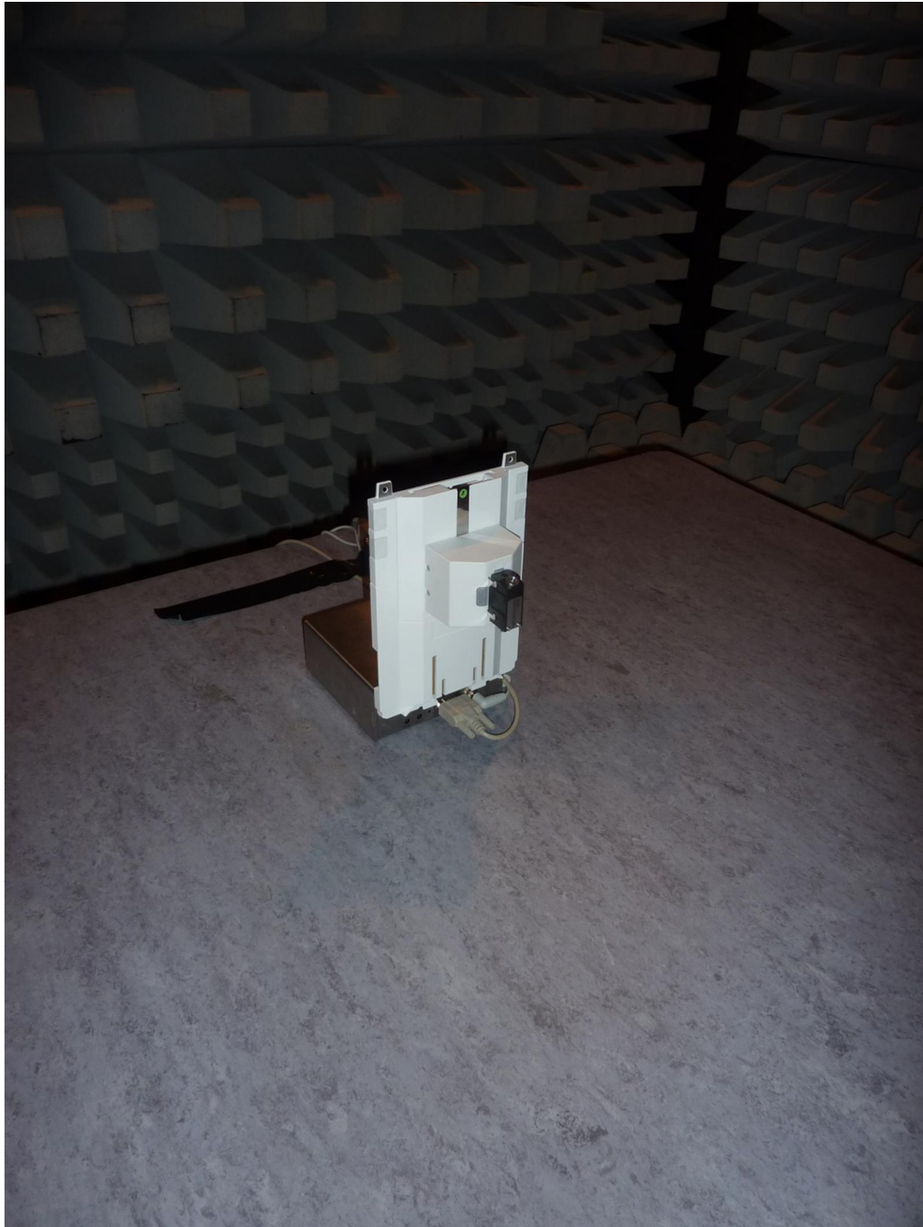
181223_c.jpg: QLX3 liquid module, test setup fully anechoic chamber
