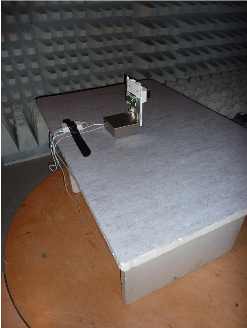
181223_a.jpg: QLX3 liquid module, test setup fully anechoic chamber
