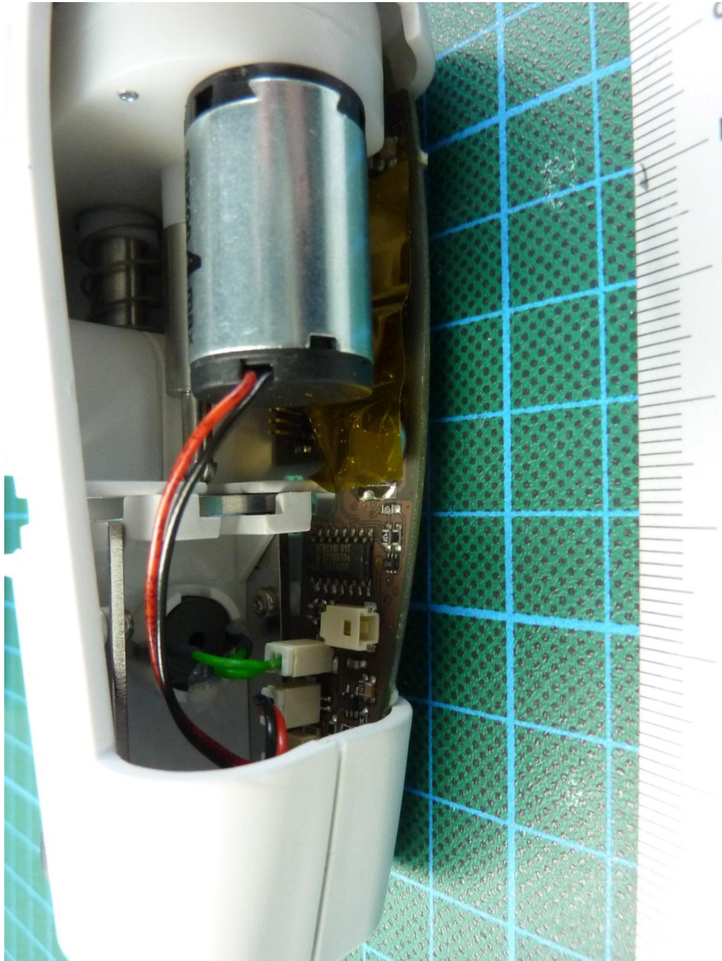
161007_11.jpg: Quantos HPD, internal view 2
