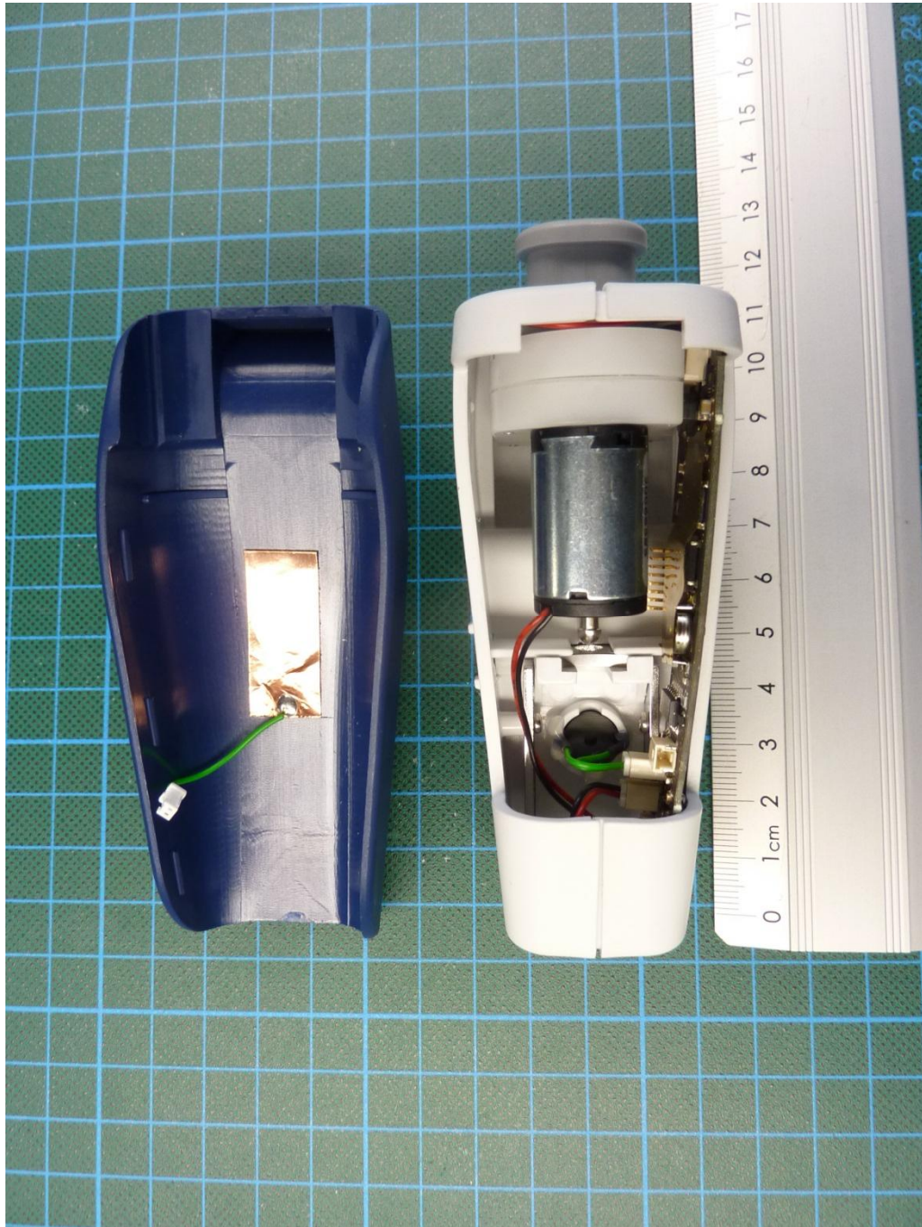
161007_10.jpg: Quantos HPD, internal view 1
