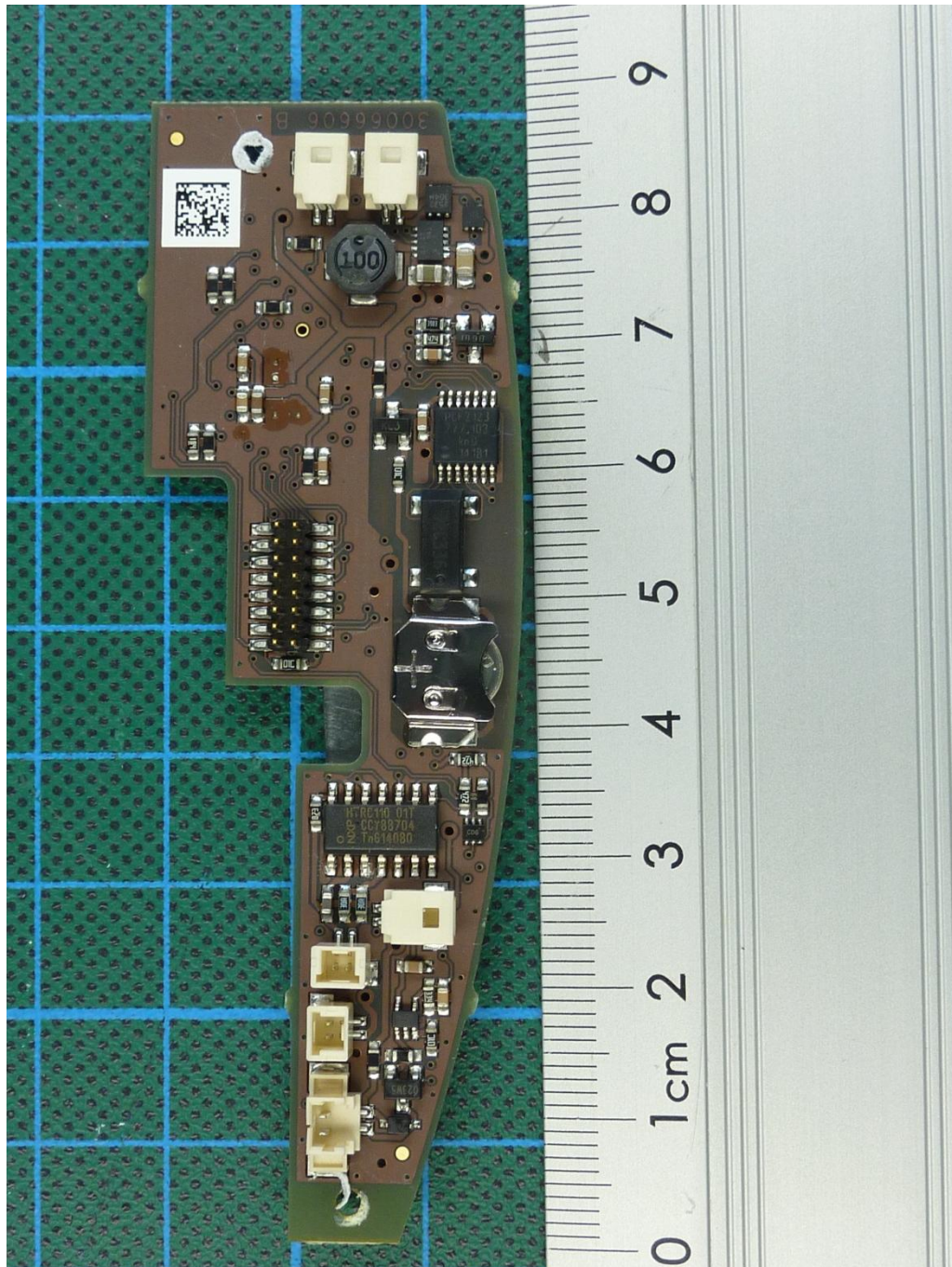
161007_16.jpg: Quantos HPD, PCB, top view
