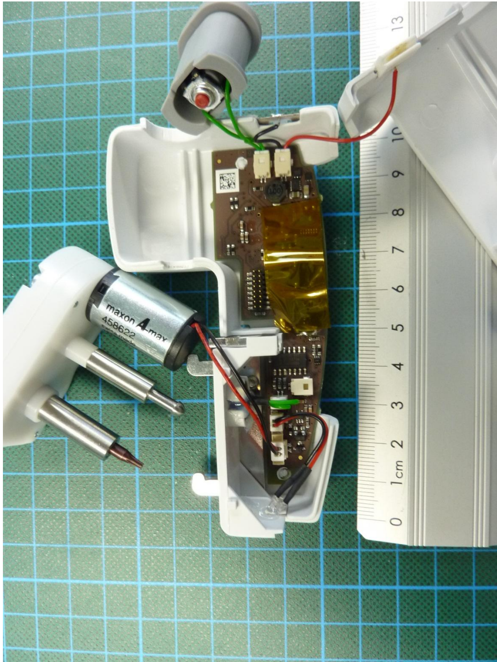
161007_14.jpg: Quantos HPD, internal view 3
