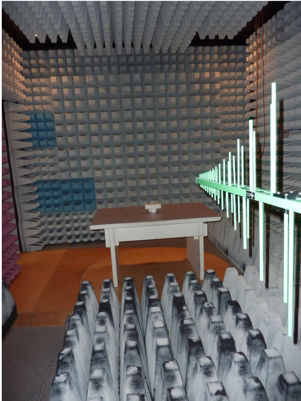
161007_1e.jpg: Quantos HPD, test setup fully anechoic chamber
