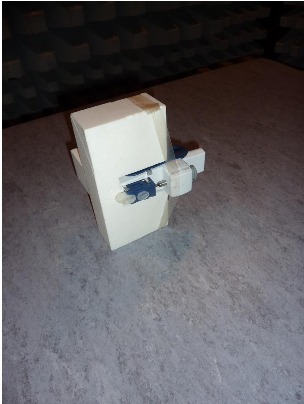
161007_1c.jpg: Quantos HPD, test setup fully anechoic chamber, Position 3
