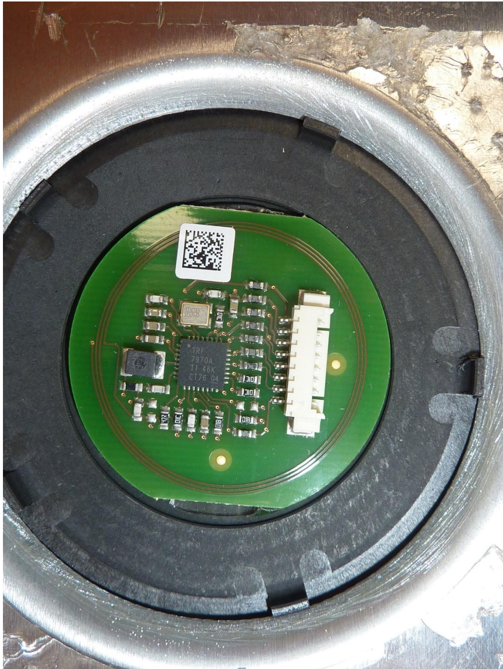
161000_10.jpg: SmartSample, internal view 2
