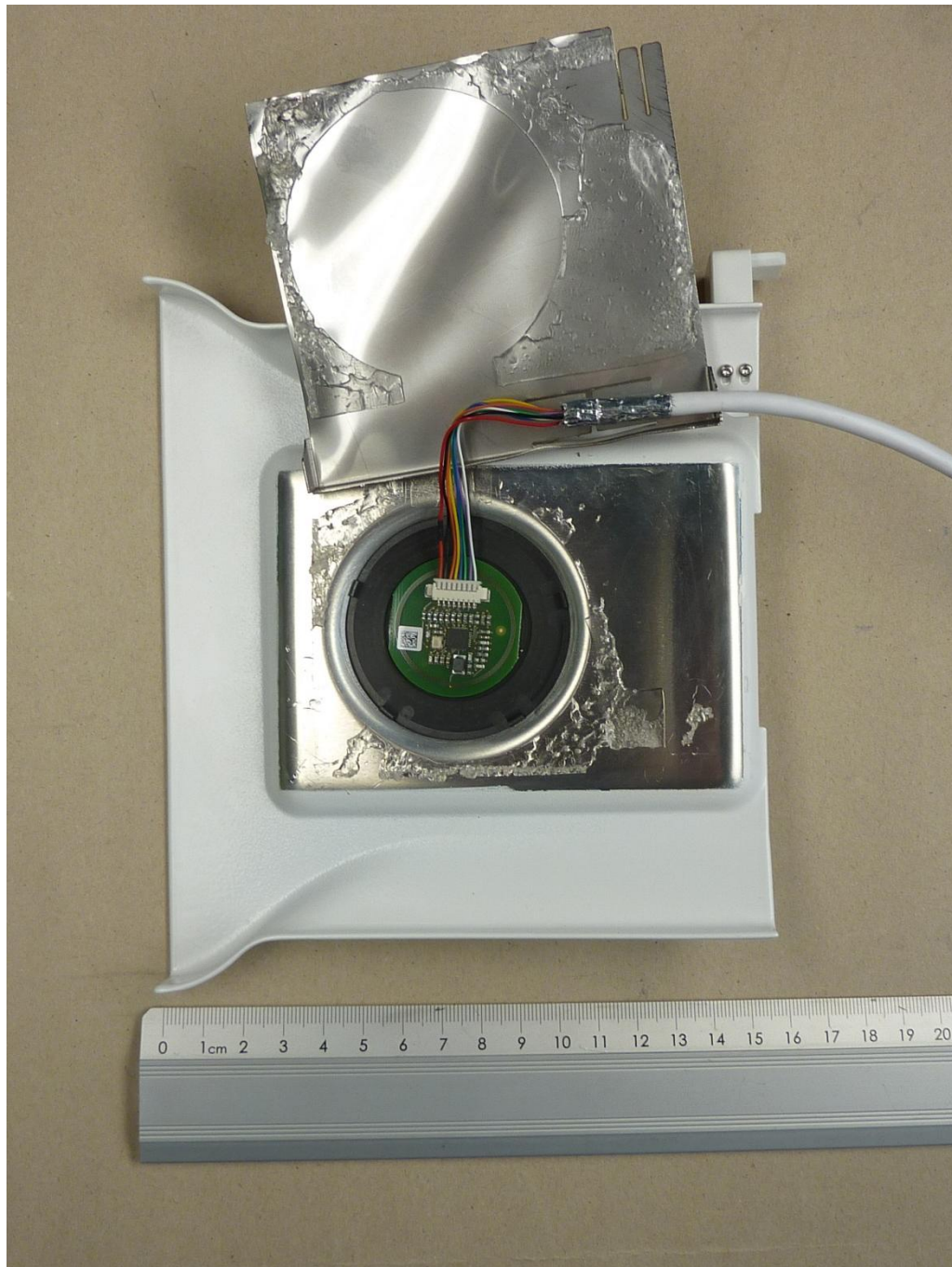
161000_9.jpg: SmartSample, internal view 1
