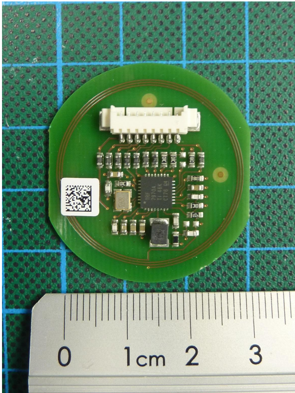
161000_11.jpg: SmartSample, PCB, top view
