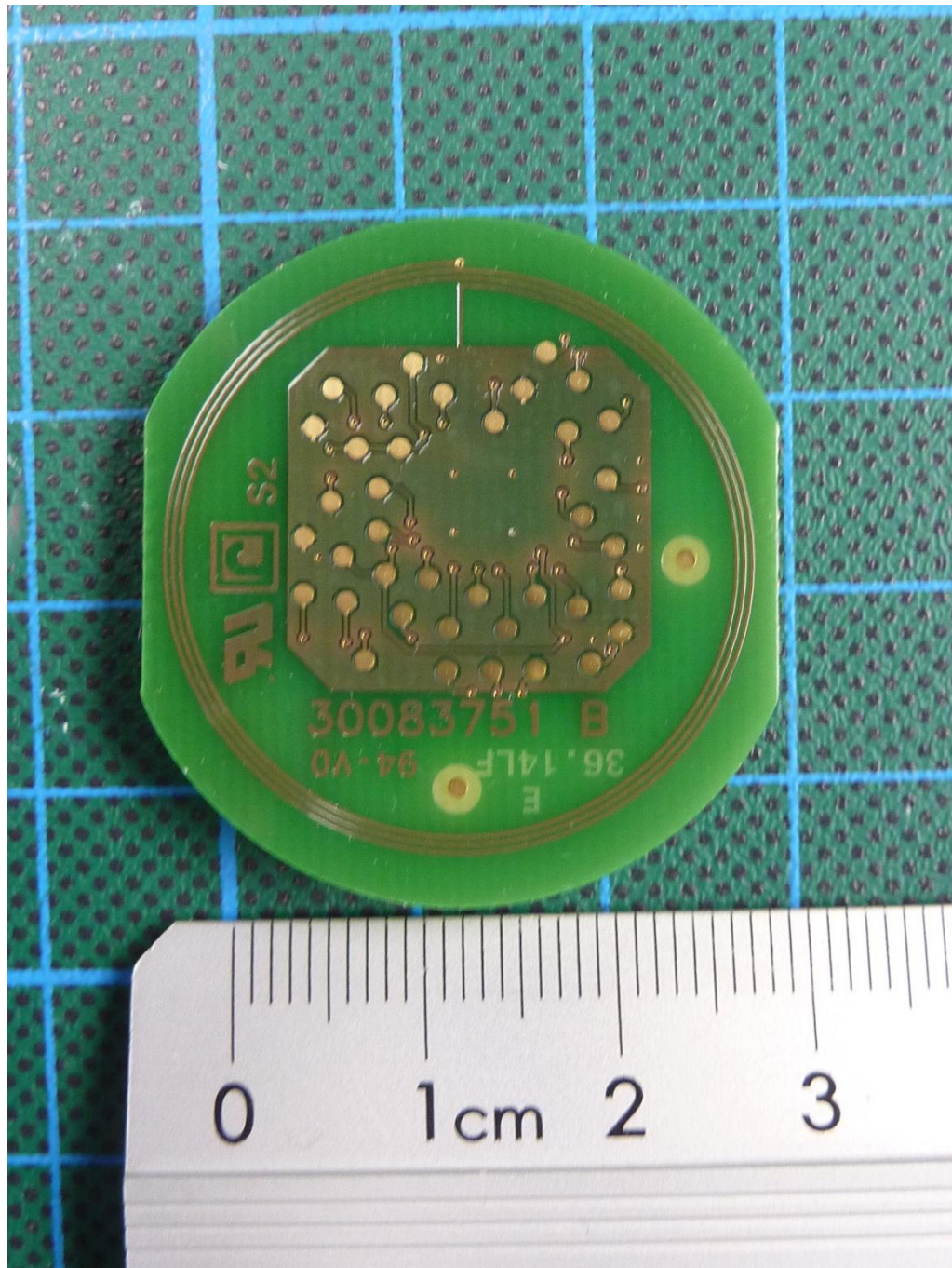
161000_12.jpg: SmartSample, PCB, bottom view
