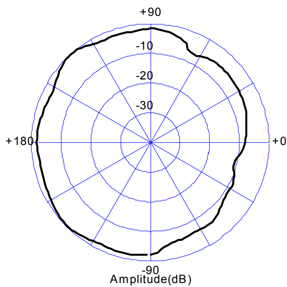
Horizontal Pattern
