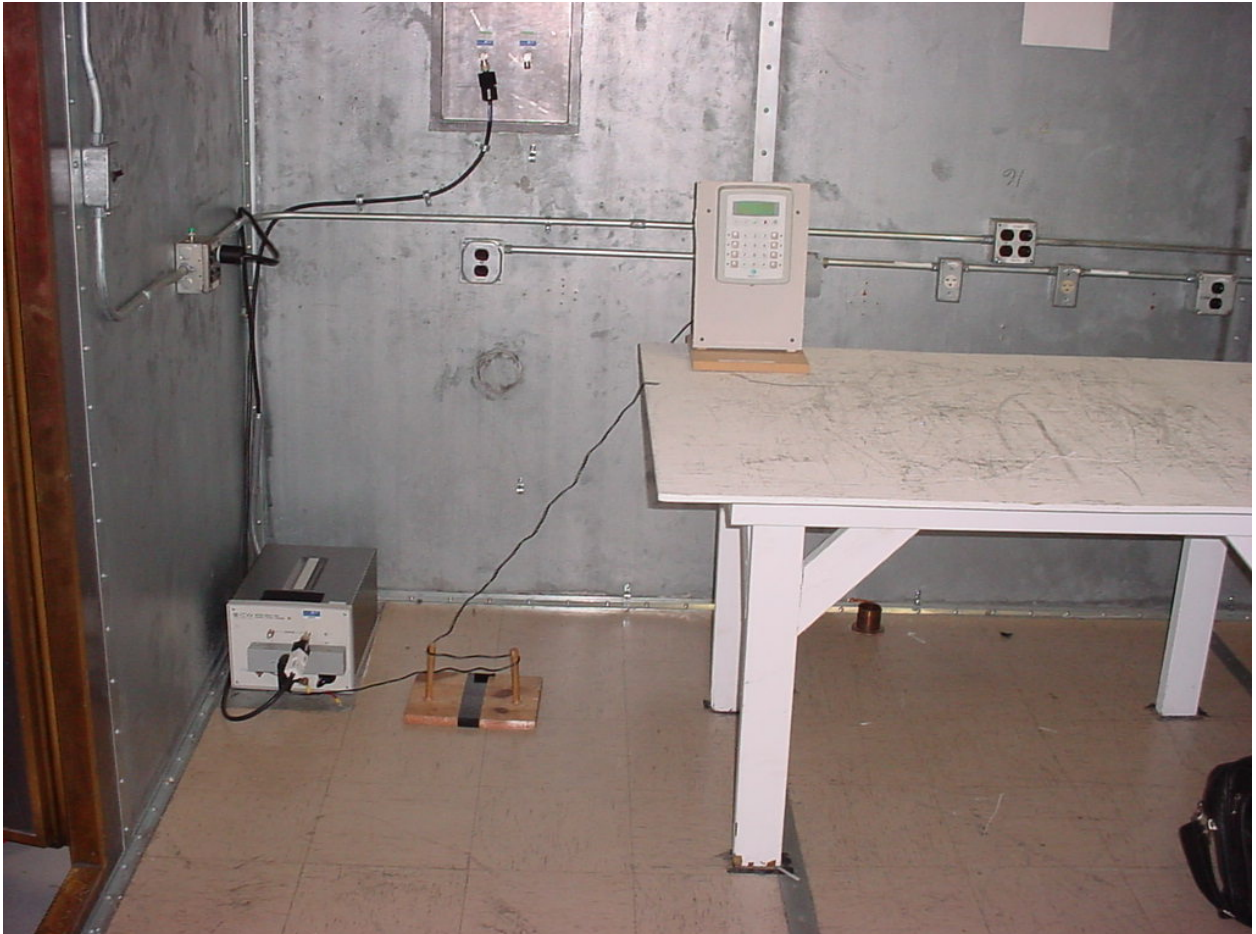
Figure 2: Test Setup – Conducted Emissions – FRIWO PS
