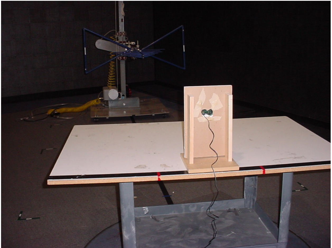
Figure 4: Test Setup – Radiated Emissions
