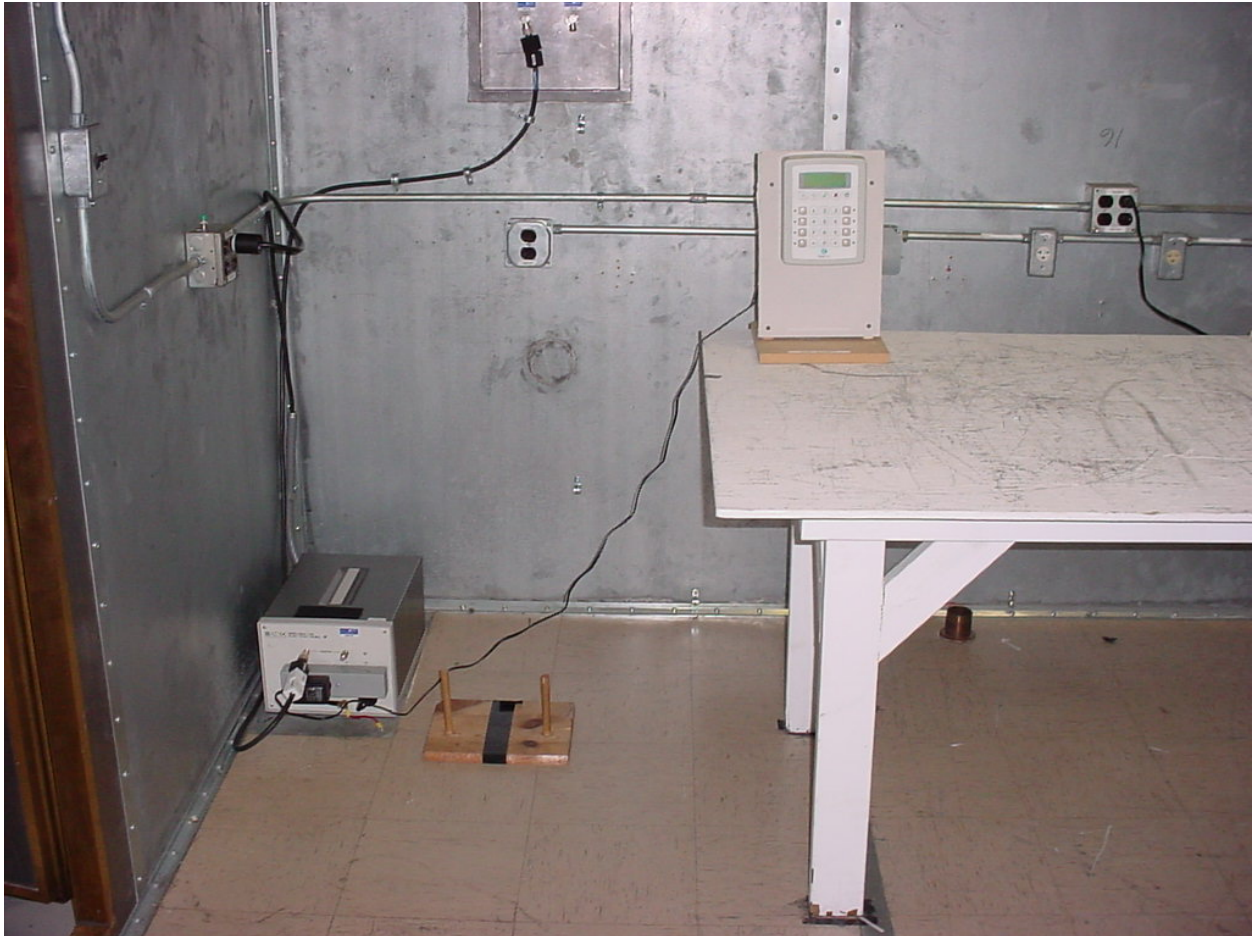
Figure 1: Test Setup – Conducted Emissions – GlobTek PS
