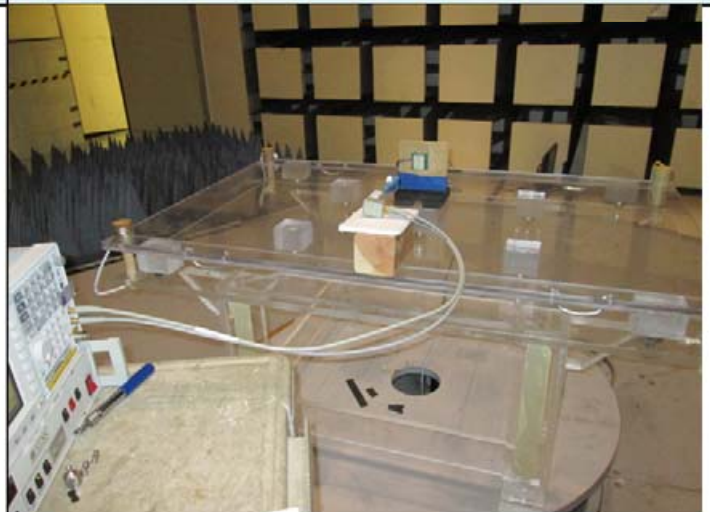
Setup for 18 to 26.5 GHz, Front
