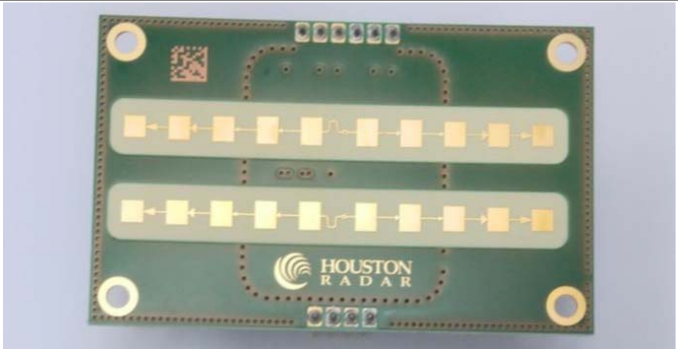
RF Module, Antenna Side
