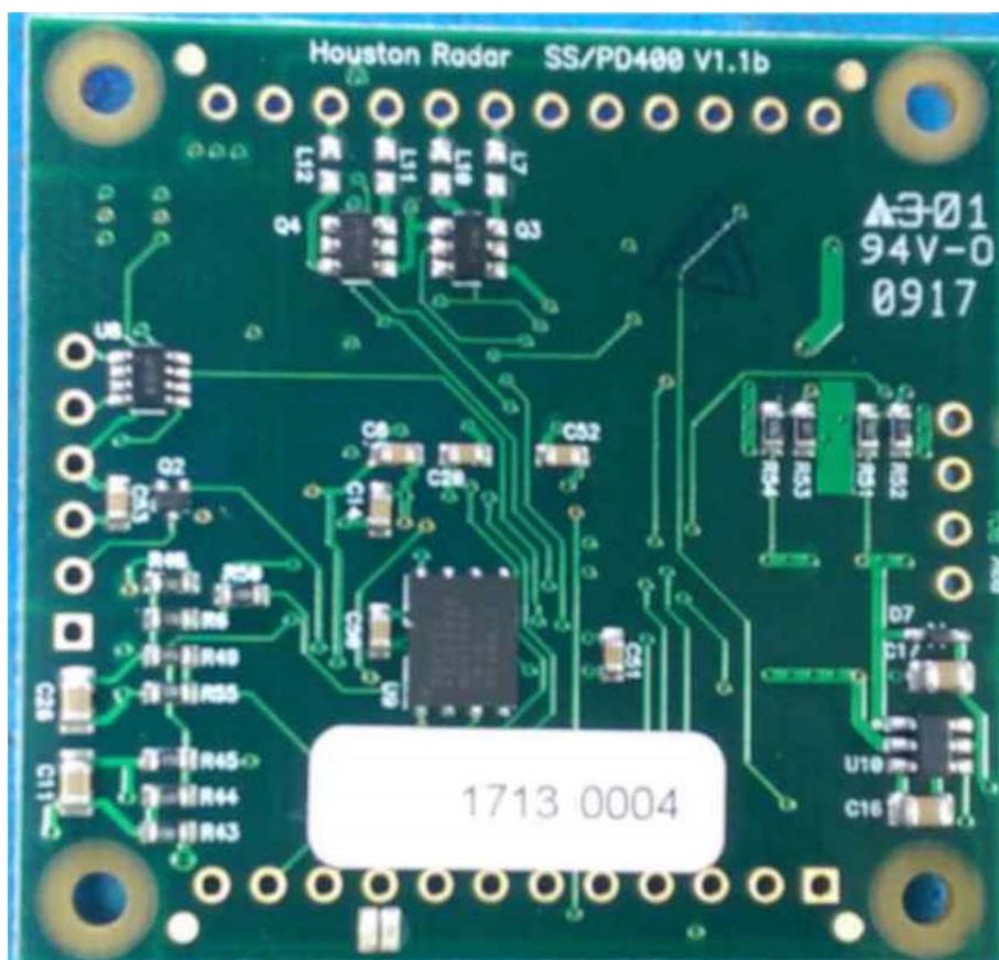
Interface Board, Side 2
