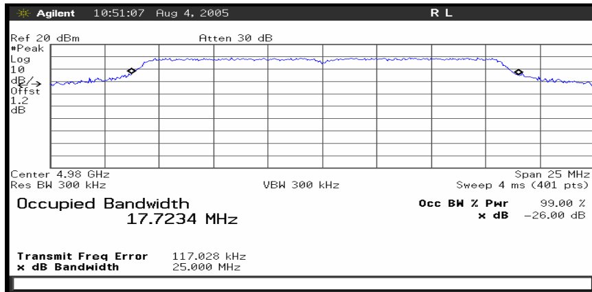
Plot 17. Measured Occupied Bandwidth
