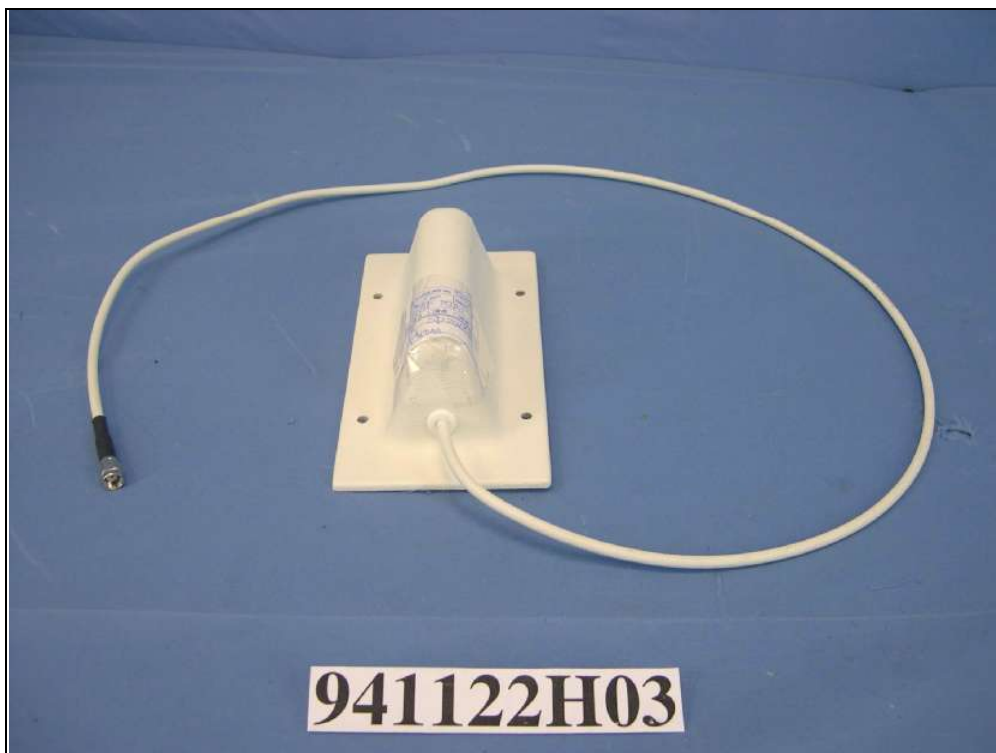
Antenna Model No.: S24497P
