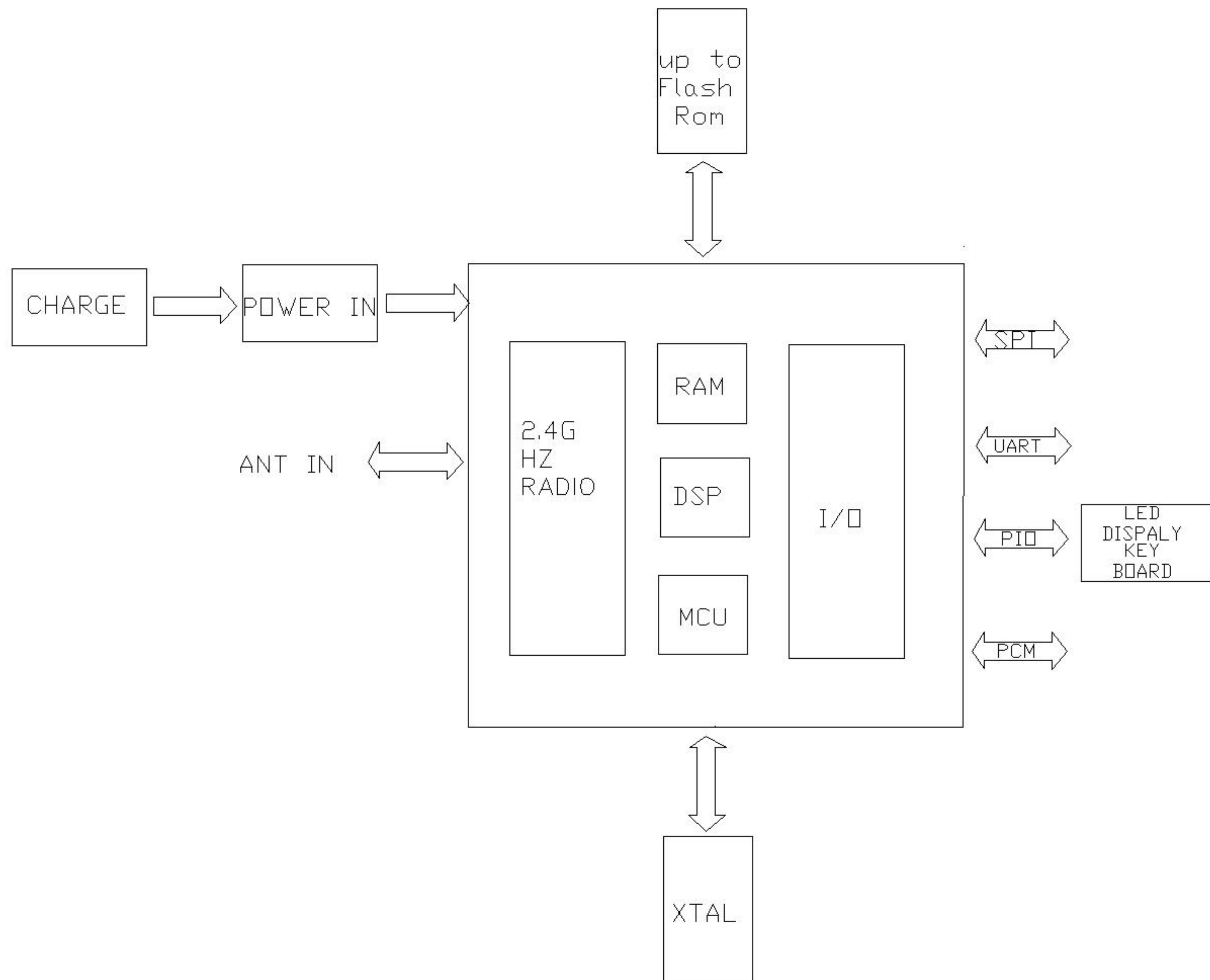
KISS-12 Block Diagram
