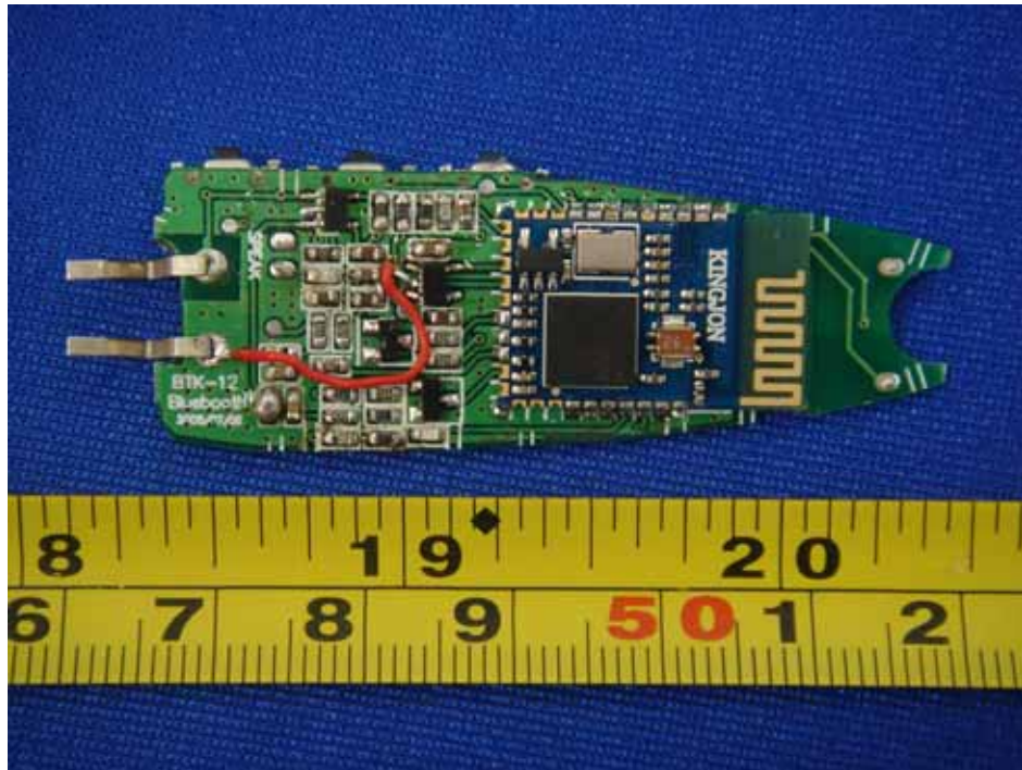
PCB - Component View (1)
