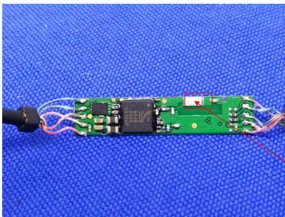
BT Antenna
