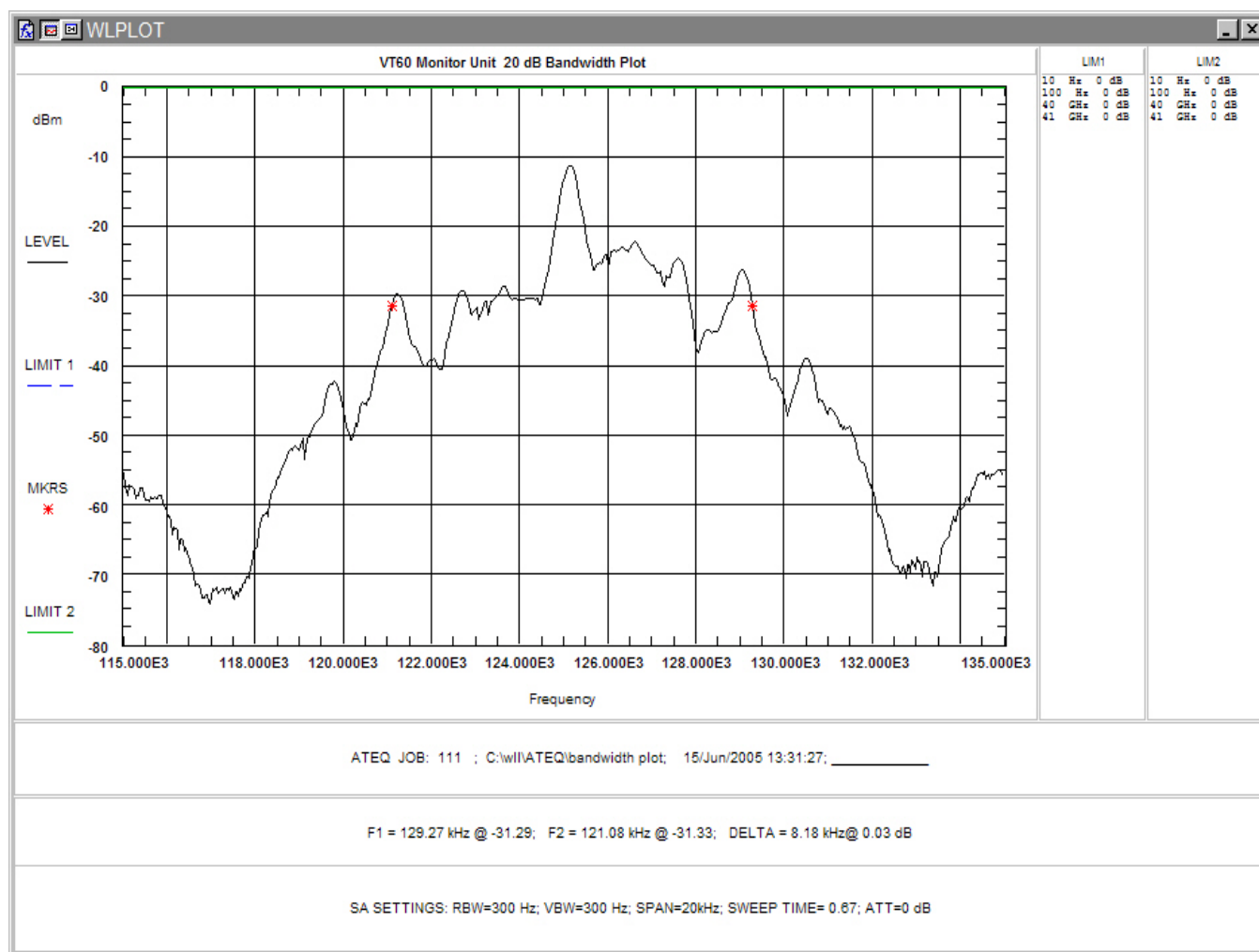
Figure 1. Occupied Bandwidth
