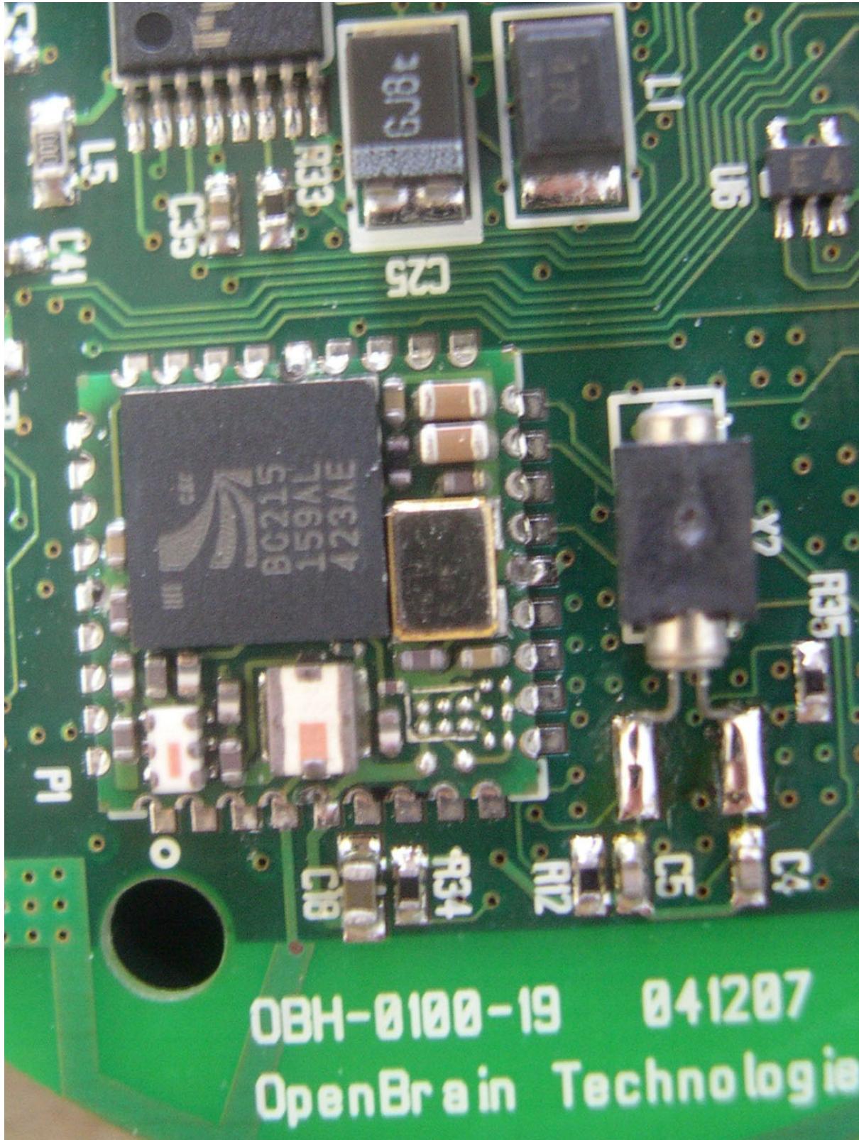
<Photograph 4: RF Shielding CAN removed>
