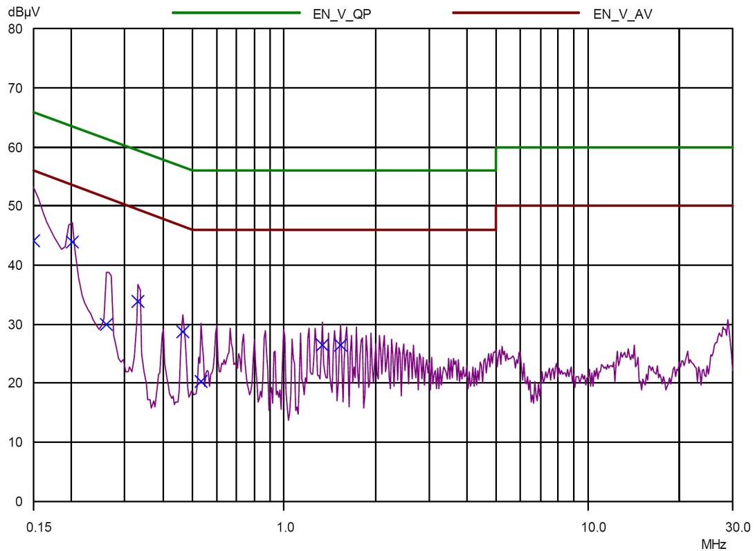
Figure 11. Plot of the Conducted Emissions (INDIRECTLY)
