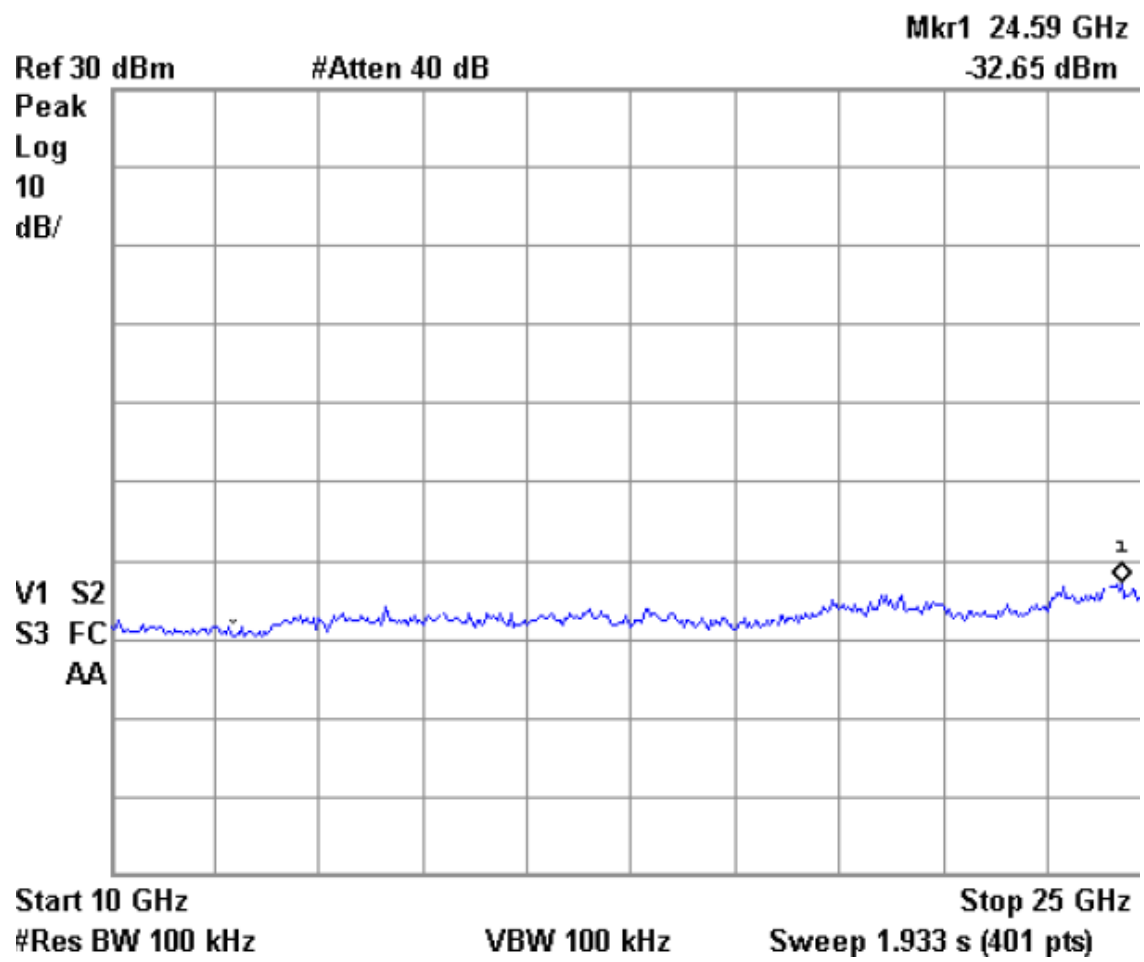
Out of Band Conducted Spurious Emission of Top Channel
