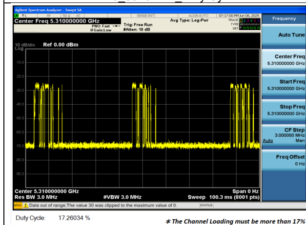
EHT40_5310MHz_Duty Cycle
