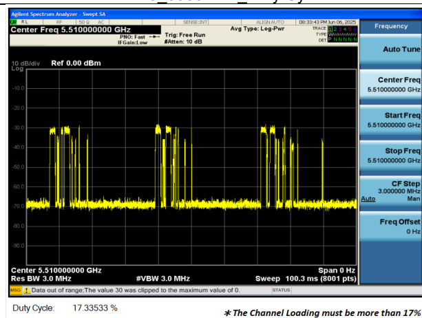
EHT40_5510MHz_Duty Cycle
