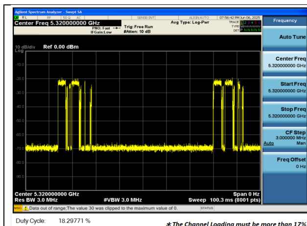
EHT20_5320MHz_Duty Cycle
