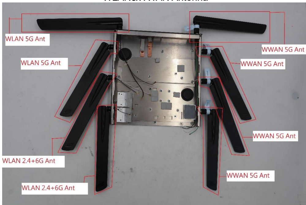
WLAN&WWAN Antenna
