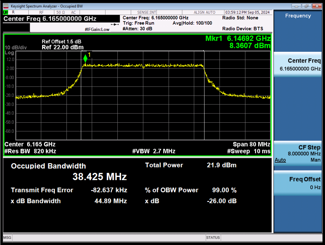
11AX40SISO-Ant1-6165-PASS
