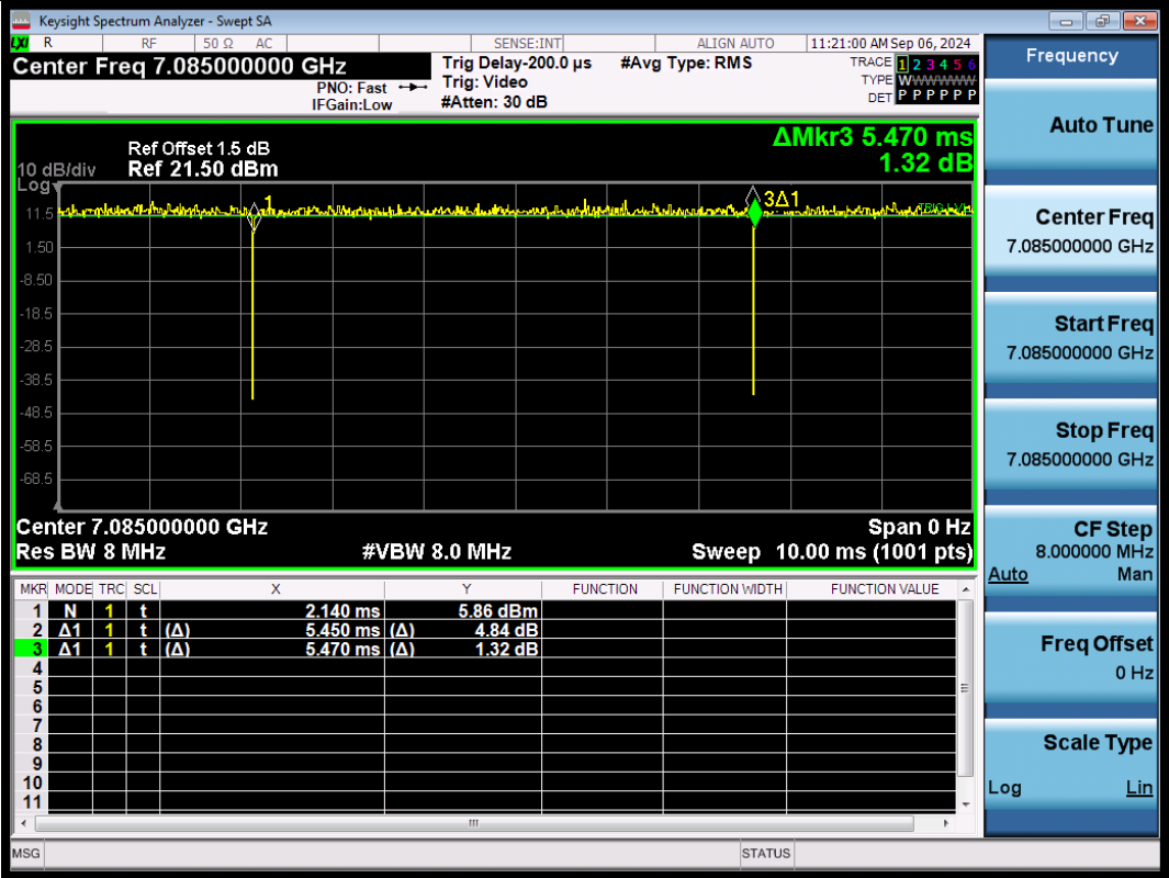
NTNV-11BE40SISO-Ant1-7085
