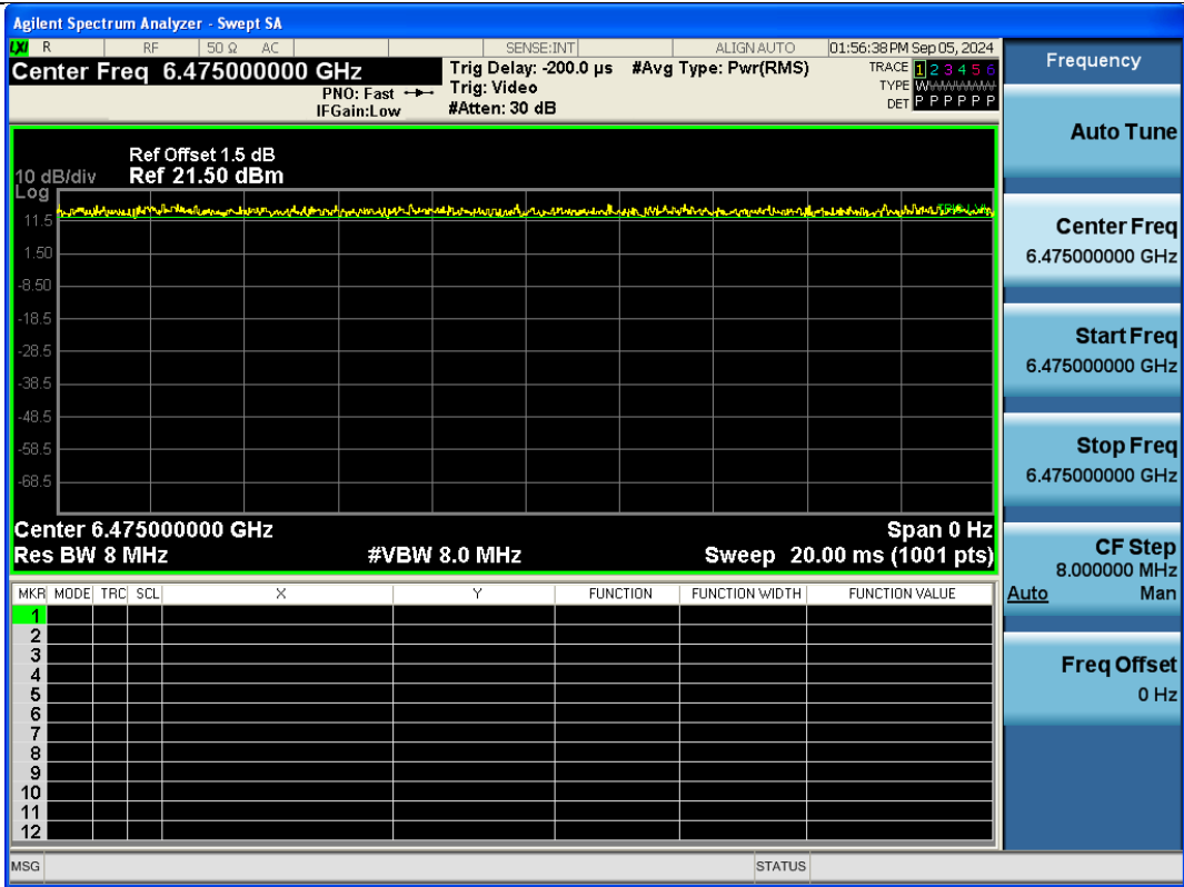
NTNV-11AX20SISO-Ant1-6475
