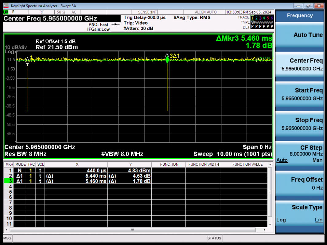
NTNV-11AX40SISO-Ant1-5965
