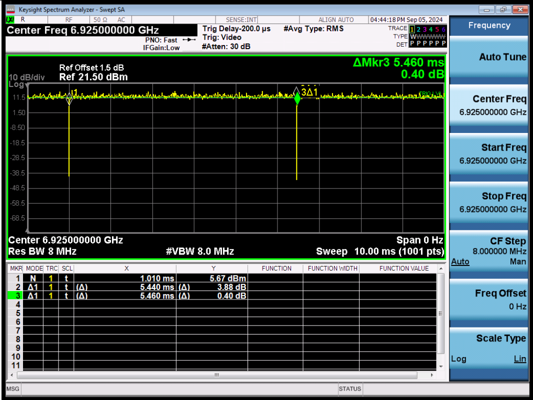
NTNV-11AX40SISO-Ant1-6925
