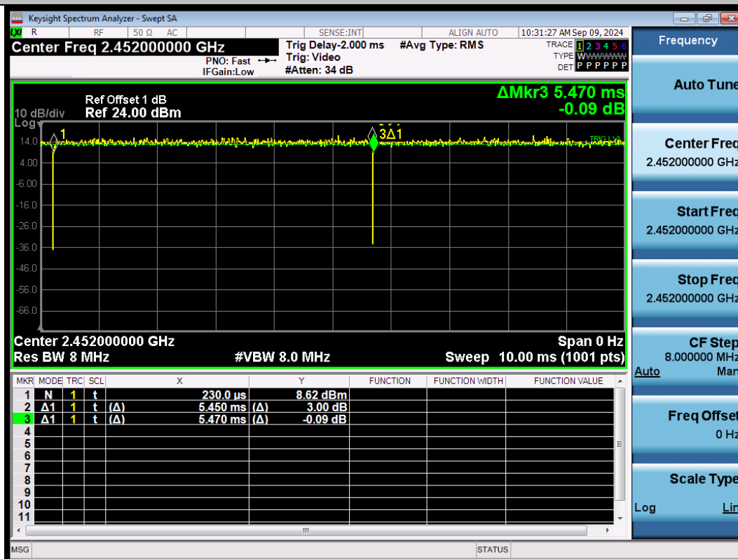
NTNV-11BE40SISO-Ant1-2452
