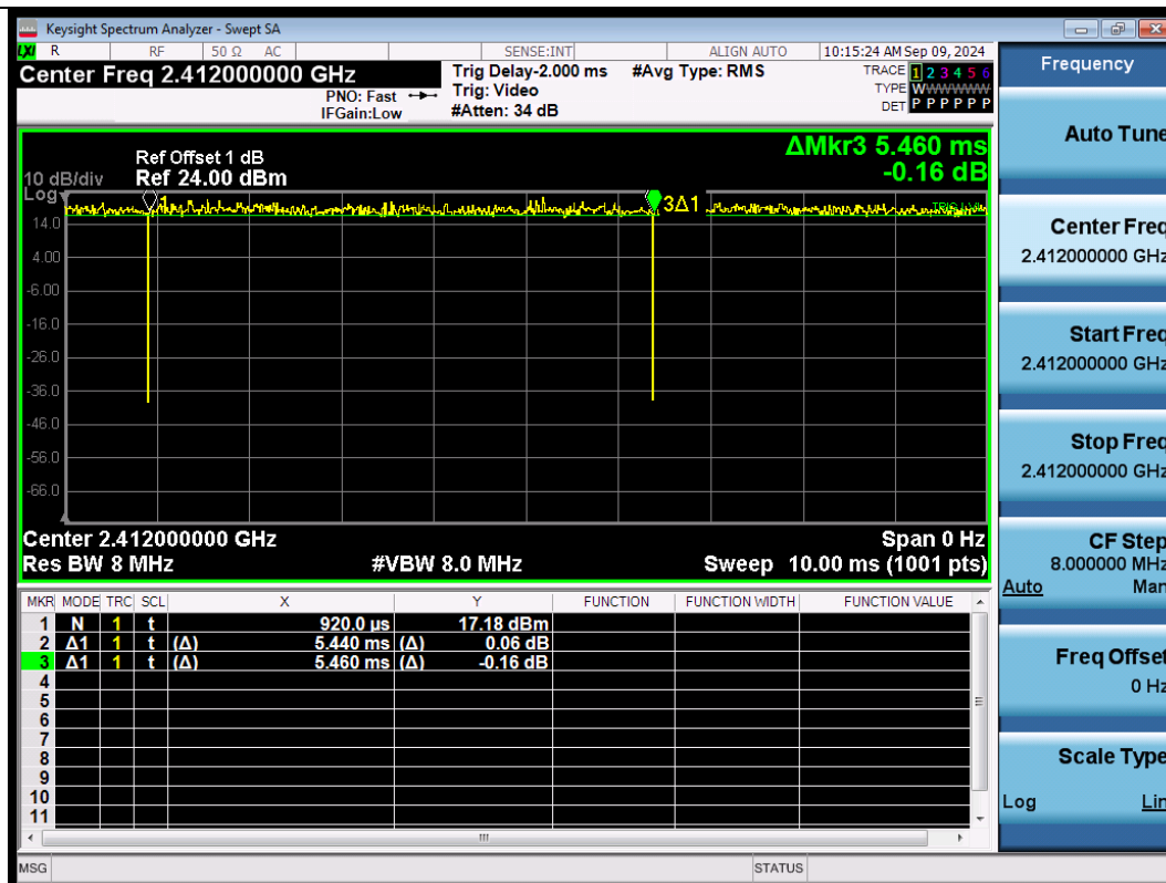
NTNV-11AX20SISO-Ant1-2412
