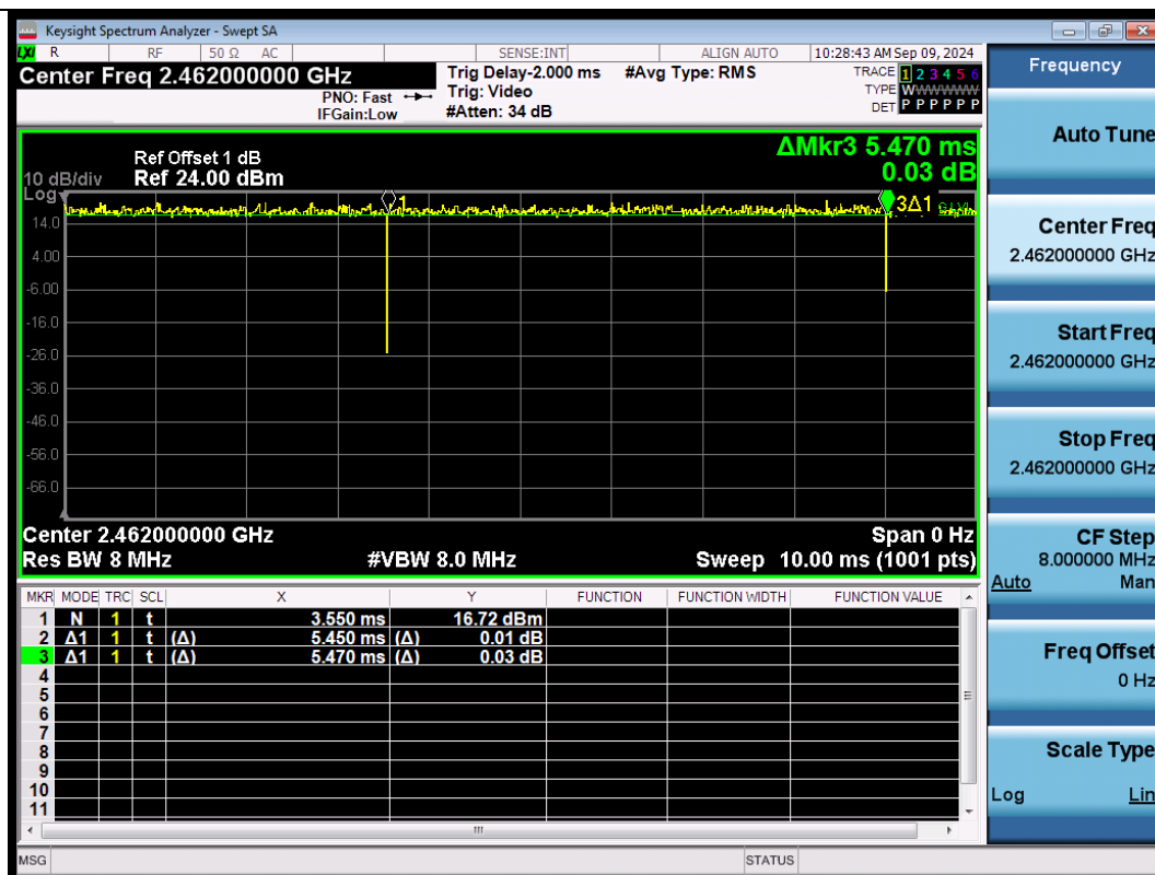
NTNV-11BE20SISO-Ant1-2462
