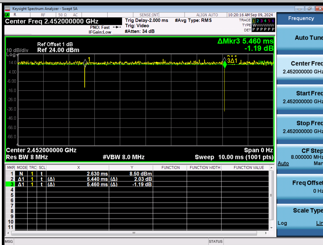
NTNV-11AX40SISO-Ant1-2452
