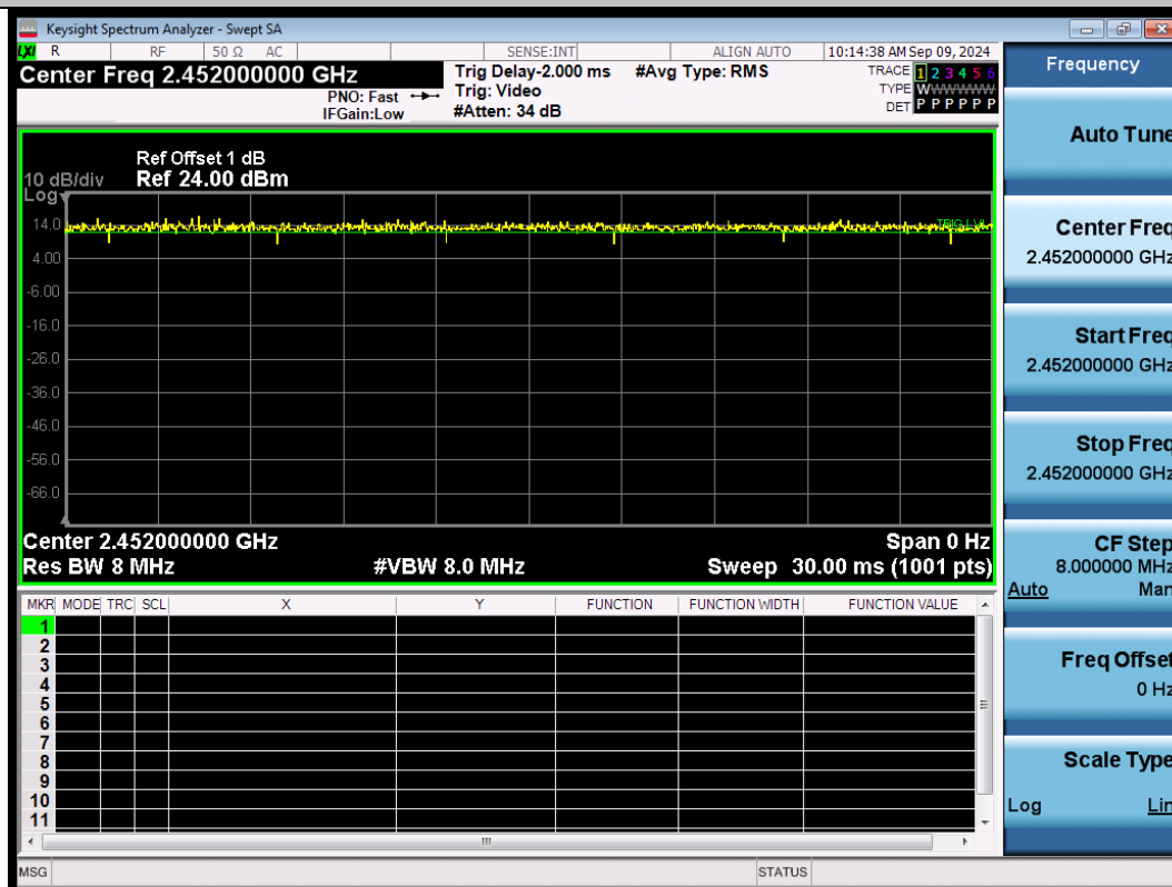
NTNV-11N40SISO-Ant1-2452
