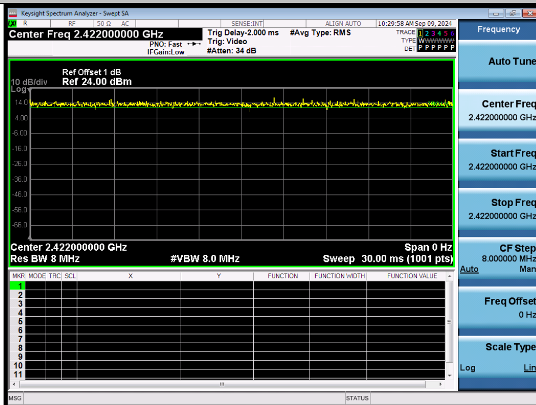
NTNV-11BE40SISO-Ant1-2422
