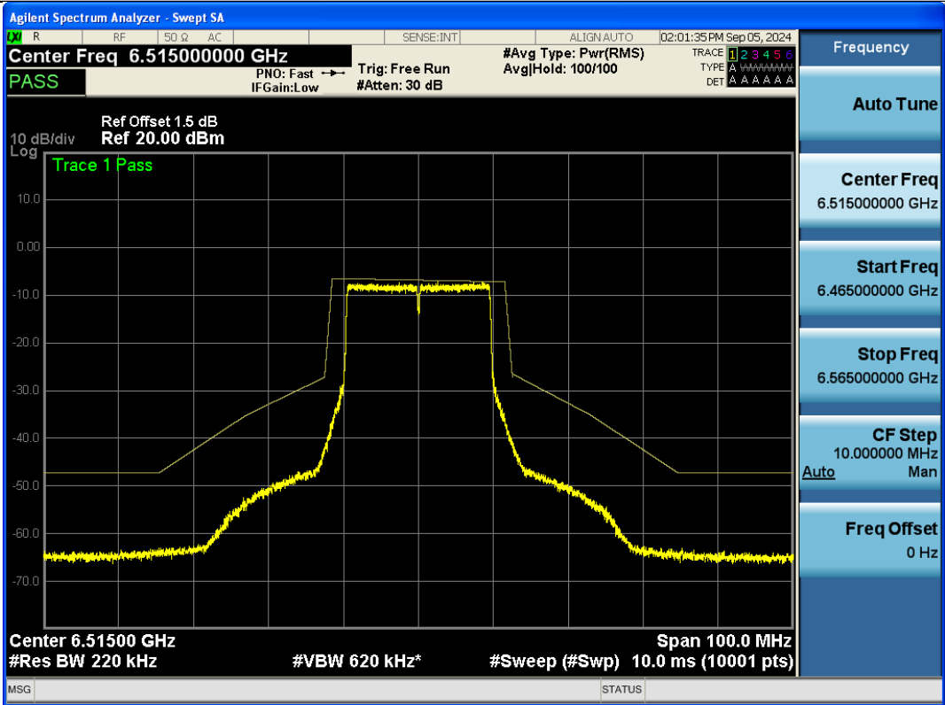
NTNV-11AX20SISO-Ant1-6515-PASS
