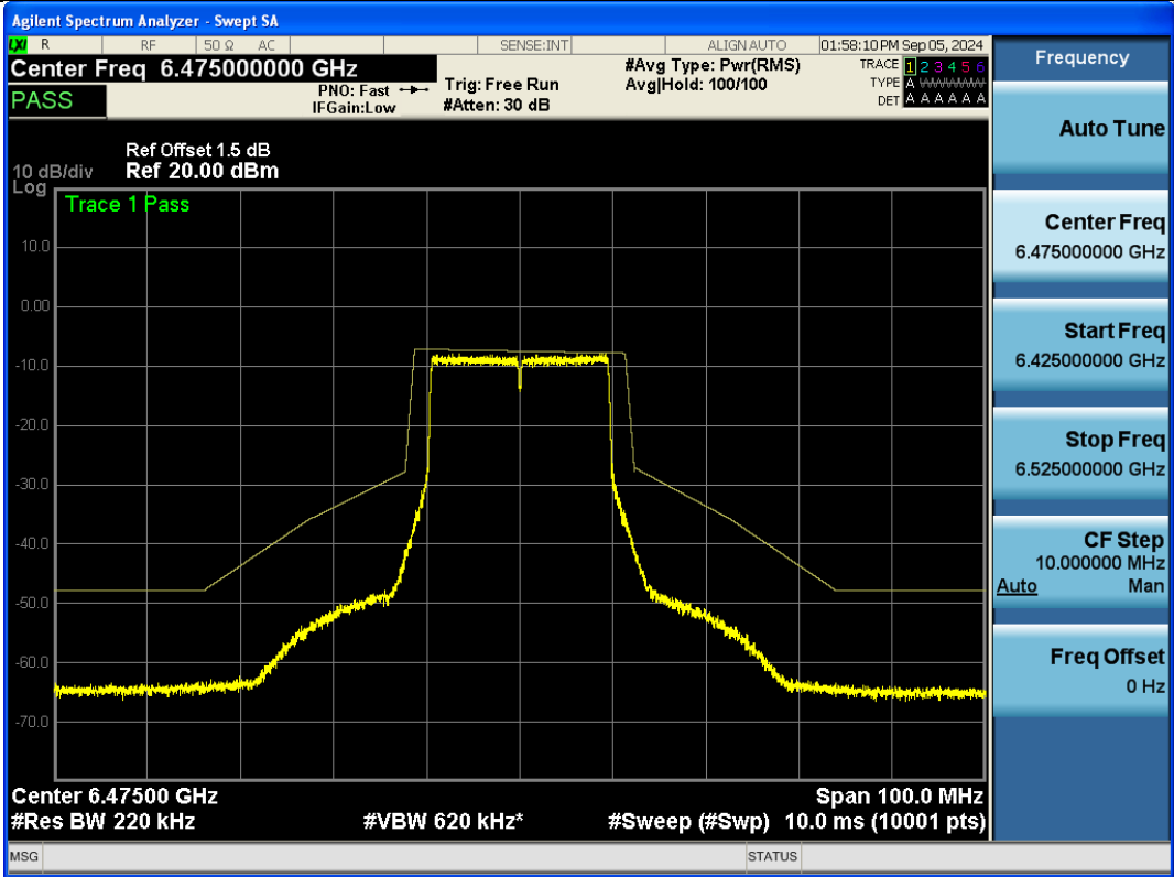
NTNV-11AX20SISO-Ant1-6475-PASS
