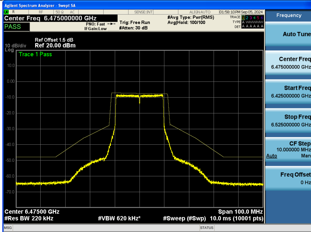
NTNV-11AX20SISO-Ant1-6475-PASS
