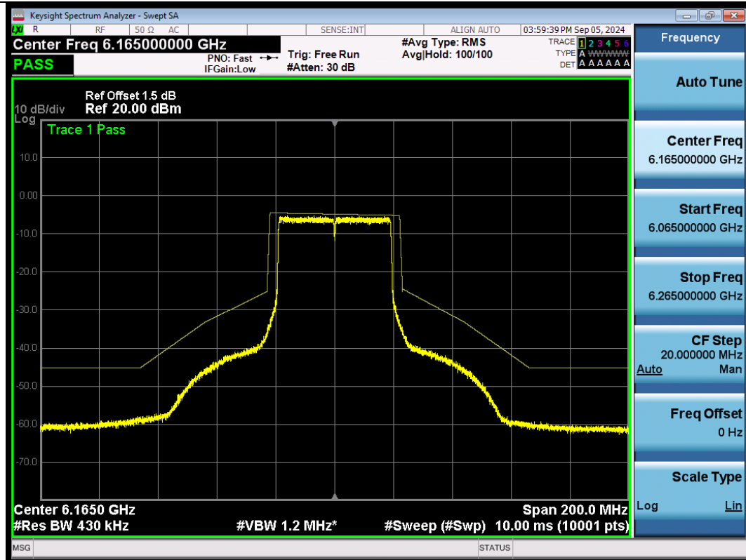
NTNV-11AX40SISO-Ant1-6165-PASS
