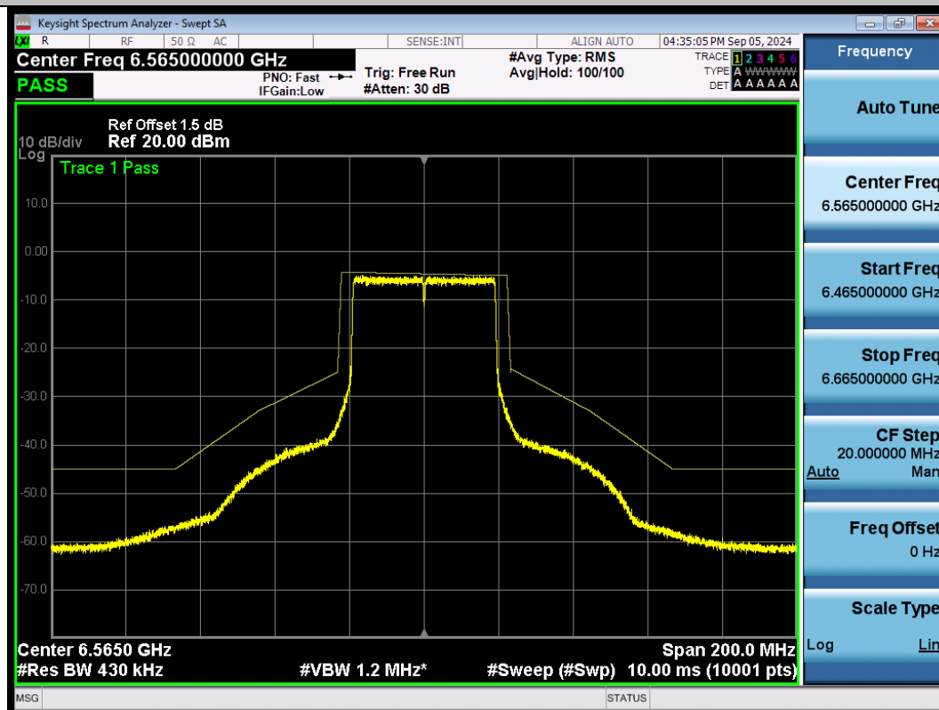
NTNV-11AX40SISO-Ant1-6565-PASS
