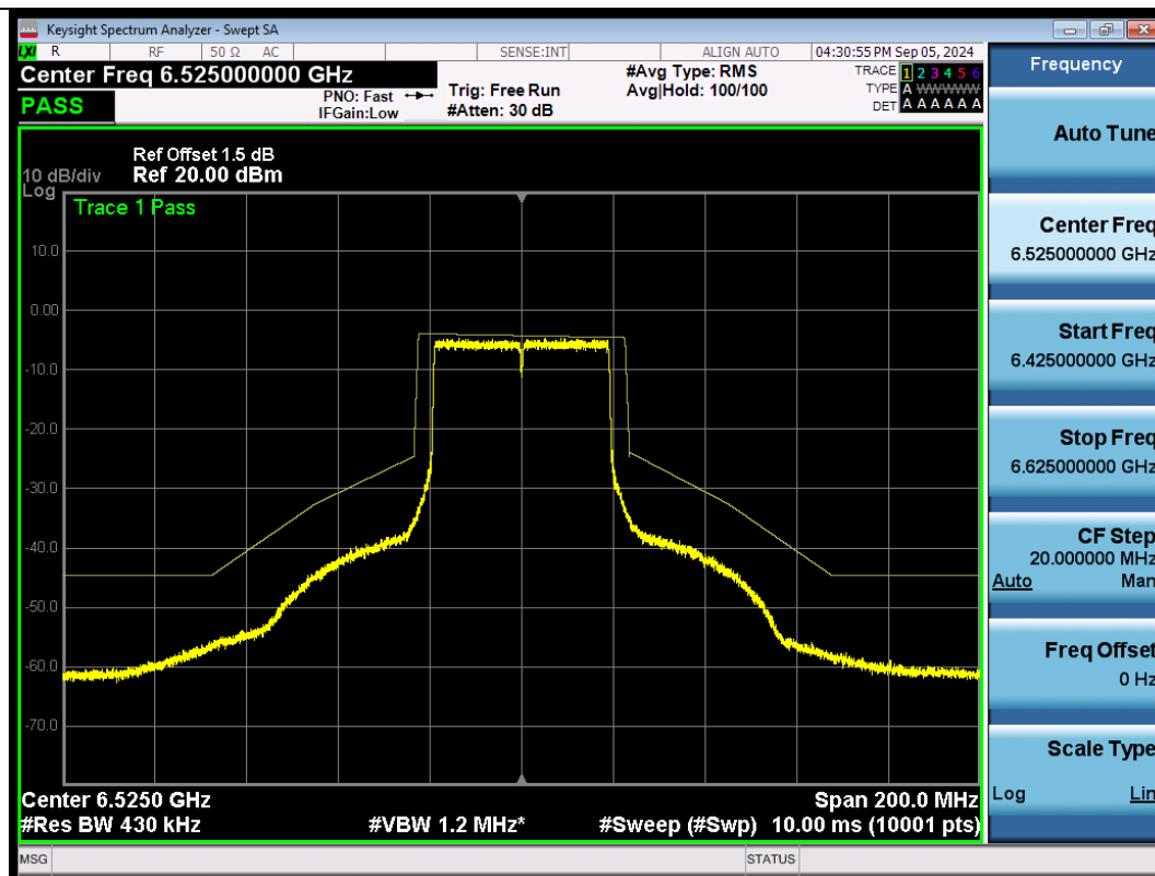
NTNV-11AX40SISO-Ant1-6525-PASS
