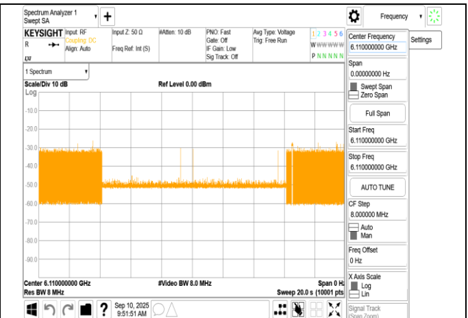
802.11be_320MHz_6265MHz_Interference_6110MHz_- 70.22dBm_Minimal
