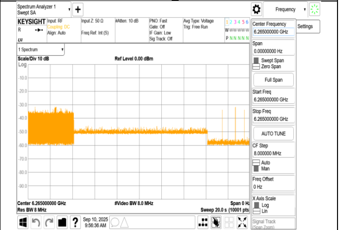
802.11be_320MHz_6265MHz_Interference_6265MHz_- 70.17dBm_OFF
