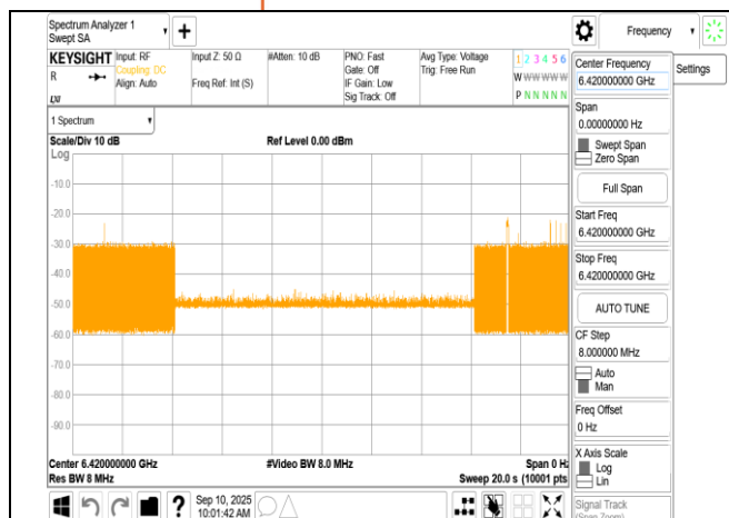
802.11be_320MHz_6265MHz_Interference_6420MHz_- 70.32dBm_OFF
