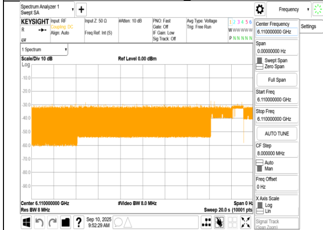
802.11be_320MHz_6265MHz_Interference_6110MHz_- 73.22dBm_ON
