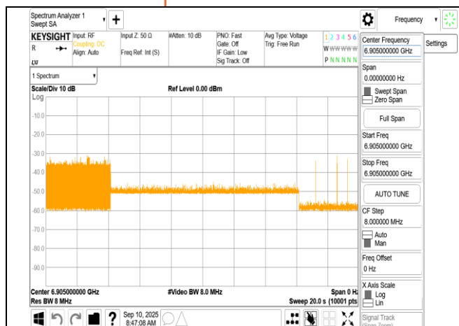
802.11be_320MHz_6905MHz_Interference_6905MHz_- 70.15dBm_OFF
