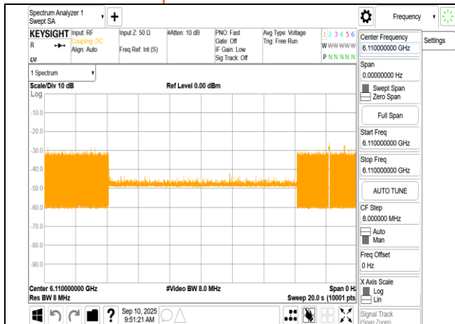
802.11be_320MHz_6265MHz_Interference_6110MHz_- 67.22dBm_OFF
