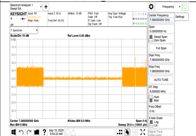
802.11be_320MHz_6905MHz_Interference_7060MHz_- 70.23dBm_OFF
