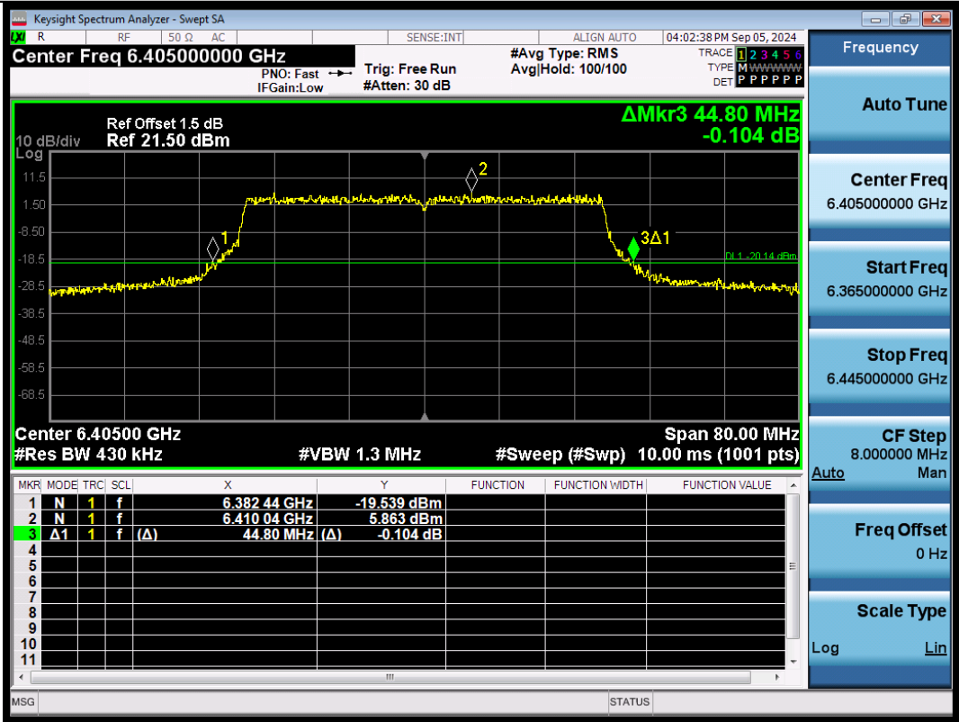
11AX40SISO-Ant1-6405
