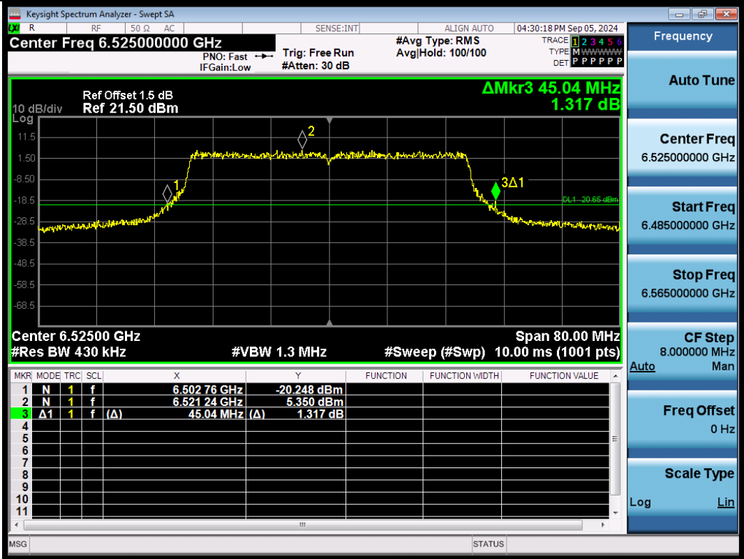
11AX40SISO-Ant1-6525
