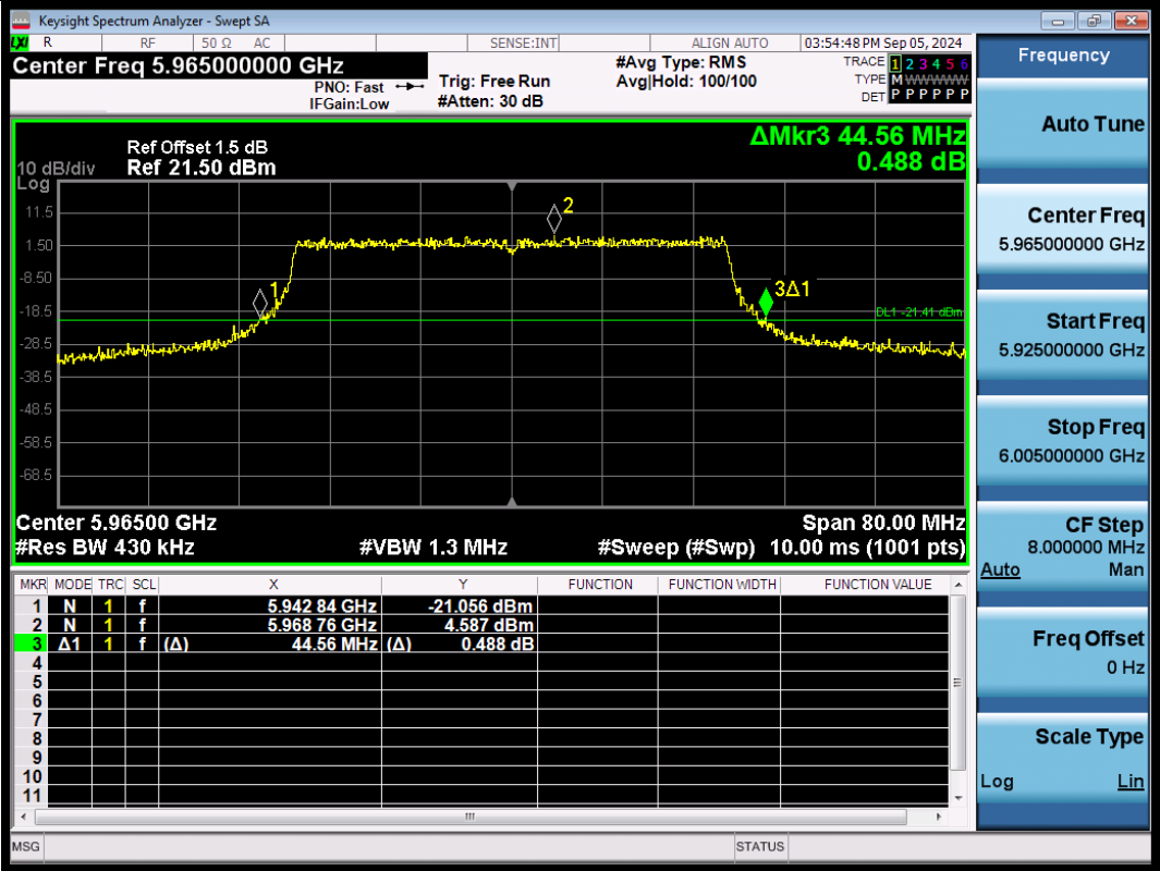
11AX40SISO-Ant1-5965
