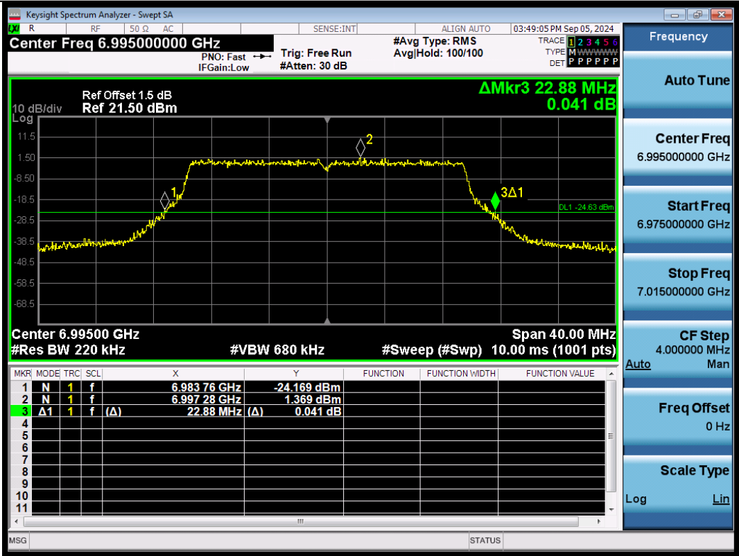
11AX20SISO-Ant1-6995
