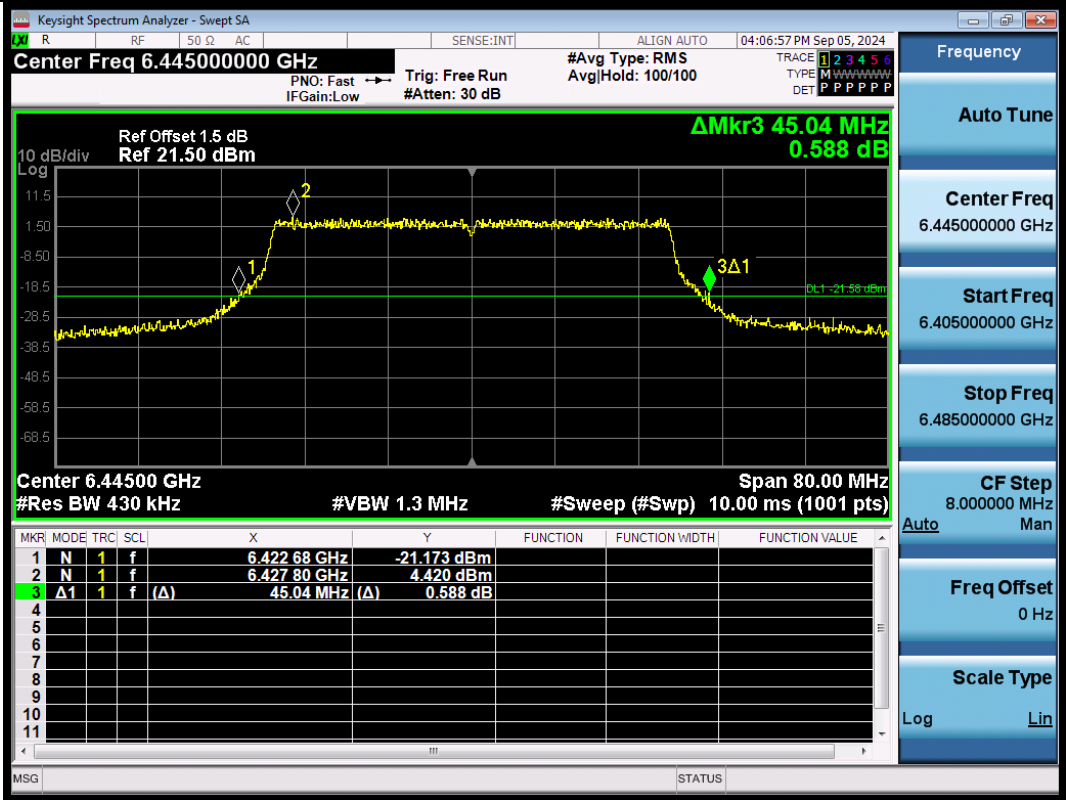
11AX40SISO-Ant1-6445
