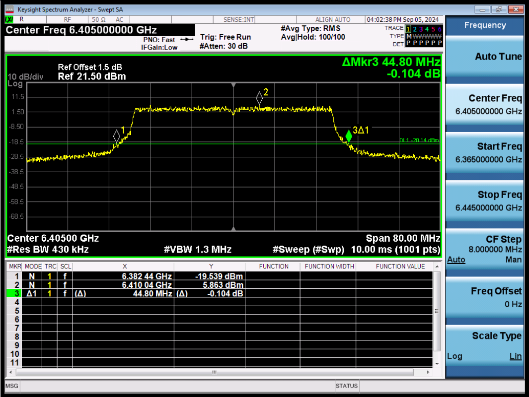
11AX40SISO-Ant1-6405
