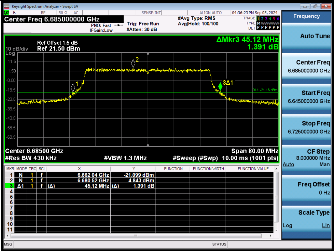
11AX40SISO-Ant1-6685
