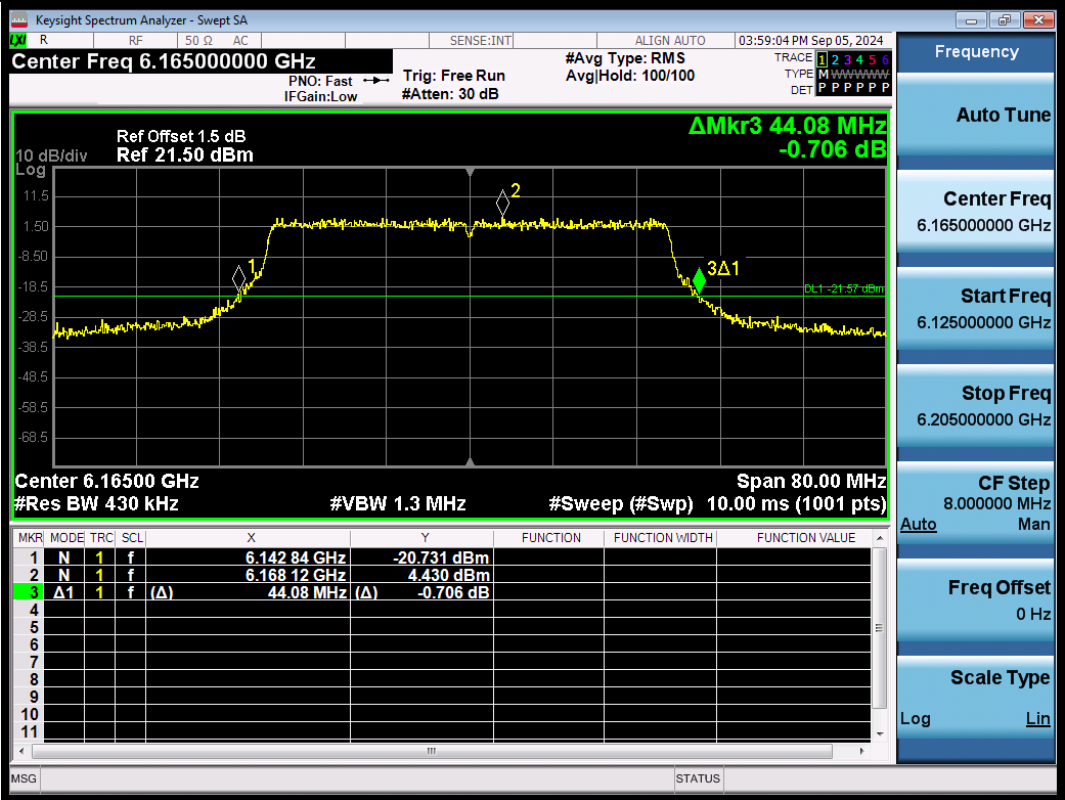
11AX40SISO-Ant1-6165
