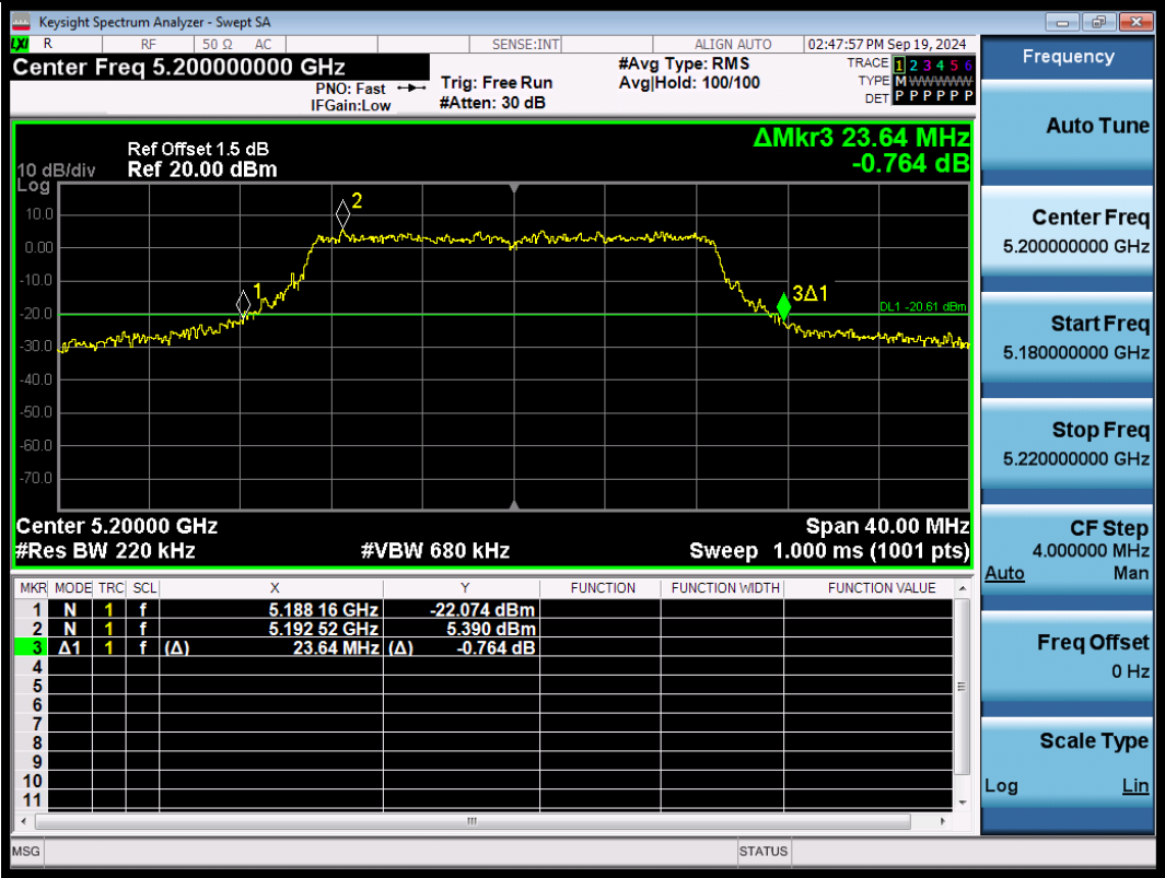
11AC20SISO-Ant1-5200
