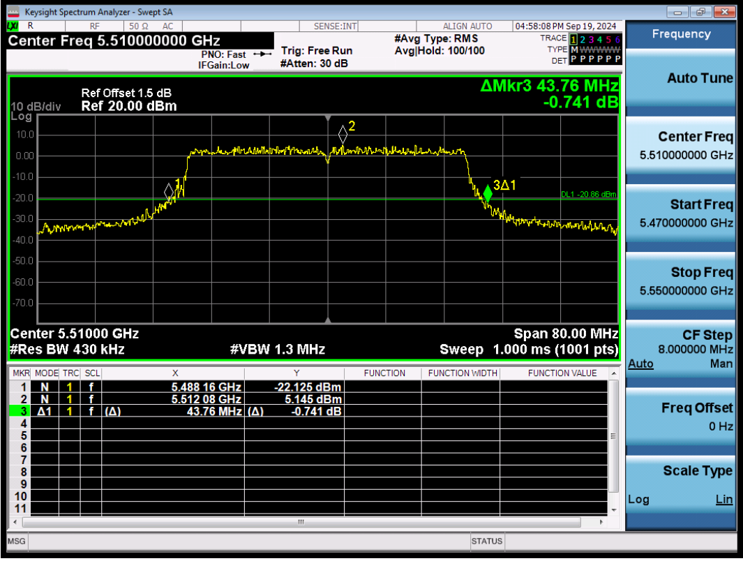
11AX40SISO-Ant1-5510
