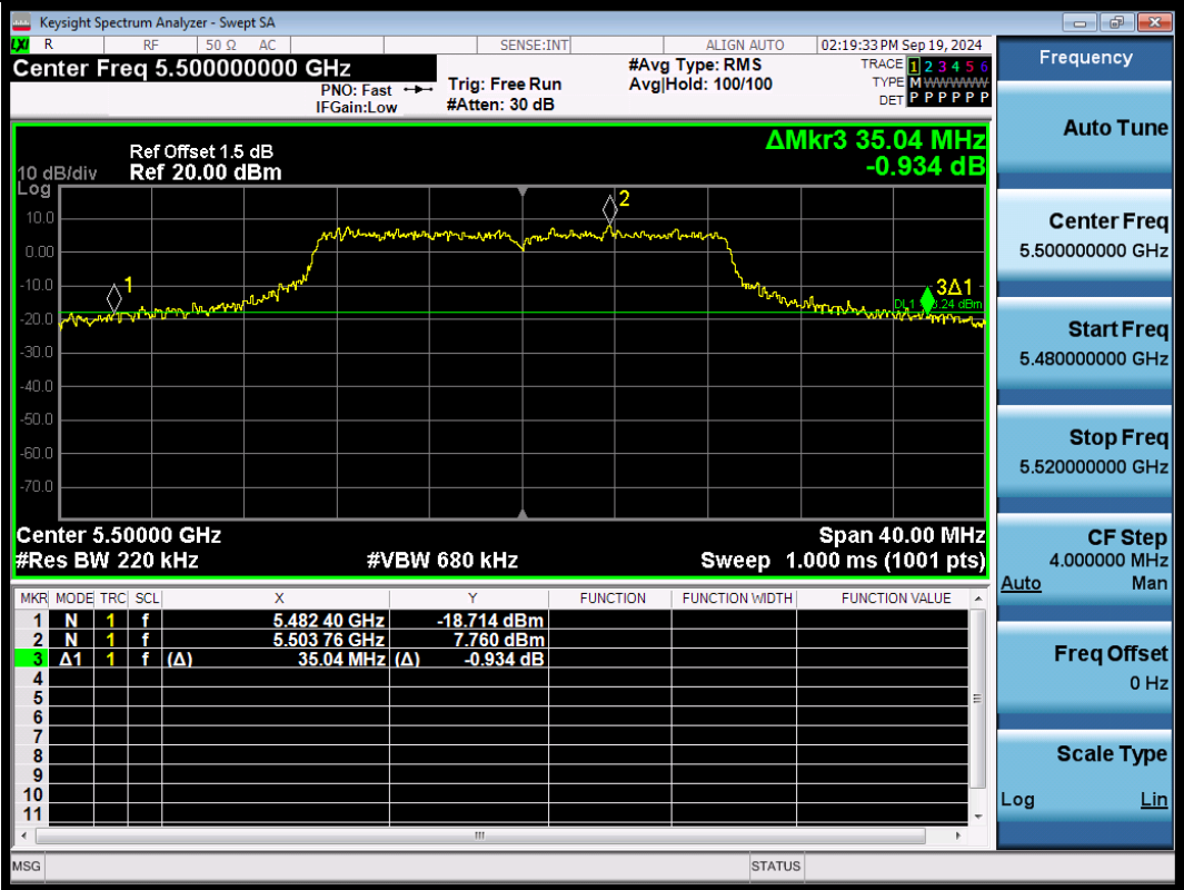
11N20SISO-Ant1-5500
