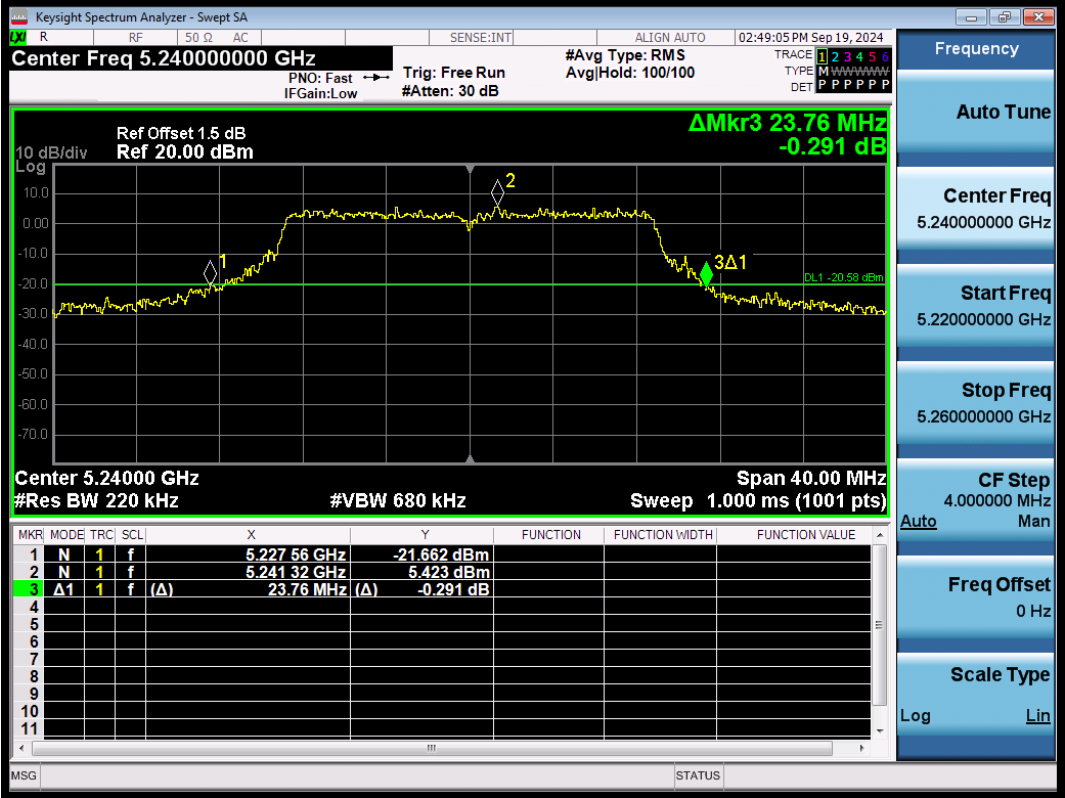
11AC20SISO-Ant1-5240
