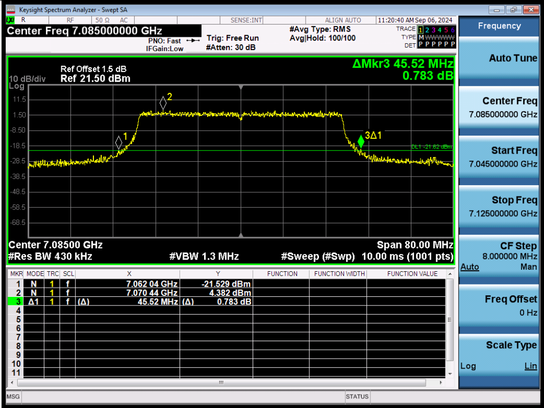
11BE40SISO-Ant1-7085
