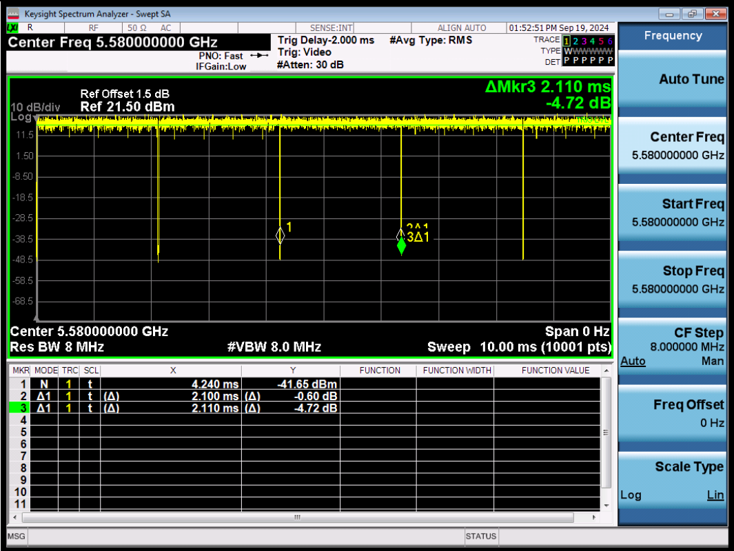
NTNV-11A-Ant1-5580
