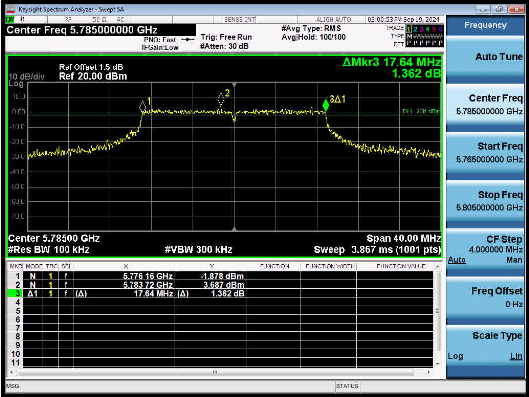
11AC20SISO-Ant1-5785-PASS
