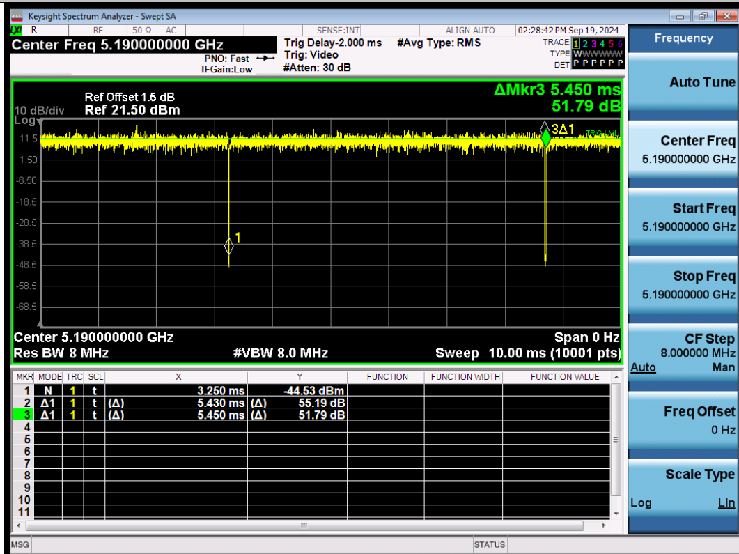
NTNV-11N40SISO-Ant1-5190
