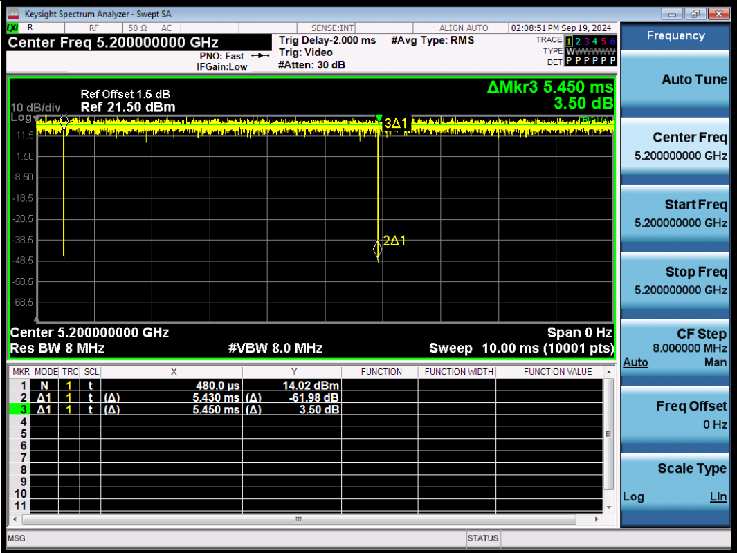
NTNV-11N20SISO-Ant1-5200
