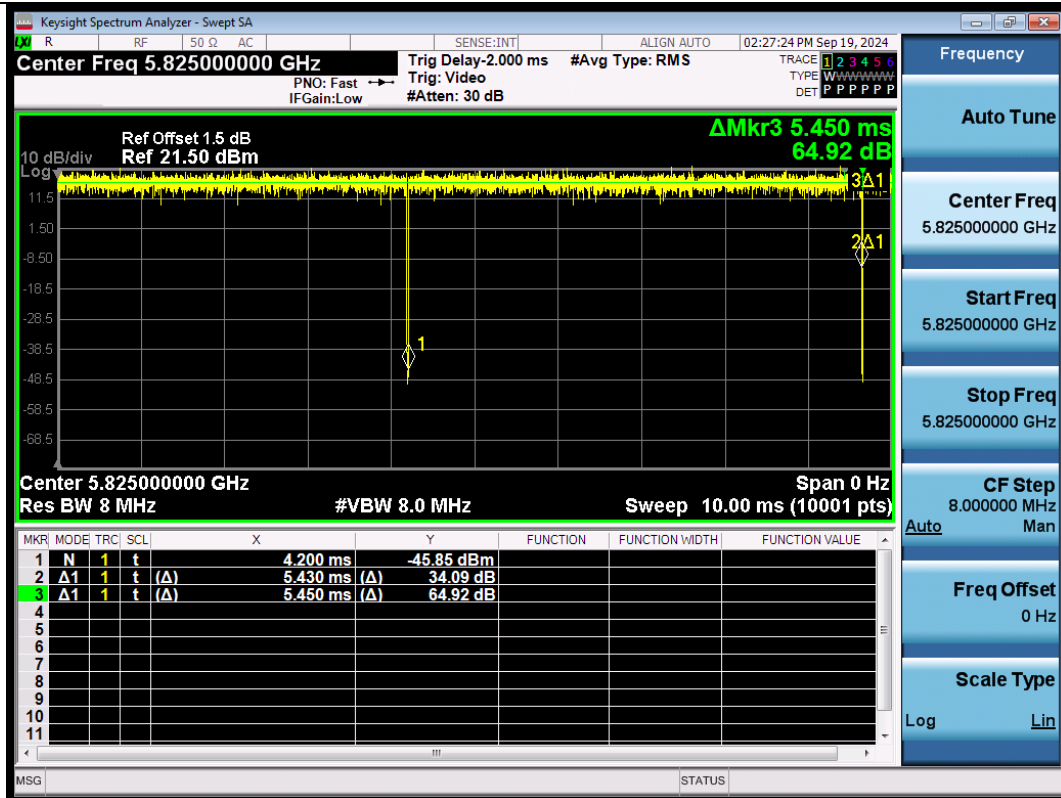
NTNV-11N20SISO-Ant1-5825
