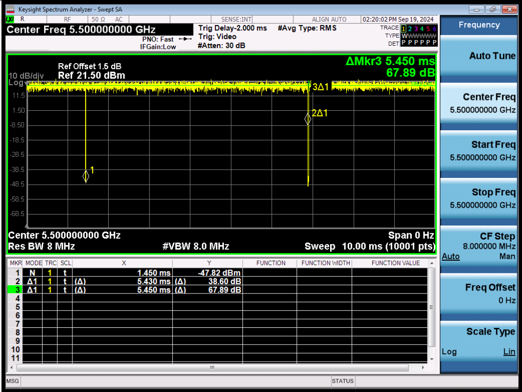
NTNV-11N20SISO-Ant1-5500
