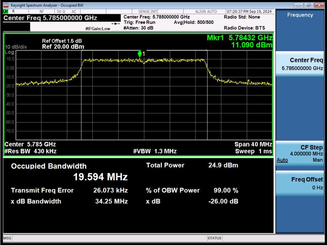
11BE20SISO-Ant1-5785
