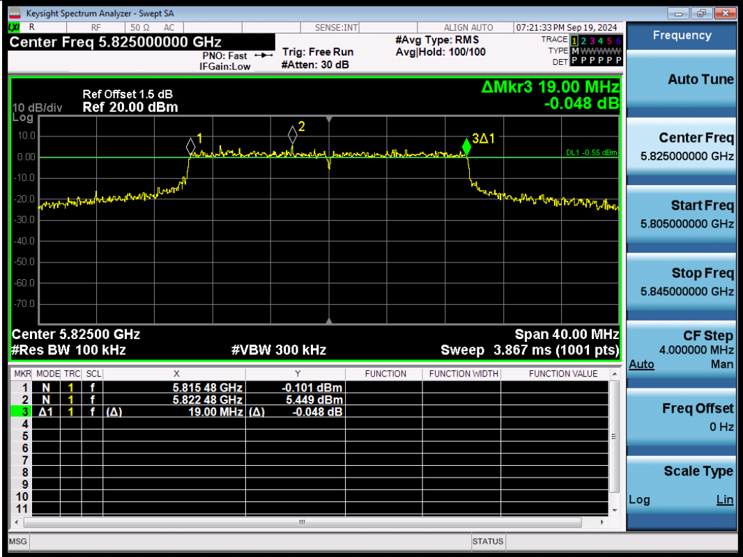
11BE20SISO-Ant1-5825-PASS
