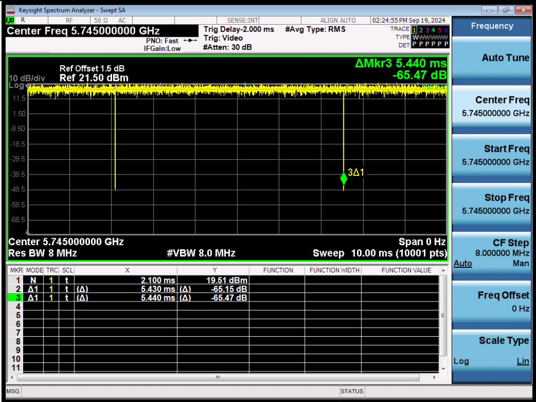
NTNV-11N20SISO-Ant1-5745
