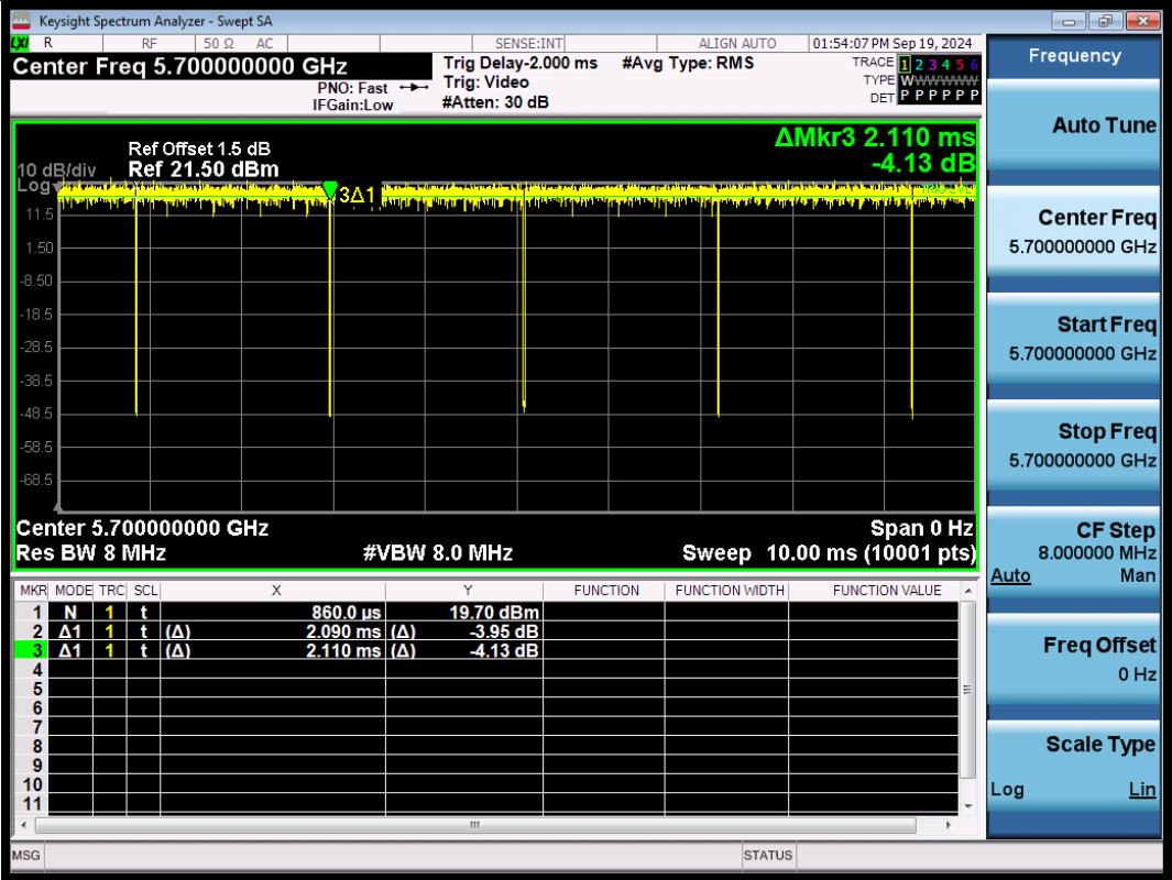
NTNV-11A-Ant1-5700
