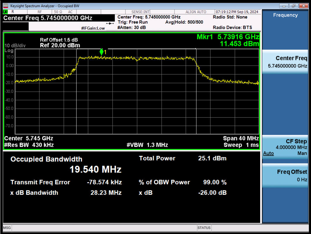
11BE20SISO-Ant1-5745
