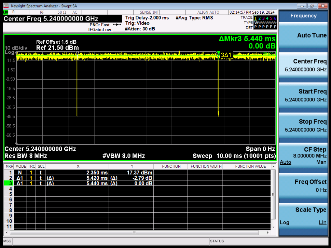
NTNV-11N20SISO-Ant1-5240
