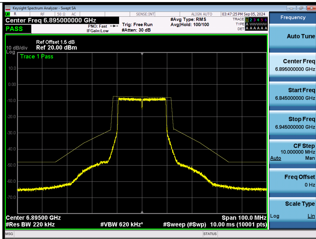
NTNV-11AX20SISO-Ant1-6895-PASS
