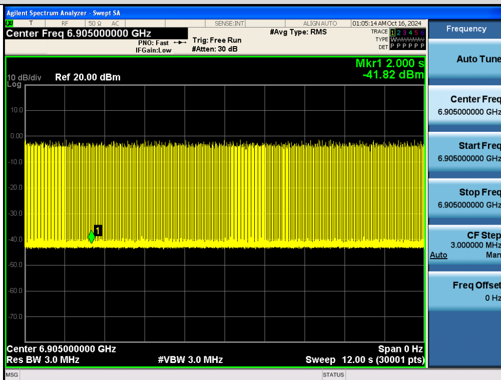
802.11 BE (320MHz) 6905 -7060MHz - Normal Operation
