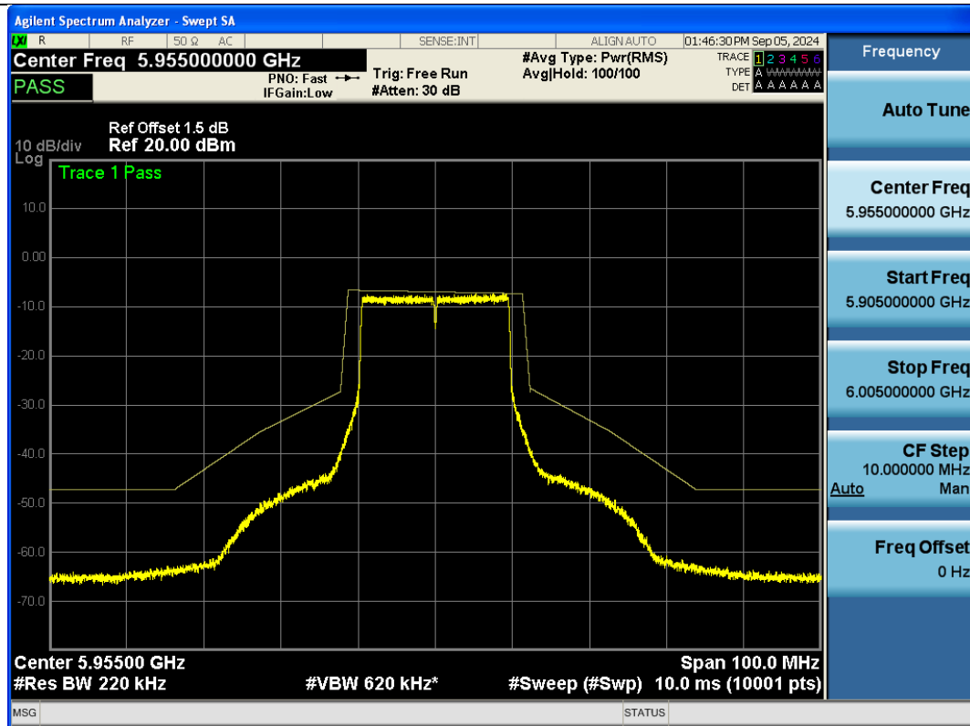
NTNV-11AX20SISO-Ant1-5955-PASS
