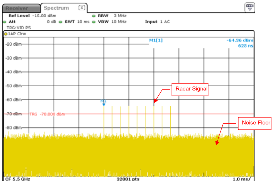
Radar Signal 6
