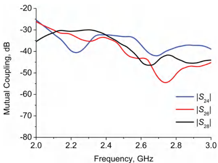
Mutual Coupling
