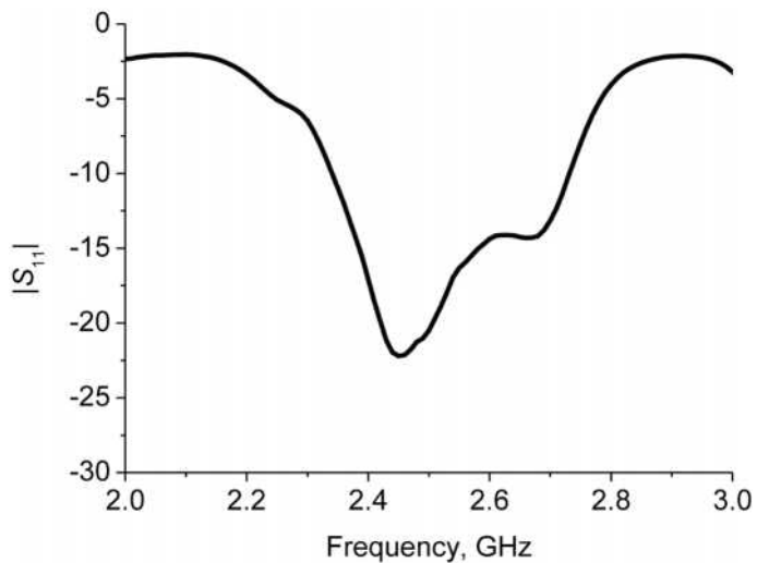
Return Loss
