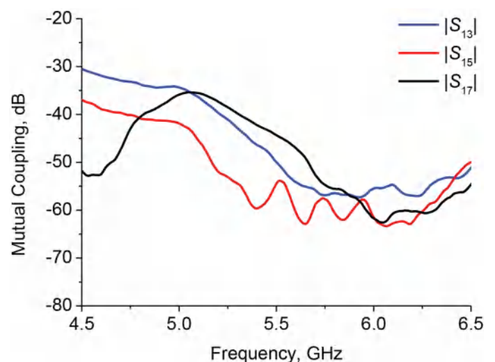
Mutual Coupling
