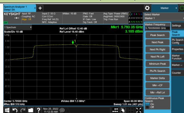
Channel 159 (5795MHz)
