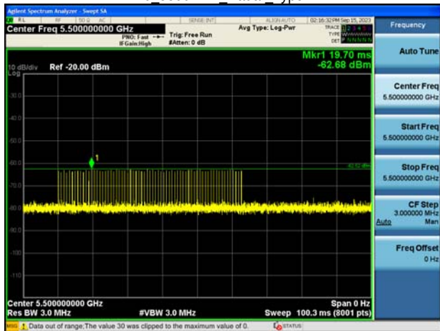
HE20 5500MHz Radar Type 1-B
