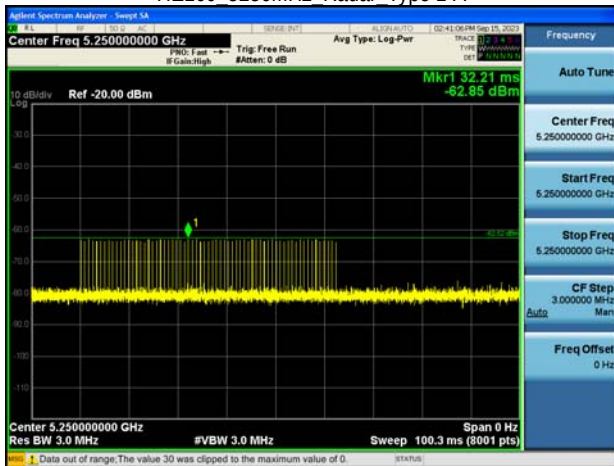
HE160 5250MHz Radar Type 1-B
