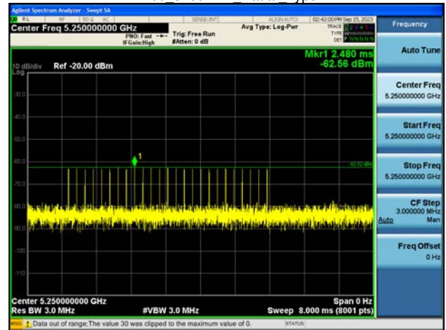
HE160 5250MHz Radar Type 3
