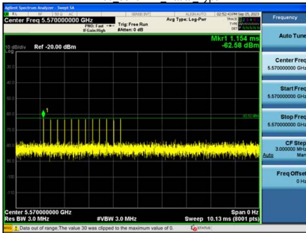
HE160 5570MHz Radar Type 5
