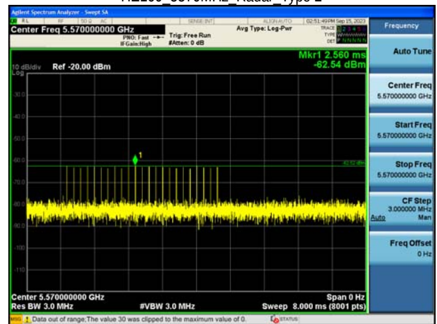
HE160 5570MHz Radar Type 2
