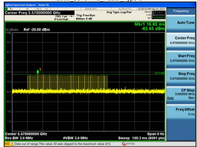
HE160 5570MHz Radar Type 1-B
