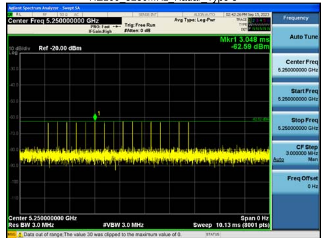
HE160 5250MHz Radar Type 4
