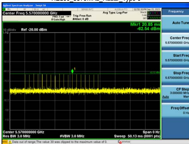
HE160 5570MHz Radar Type 0
