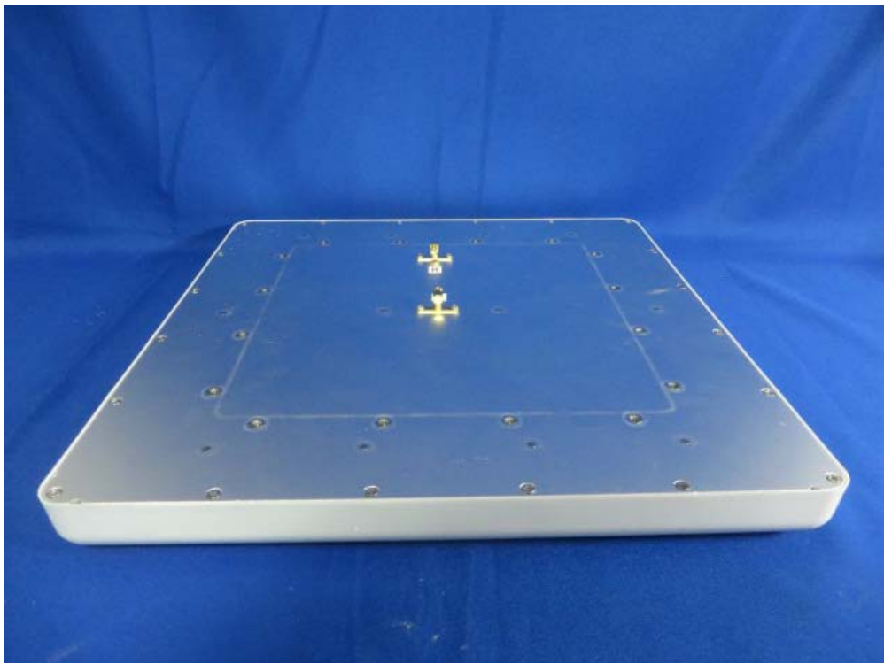
(18) EUT Photo (Panel Antenna 23dBi)
