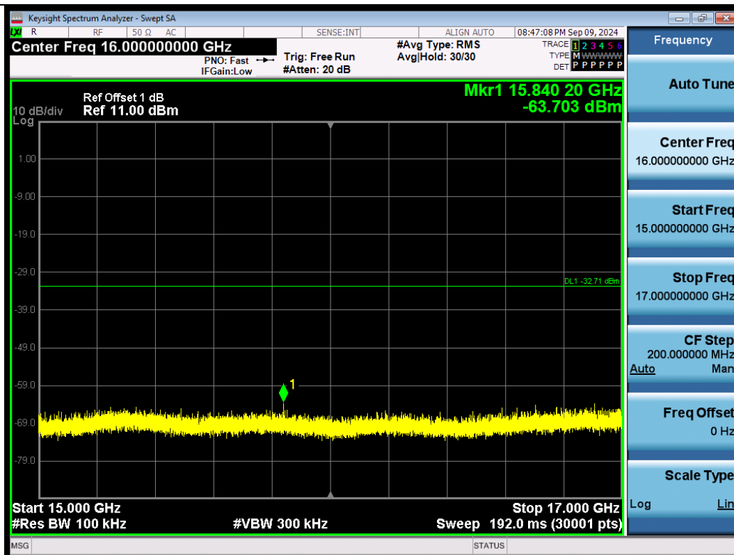
11N40SISO-Ant1-2422-15000~17000-PASS
