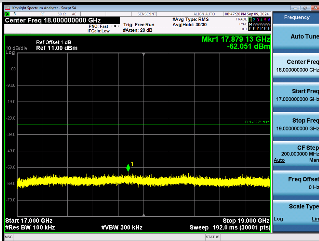
11N40SISO-Ant1-2422-17000~19000-PASS
