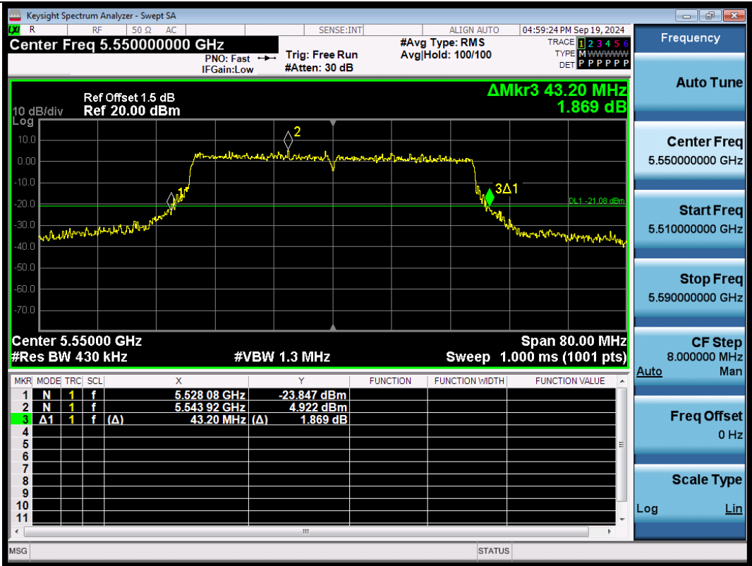
11AX40SISO-Ant1-5550
