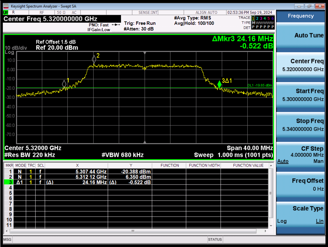
11AC20SISO-Ant1-5320
