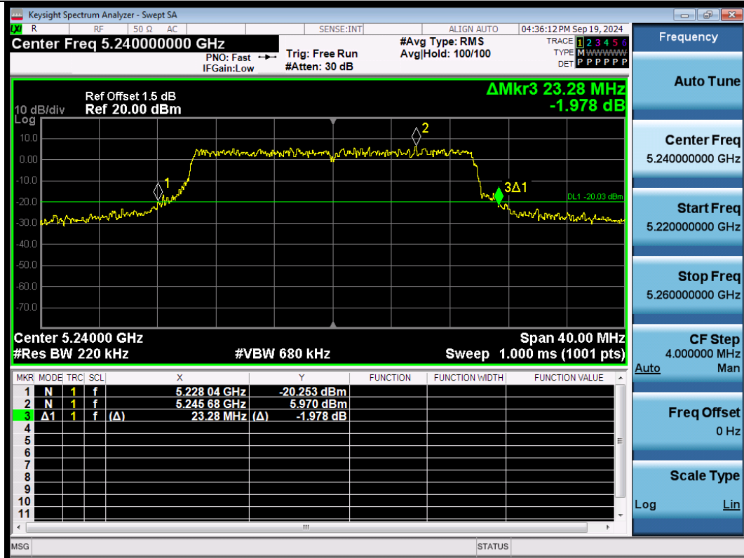
11AX20SISO-Ant1-5240
