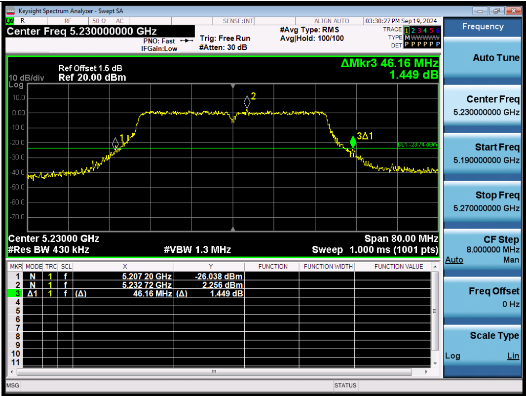
11AC40SISO-Ant1-5230
