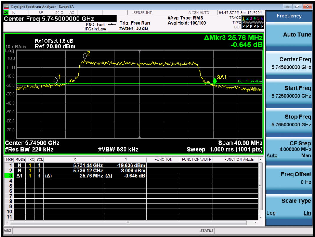
11AX20SISO-Ant1-5745
