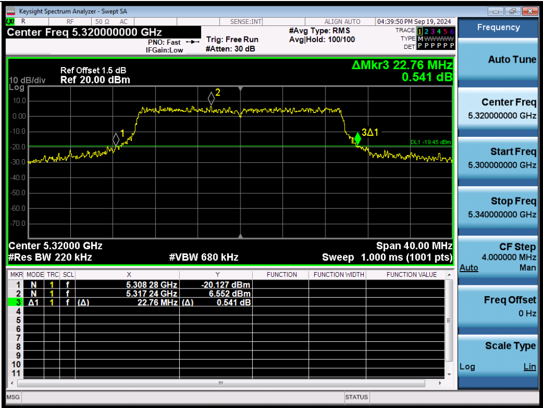
11AX20SISO-Ant1-5320
