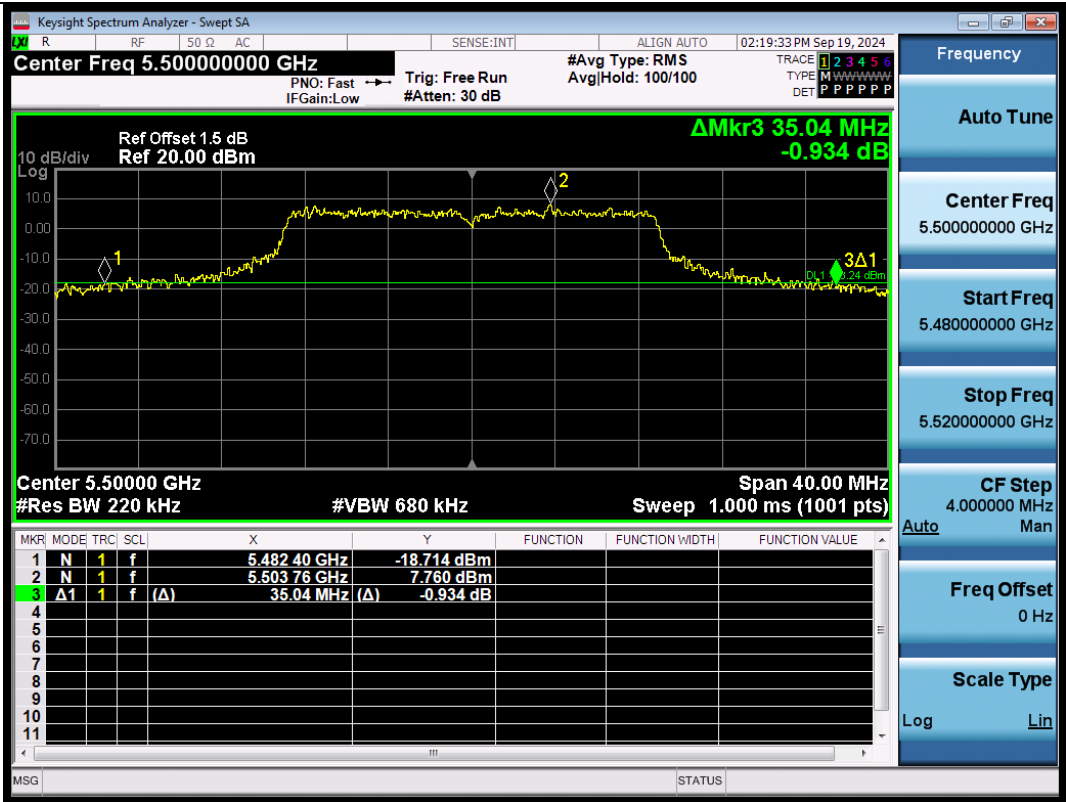
11N20SISO-Ant1-5500
