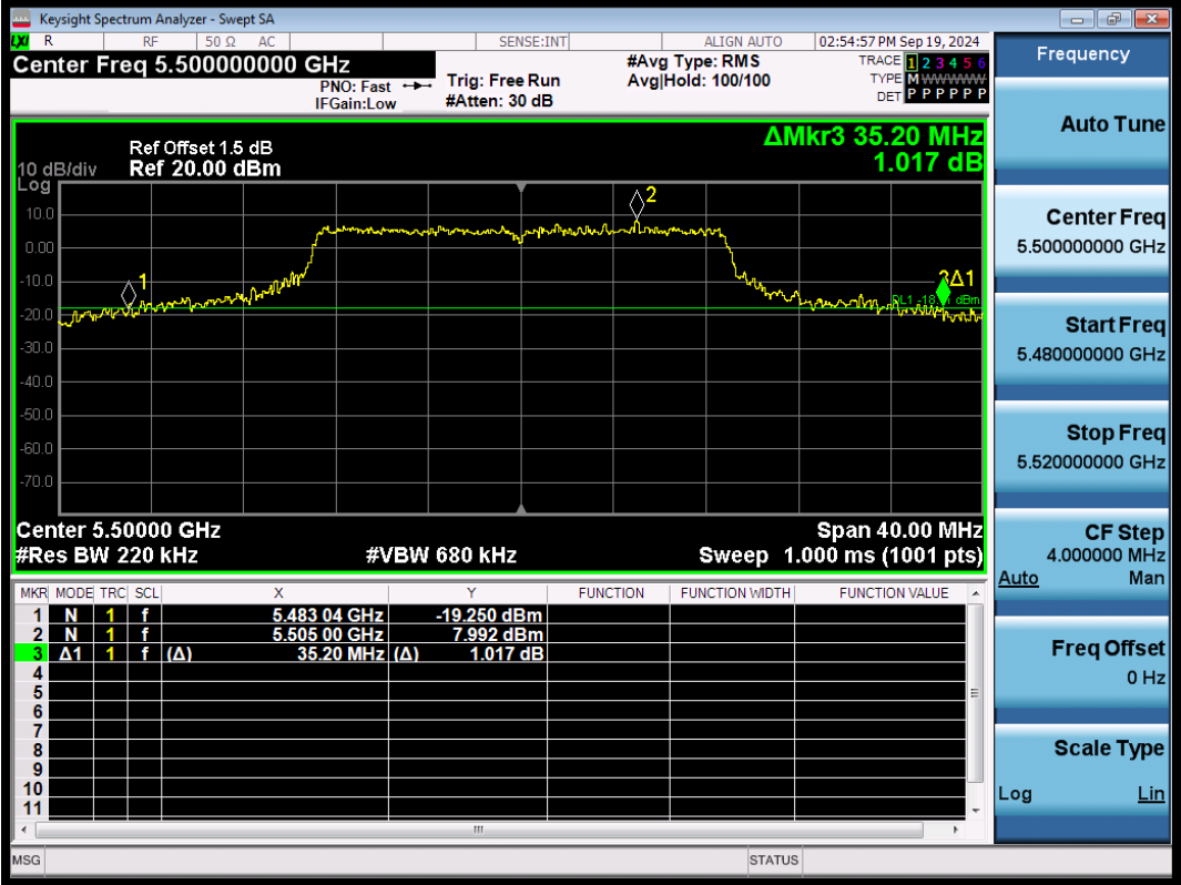
11AC20SISO-Ant1-5500
