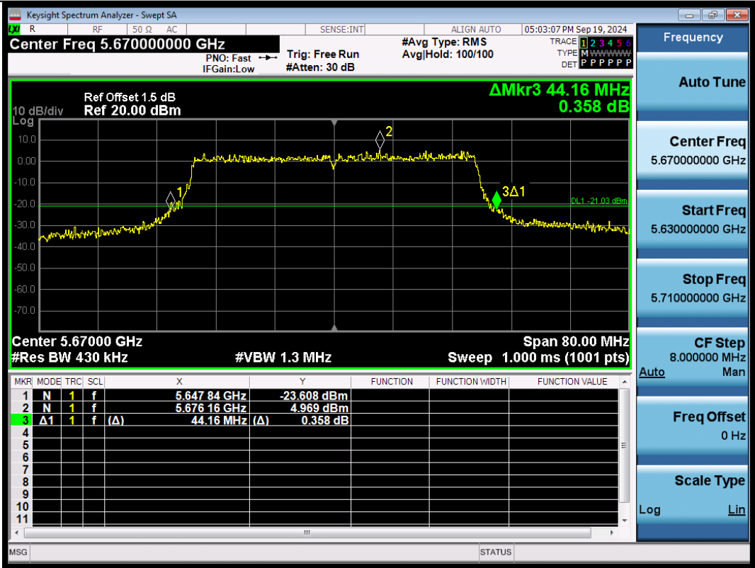
11AX40SISO-Ant1-5670
