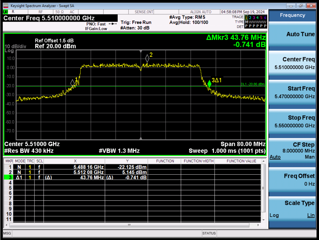
11AX40SISO-Ant1-5510
