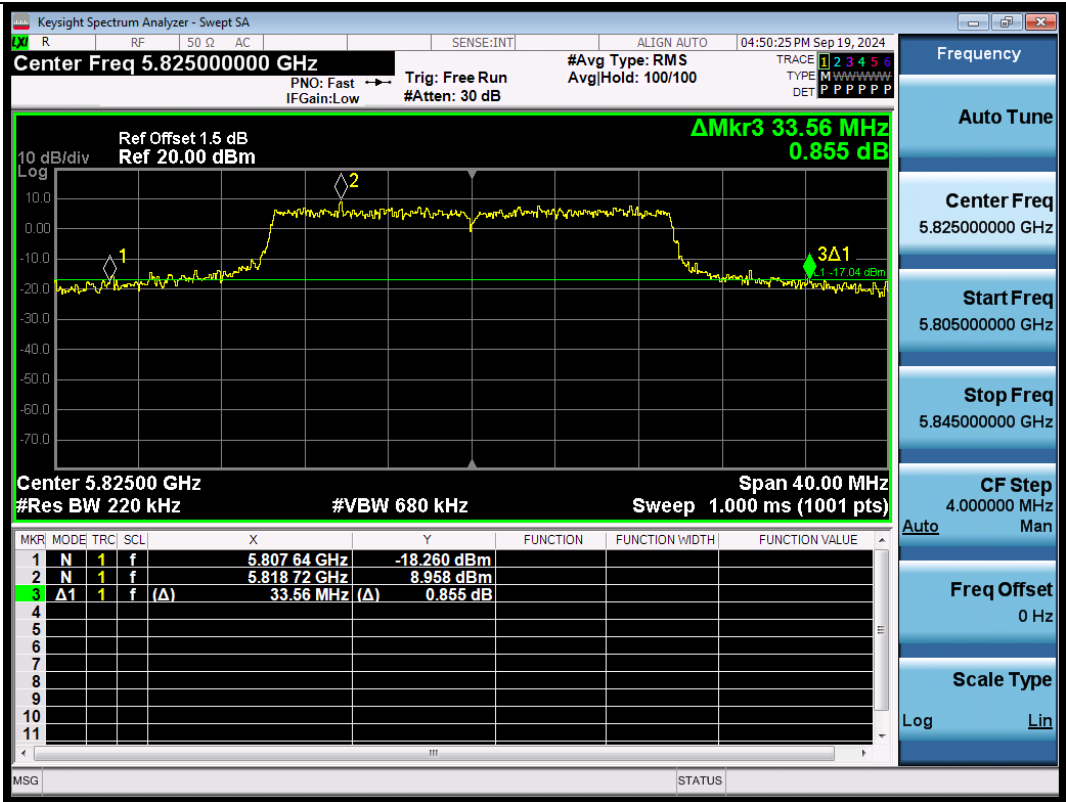
11AX20SISO-Ant1-5825
