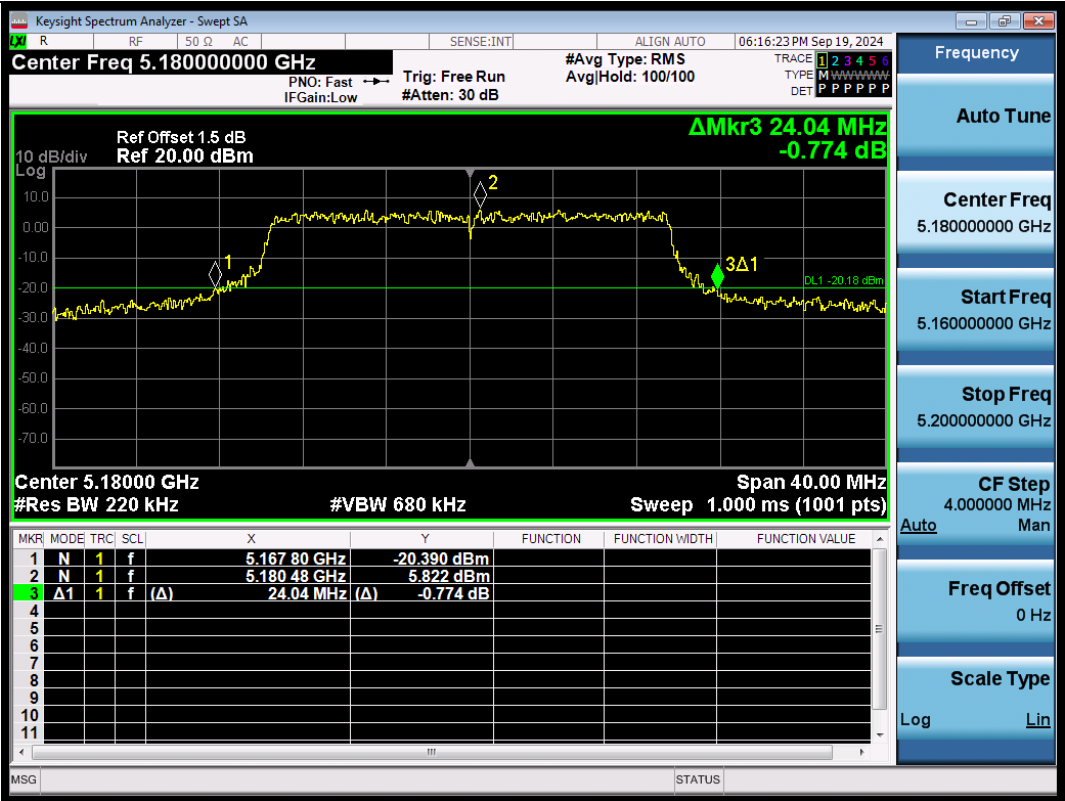
11BE20SISO-Ant1-5180
