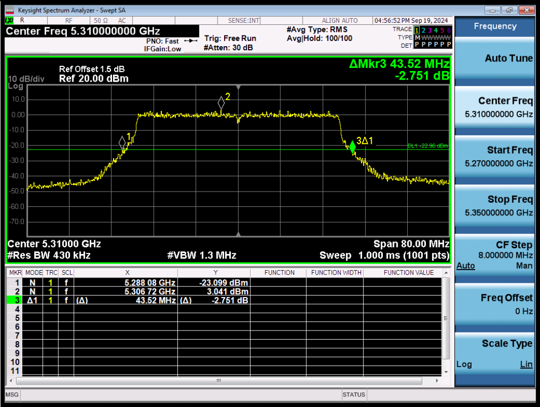
11AX40SISO-Ant1-5310
