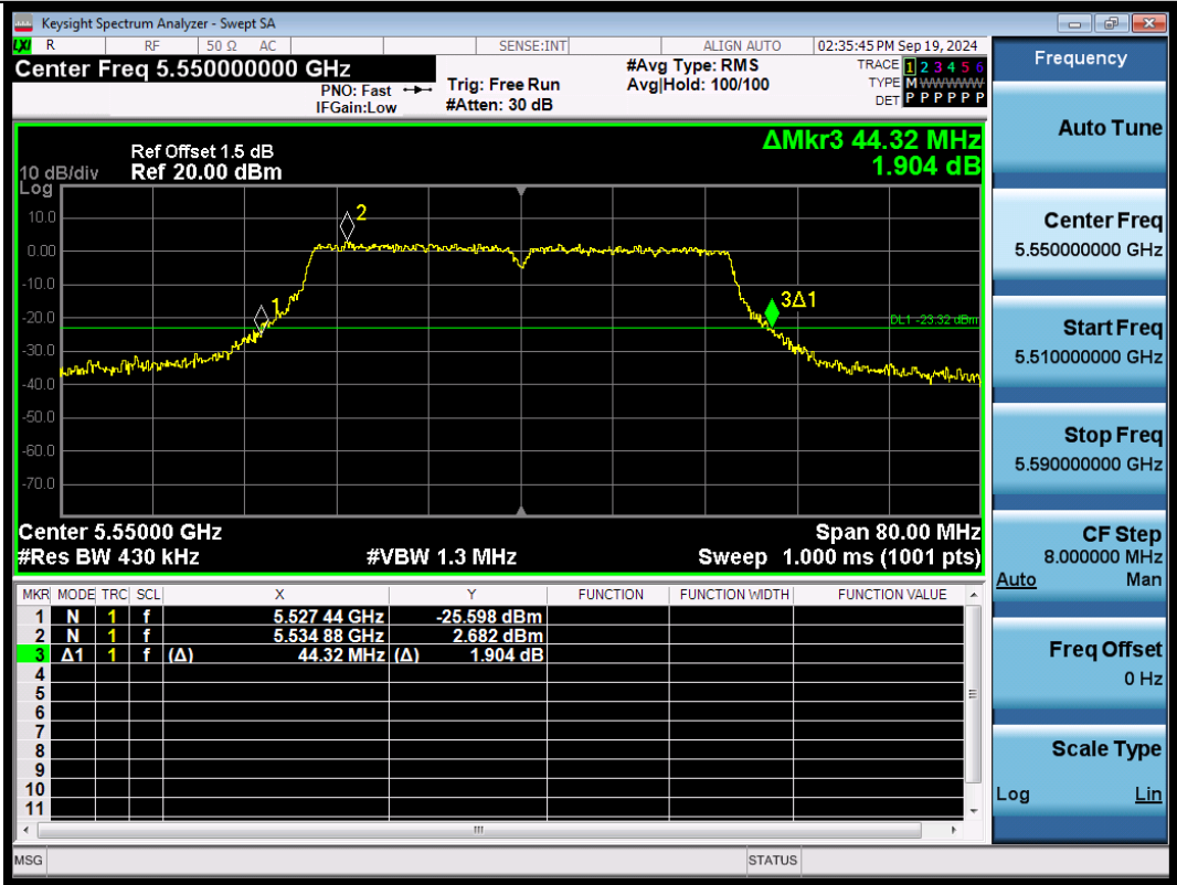
11N40SISO-Ant1-5550
