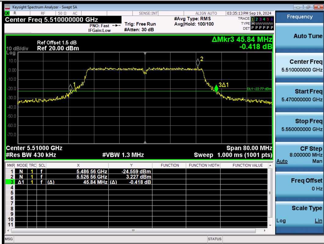
11AC40SISO-Ant1-5510
