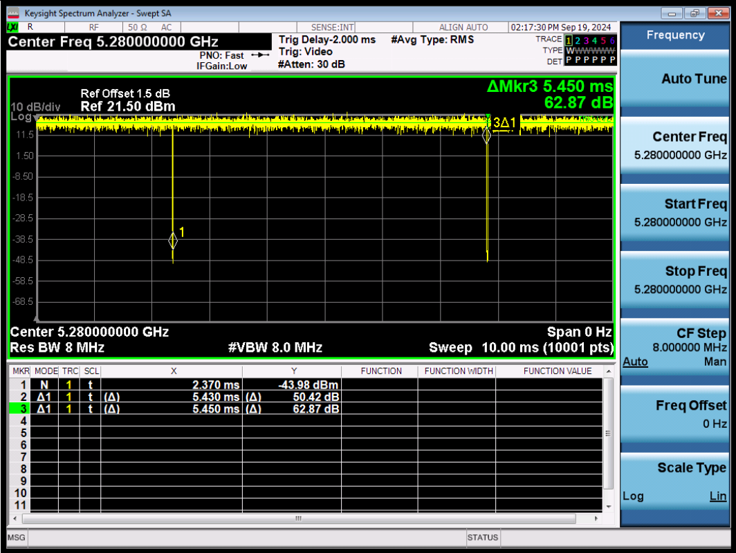
NTNV-11N20SISO-Ant1-5280
