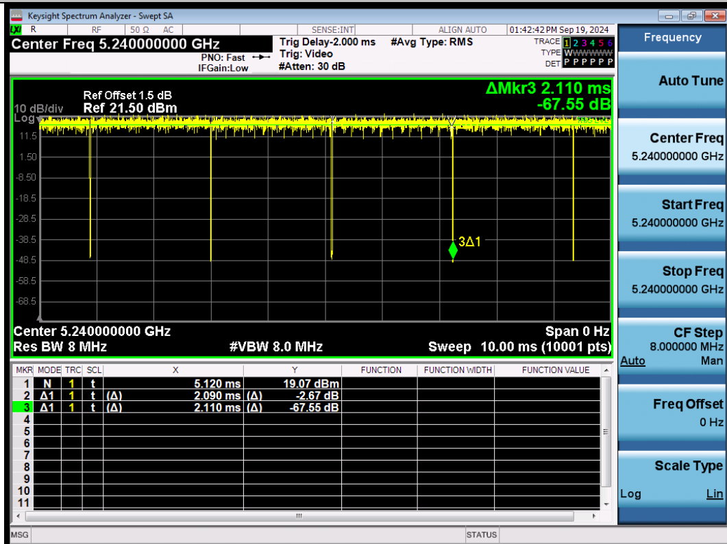
NTNV-11A-Ant1-5240
