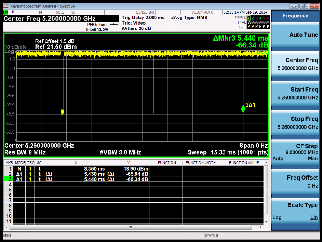
NTNV-11N20SISO-Ant1-5260
