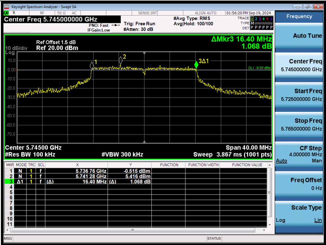
11A-Ant1-5745-PASS
