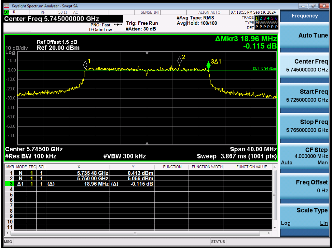
11BE20SISO-Ant1-5745-PASS
