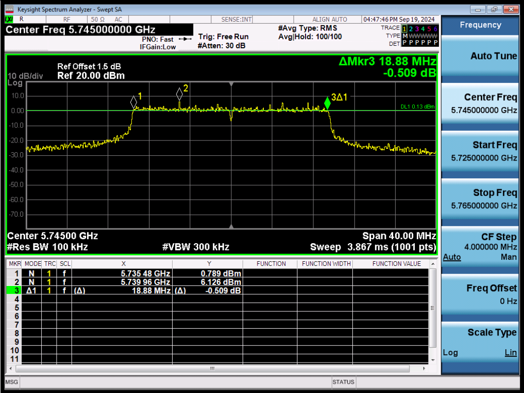
11AX20SISO-Ant1-5745-PASS
