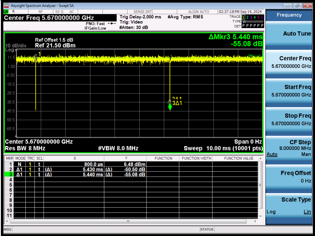
NTNV-11N40SISO-Ant1-5670
