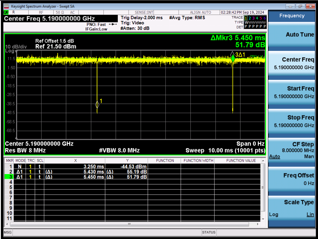
NTNV-11N40SISO-Ant1-5190
