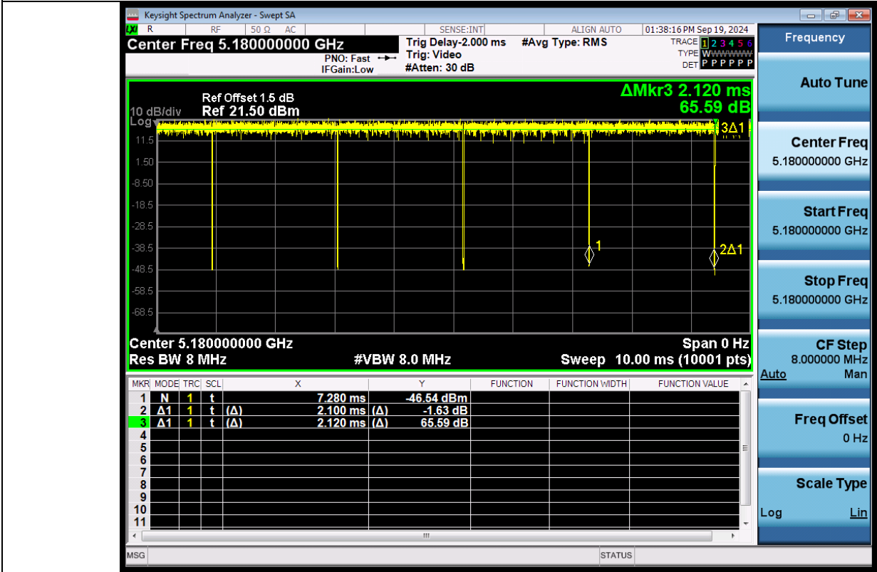
NTNV-11A-Ant1-5180
