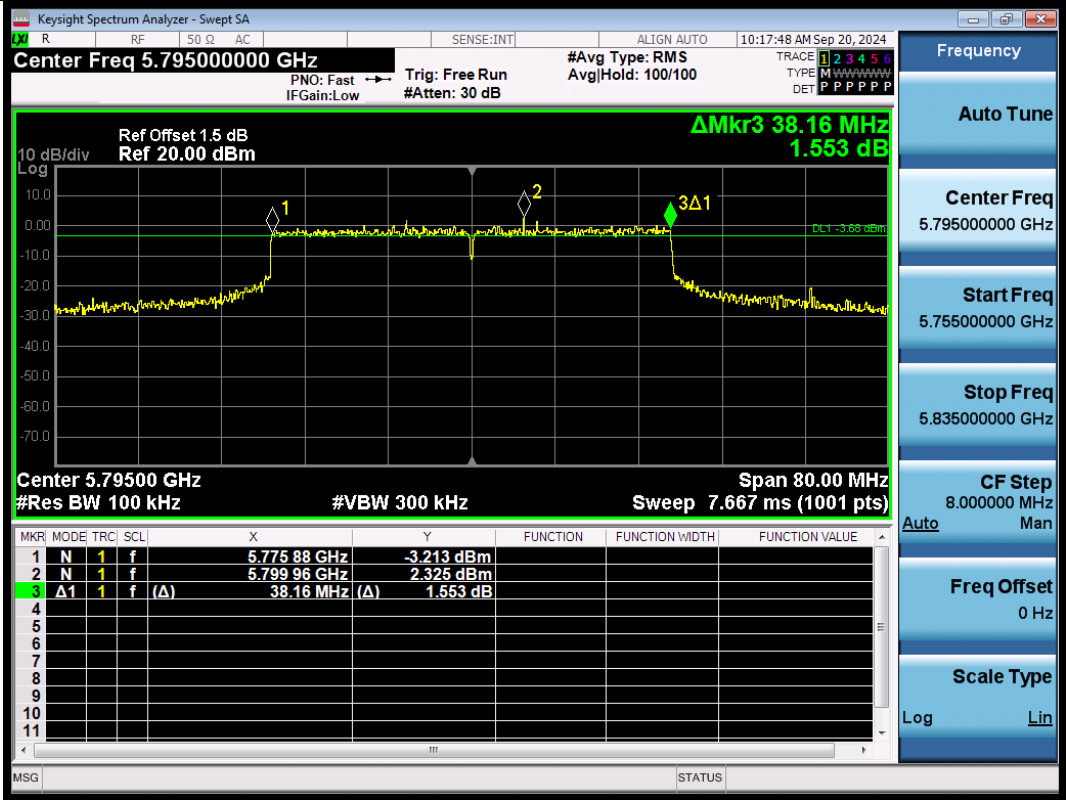
11BE40SISO-Ant1-5795-PASS
