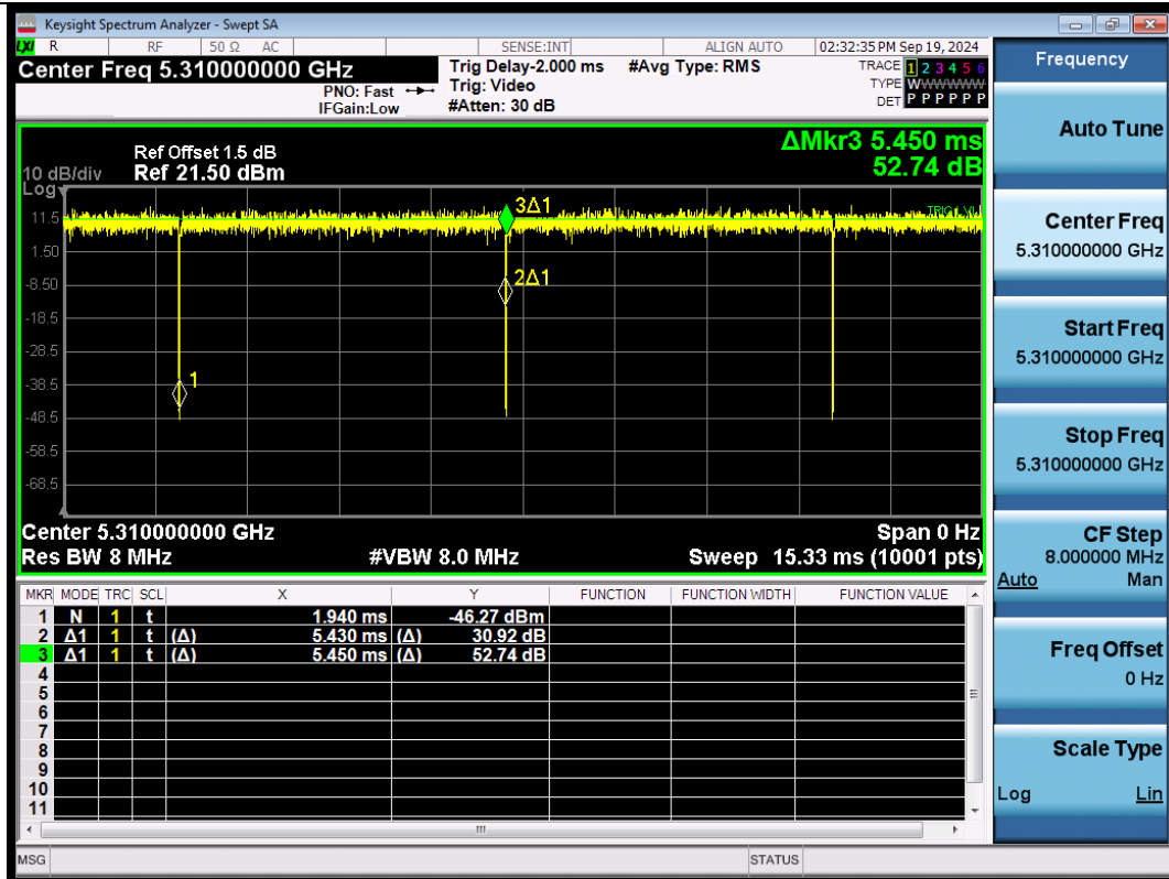
NTNV-11N40SISO-Ant1-5310
