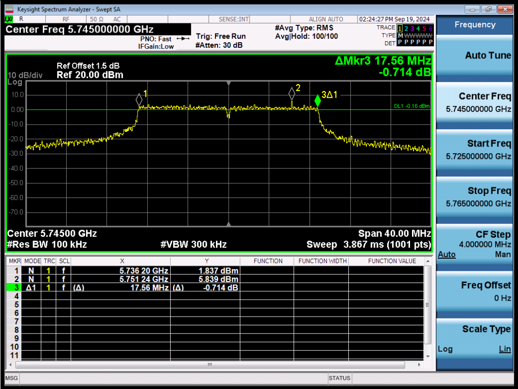
11N20SISO-Ant1-5745-PASS
