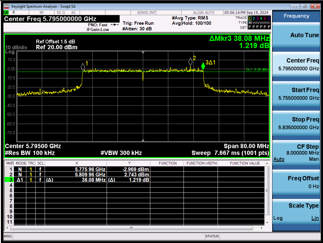
11AX40SISO-Ant1-5795-PASS
