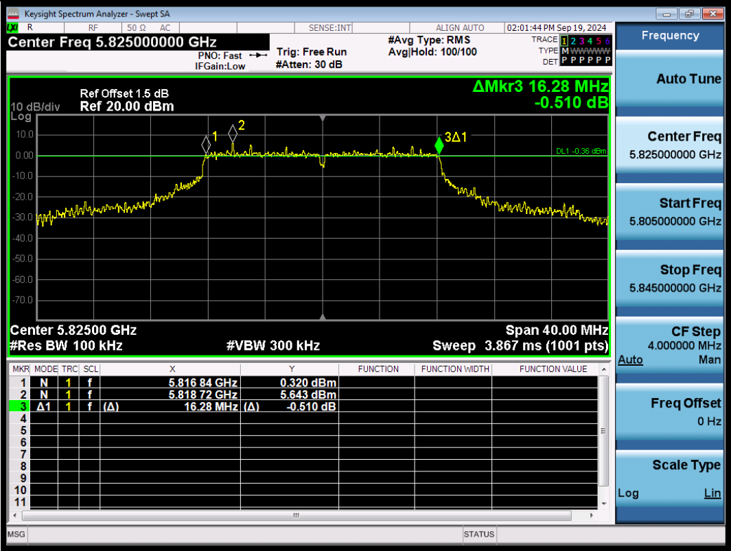
11A-Ant1-5825-PASS
