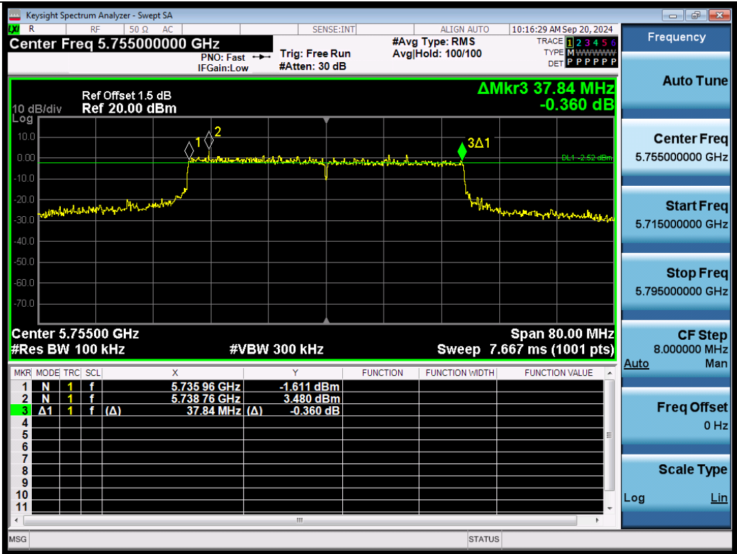
11BE40SISO-Ant1-5755-PASS
