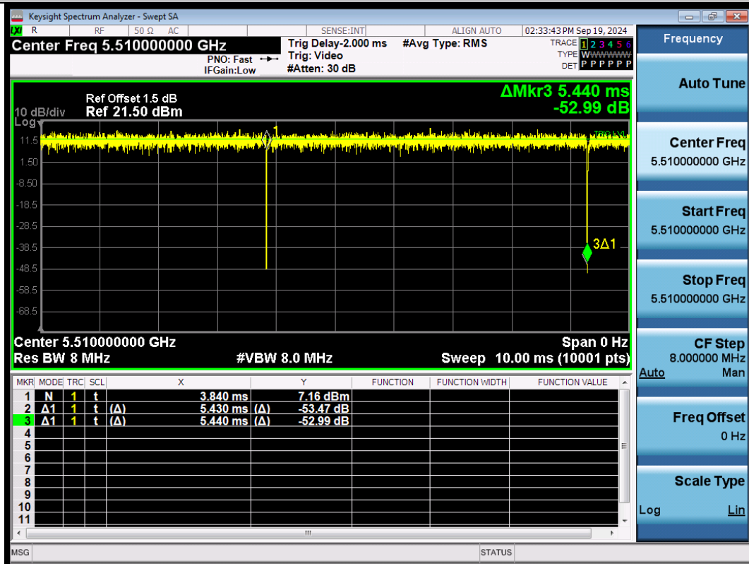
NTNV-11N40SISO-Ant1-5510
