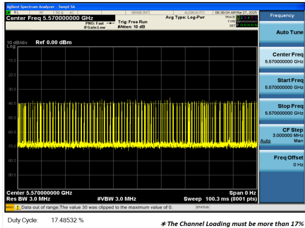
EHT160_5570MHz_Duty Cycle
